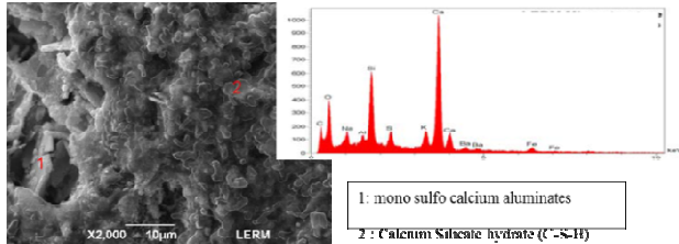
Fig. 11: Microstructure details
