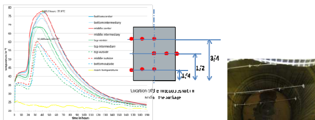
Fig. 5: Diagram of temperature evolution on and within a 380 L package (scale 1) during hardening
