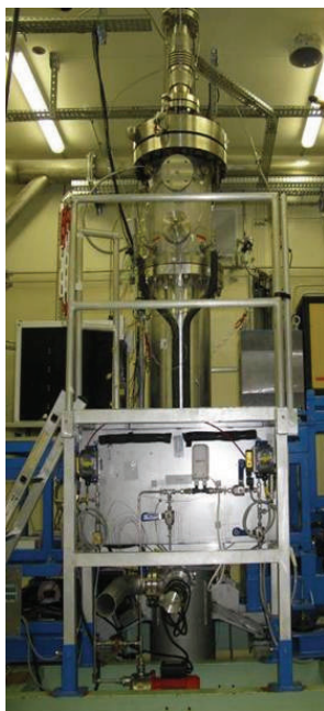
Figure 3. KROTOS facility.
