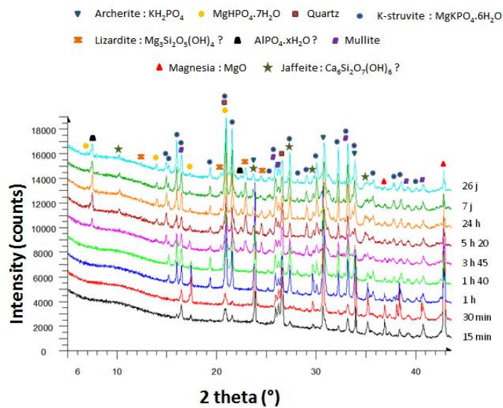
Figure 2: X-ray diffraction patterns of MPC paste aged from 15 min to 26 d ( \text{MgO} + \text{KH}_2\text{PO}_4 + \text{fly ash} , w/c = 0.56 )
