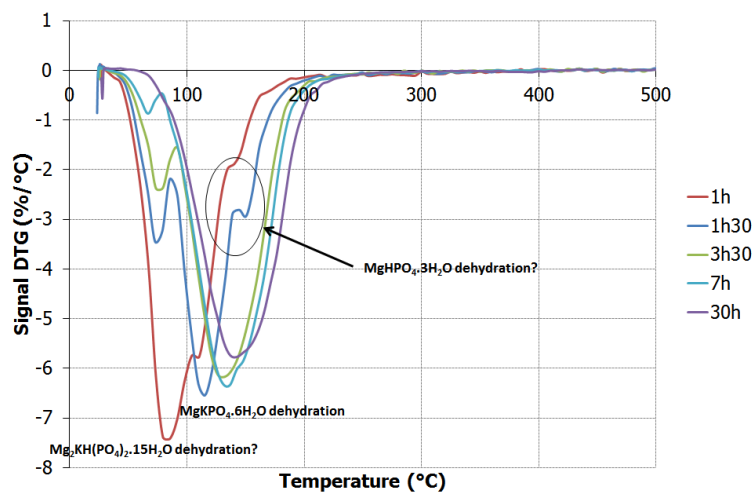
Figure 6: Thermograms of MPC suspension from 1 h to 30 h ( MgO + KH_2PO_4 + H_2O , w/c = 10 )
