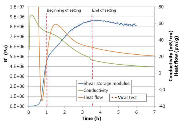
Figure 1 : Evolution of the electrical conductivity, heat flow and shear storage modulus of a MPC paste during hydration (MgO + \text{KH}_2\text{PO}_4 + fly ash, w/c = 0.56).
