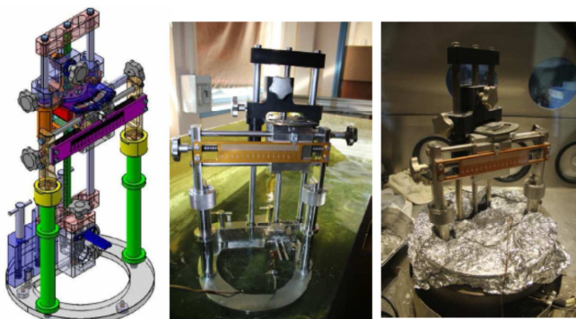
Fig 8. of TUCSS testing device (DEFO): CAD representation, water and sodium tests
