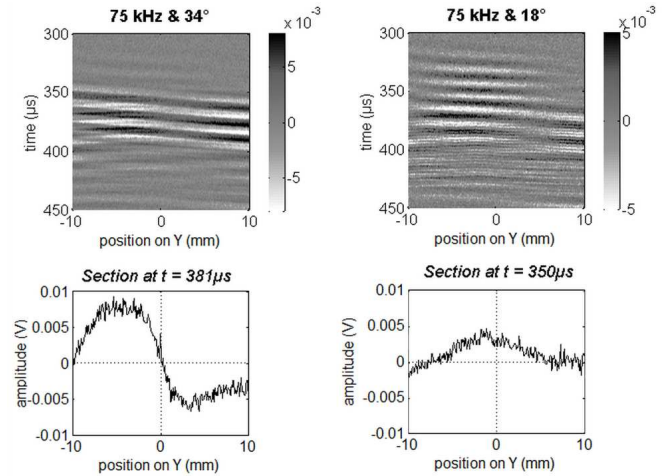
Fig. 21. Pressure amplitudes measured along the edge of the second plate. Left: antisymmetric mode. Right: symmetric mode.
