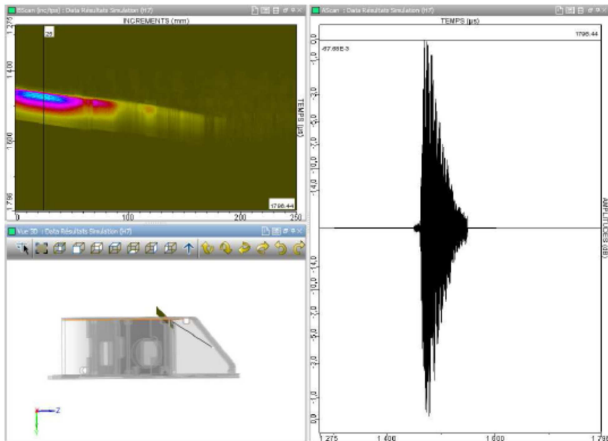
Fig. 17. CIVA code simulation of strongback inspection: example of NDE results.
