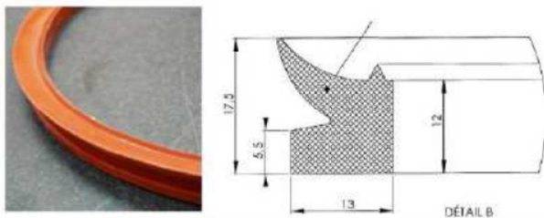
Fig. 32. Profile of silicone sealing joint.
