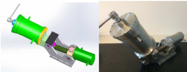
Fig. 35. Specific tight robot mockup with 2 degrees of freedom.
