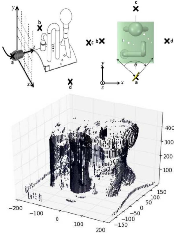
Fig. 13. XY raster and Z-theta approaches for CIVA code calculation of 3D mockup. Z-theta CIVA results.
