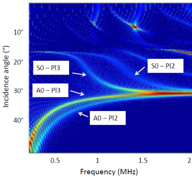
Fig. 19. Modulus of the acoustic transmission coefficients through a set of two plates immersed in water, along frequency and incidence.
