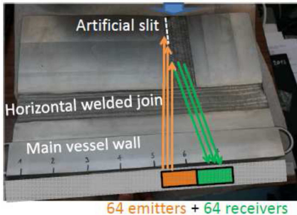
Fig. 26. Under water test configuration for vertical welded joint inspection with one 128 element sensor (plane wave case).
