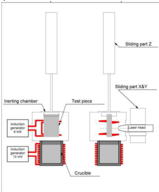
Fig. 29. BALTHAZAR laser test facility.
