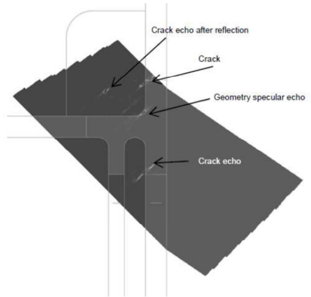
Fig. 24. NDE simulation of T45 inspection of strongback supporting skirt with two cracks, from behind the main vessel.
