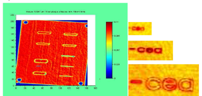
Fig. 12. Acoustic imaging (signal amplitude of echoes) of a plate with engraved slits and letters (under water test at room temperature).
