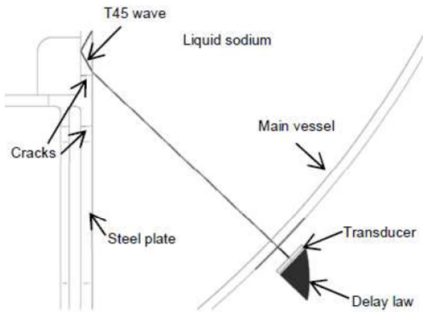
Fig. 23. Configuration of T45 inspection of strongback supporting skirt with two cracks, from behind the main vessel.
