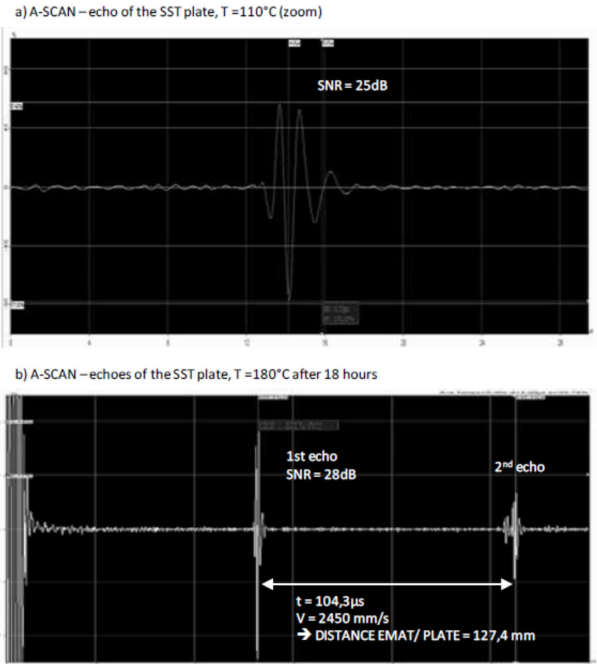
Fig. 2. A-SCAN of the EMAT echoes (in sodium at 110°C and 180°C).
