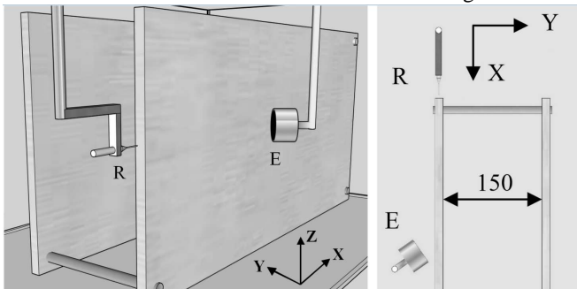
Fig. 20. Experimental setup (left: 3D, right: 2D top view).
