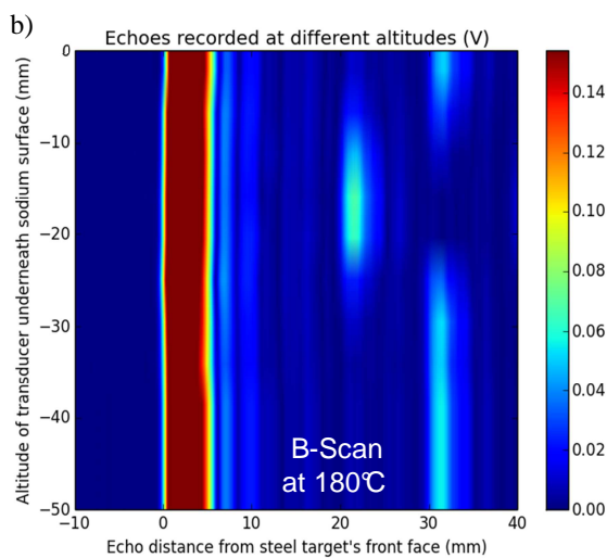
Fig 7. B-scan of the interior a 30mm thick stainless steel target comprising a 20x10mm notch on its backside – a) sketch of the experiment – b) B-scan
