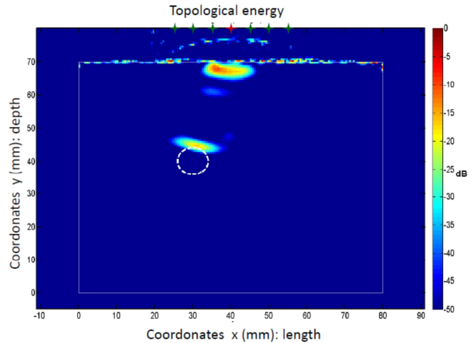
Fig. 10. Calculated topological energy for the case of a stainless steel block with an air cavity (adjoint field method).
