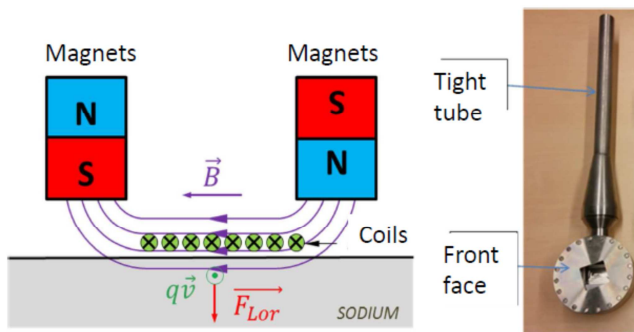
Fig. 1. Principle and photo of in sodium 8-phased array EMAT probe.
