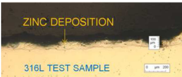
Fig. 30. Metallographic cross-section – zinc deposition on 316L steel.
