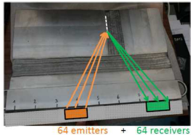
Fig. 28. Under water test configuration for vertical welded joint inspection with two 64 element sensors (focused wave case).
