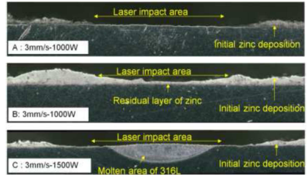
Fig. 31. Metallographic cross-sections - zinc evaporation.
