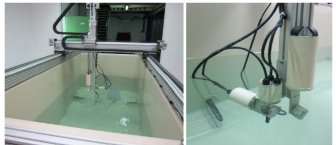
Fig. 11. VISIO water facility (2 m long, 1 m large, 1 m high) devoted to ultrasonic visualization study.
