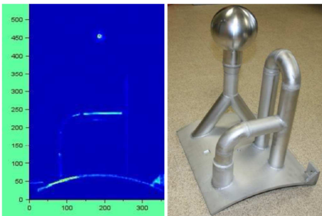
Fig. 14. In water 3D mockup ultrasonic imaging with XY raster sensor displacement in a vertical plan (echoes amplitude).
