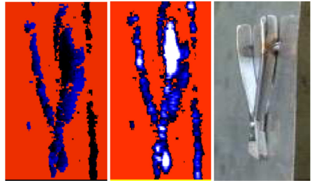
Fig. 15. In sodium acoustic imaging at 200°C: first plier raw reconstruction. Left: time of flight. Right: amplitude.
