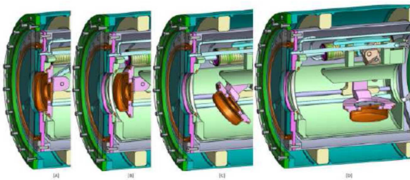
Fig. 33 Kinematic of the bell shutter: [A] Shutter closed, tight thanks to pressurized membrane [B] Depressurization of membrane and opening of the shutter [C] Removal of the shutter [D] Shutter completely removed.
