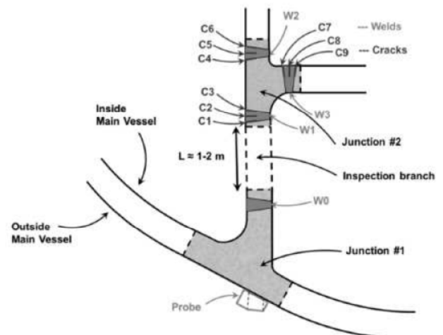
Fig. 22. Case study for guided wave inspection (top) and inspection configurations used (bottom).
