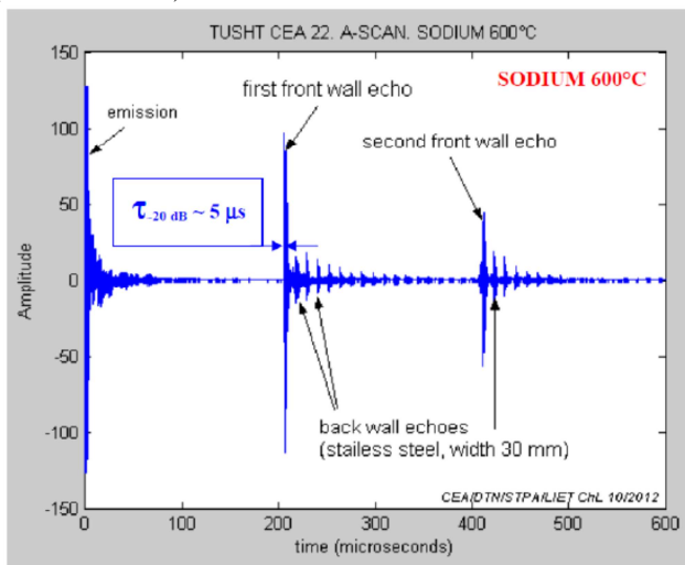
Fig. 5. TUSHT acoustic signal during sodium test at 600°C.
