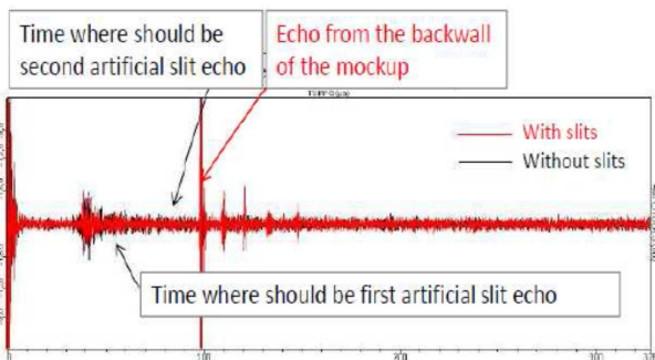
Fig. 27. NDE of core supporting skirt mockup (water test results at room temperature).
