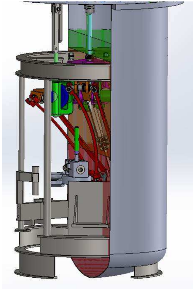
Fig. 18. Specific positioning device for US sensors, and strongback mockup for late 2015 sodium close-range NDE tests.
