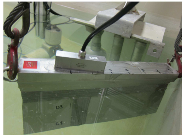
Fig. 25. Core supporting skirt mock 'up, during water tests.
