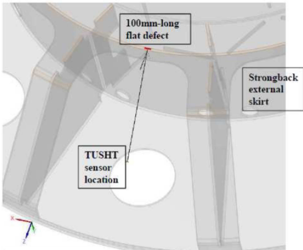
Fig. 16. CIVA code simulation of strongback inspection: example of NDE conditions.
