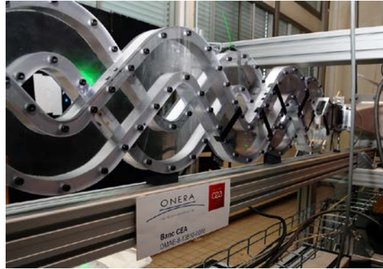
Figure 2 – LDV facility
