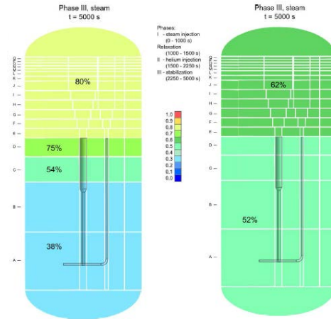
Fig.2. Planning calculations with KUPOL: steam distribution in the SPOT facility at the end of Phase III using the conditions of the original scenario (left) and the “modified scenario” (right).
