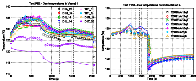
Fig.14. Post-test calculation of gas temperatures in test PE2 (left) and T116 (right) with GOTHIC (Symbols: data; Lines: simulation results).
