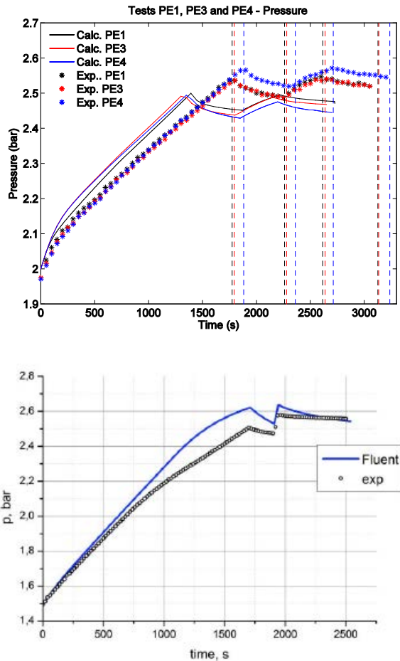
Fig.6. Pre-test calculations of pressurisation: (top) calculations with GOTHIC for tests in PANDA; (bottom) calculation with FLUENT for test MERCO-0 in MISTRA.
