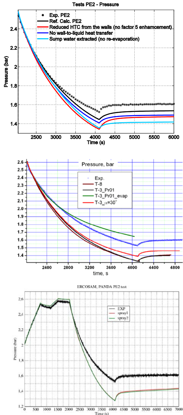
Fig.16. Post-test calculations of depressurization caused by spray in test PE2 with: (top) GOTHIC; (middle) FLUENT and various model choices; (bottom) with the LP code ASTEC (assuming two droplet trajectories).
