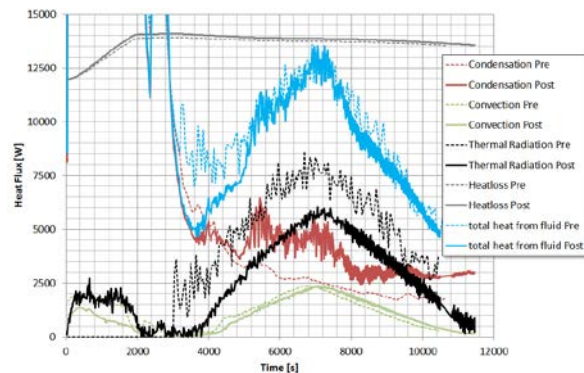
Fig.19. Post-test calculations of test PE4 with CFX: contributions to total heat transfer to the vessel walls by the various heat exchange modes.
