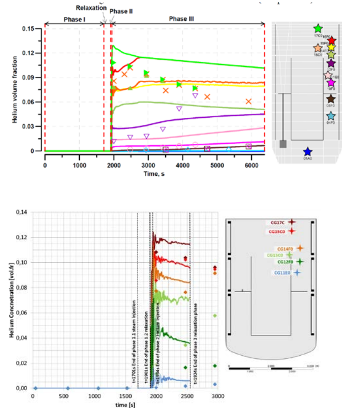
Fig.8. Pre-test calculations of helium concentrations at various locations in test MERC0-0: (top) calculations with LP code KUPOL; (bottom) calculations with the CFD code CFX. Symbols: data; Lines: simulation results.
