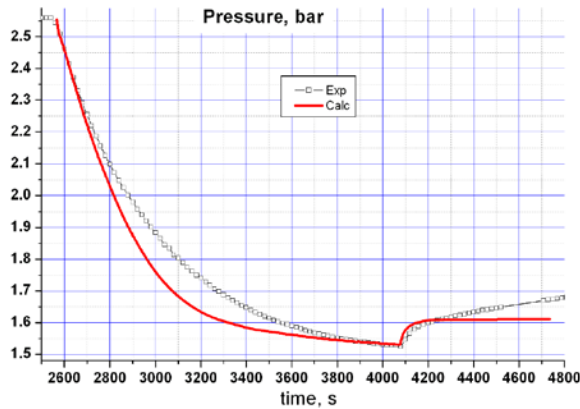
Fig.17. Post-test calculations of depressurization caused by spray: Test MERCO-1 simulated with FLUENT.
