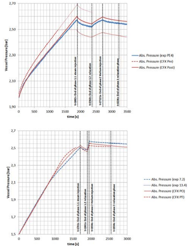
Fig.11. Pressure time-histories calculated in pre-test and post-test calculations by CFX for: (top) PANDA test PE4 and (bottom) MISTRA tests MERCO-0.
