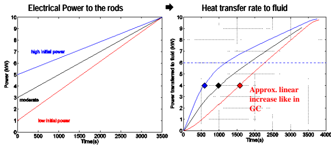
Fig.3. Planning calculations with GOTHIC: Power transferred to the fluid for various ramp shapes of electrical power supply for the test with heater in PANDA.
