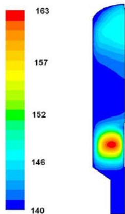
Fig.15. Post-test calculation of gas temperatures ( ^{\circ}\text{C} ) in test T116 with FLUENT.
