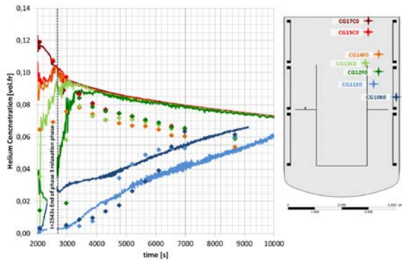
Fig.20. Post-test calculations of helium mixing caused by a heater: Test MERCO-3 simulated with CFX (Symbols: data; Lines: simulation results).
