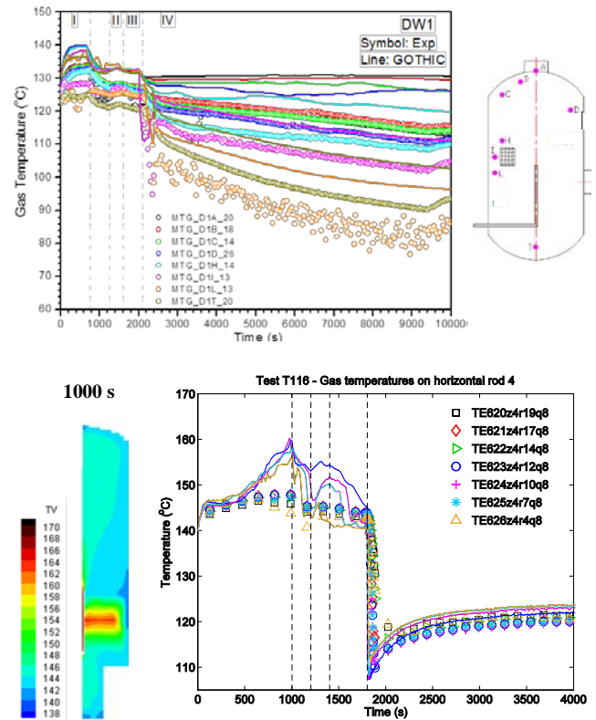
Fig.9. Pre-test calculations of gas temperatures with the GOTHIC code: (top) Vessel 1 of PANDA for test PE5; (bottom) Rod 4 ( z=1.47 m) in TOSQAN for Test T116. Symbols: data; Lines: simulation results.
