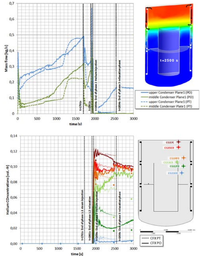
Fig.13. Post-test calculation of test MERCO-0 with CFX: (top) helium concentration distribution and circulation behind the condensers; (bottom) helium concentrations at various locations. Symbols: data; Lines: simulation results.
