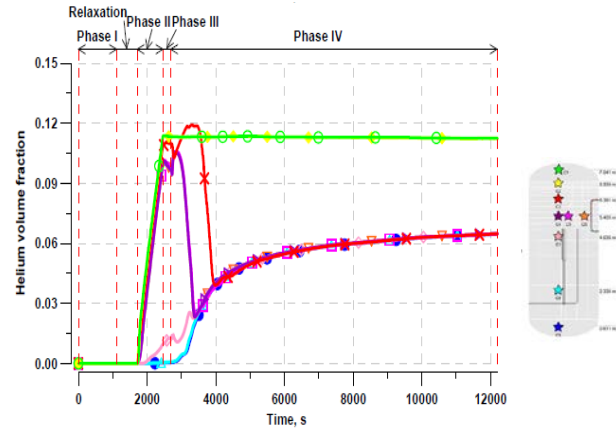
Fig.5. Planning calculations with KUPOL: helium concentrations at various elevations for test S1 in SPOT.
