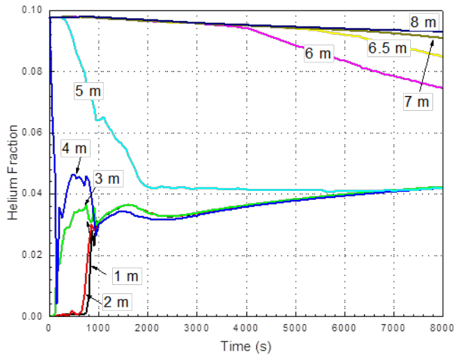
Fig.4. Planning calculations with GOTHIC for tests with a cooler in PANDA [9]: helium concentrations at various elevations for the case with cooler at 4 m.
