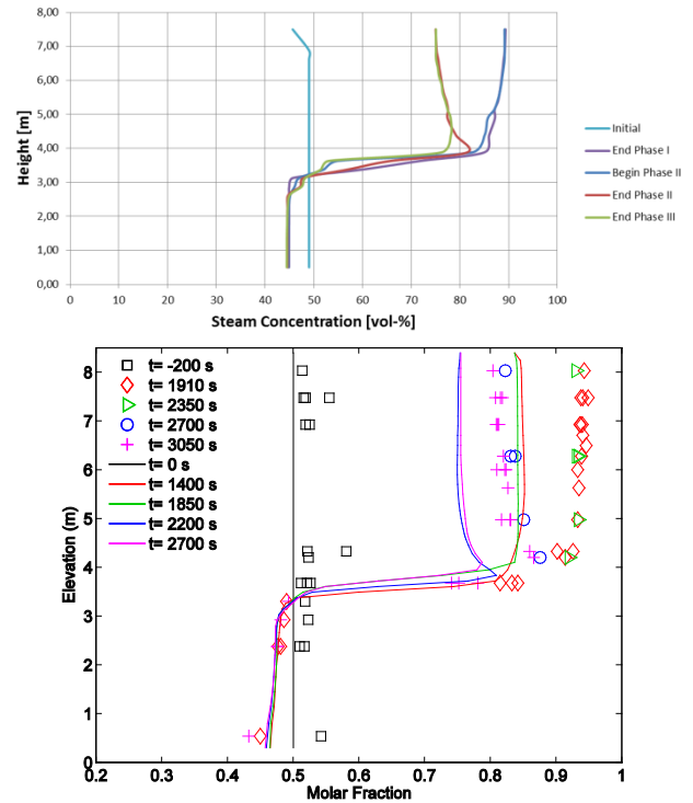
Fig.7. Pre-test calculations of steam vertical distribution in Vessel 1 for tests in PANDA with condensation: (top) calculations with the LP code COCOSYS; (bottom) calculations with GOTHIC (Symbols: data; Lines: simulation results)
