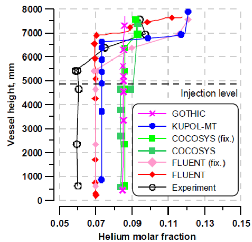
Fig.23. Post-test calculations of vertical helium distribution in test S1 in SPOT with various codes.
