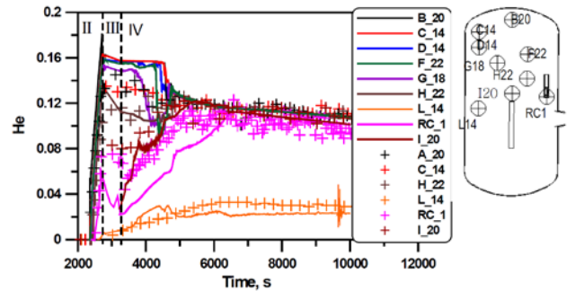
Fig.18. Post-test calculations of helium mixing caused by a heater: Test PE4 simulated with FLUENT (Symbols: data; Lines: simulation results).
