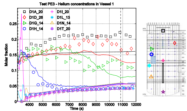
Fig.22. Post-test calculations of helium mixing caused by a cooler: simulations with GOTHIC for Test PE3 (Symbols: data; Lines: simulations results).
