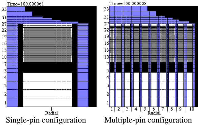
Figure 8: Radial meshing refinement (fuel bundle)
