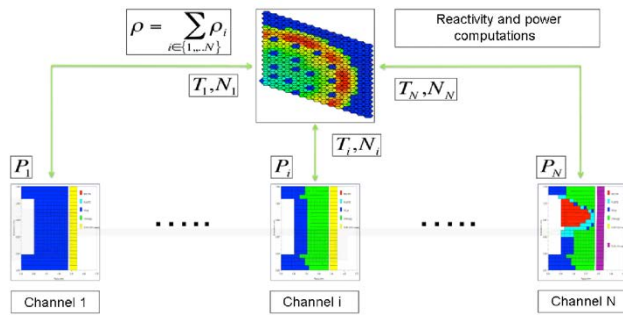
Figure 3 : Data exchange topology for the SIMMER-III/SNATCH coupled code
