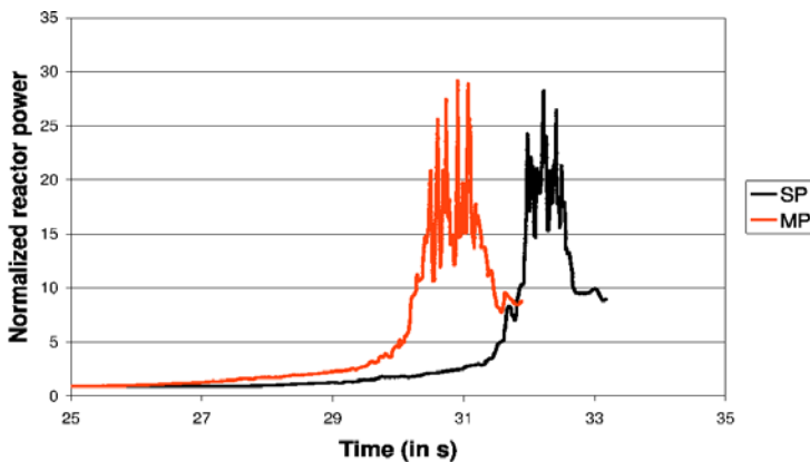
Figure 9: Power versus time for the two discretizations (SP and MP)
