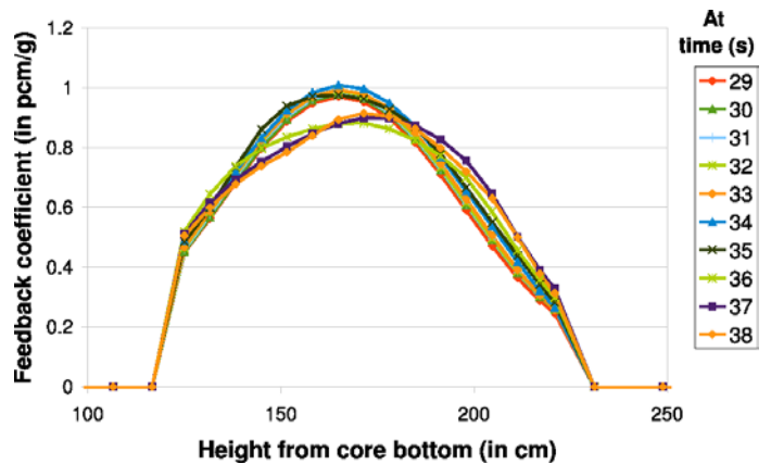
Figure 12: Fuel feedback reactivity coefficient as a function of time (high-power channel)
