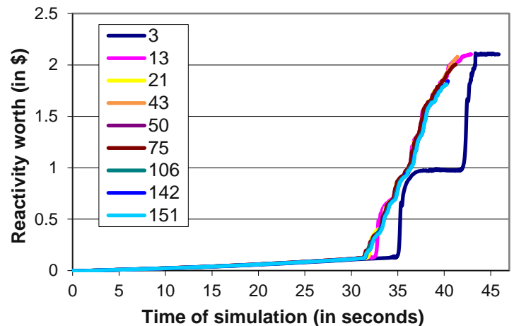
Figure 6: Coolant feedback reactivity versus time
