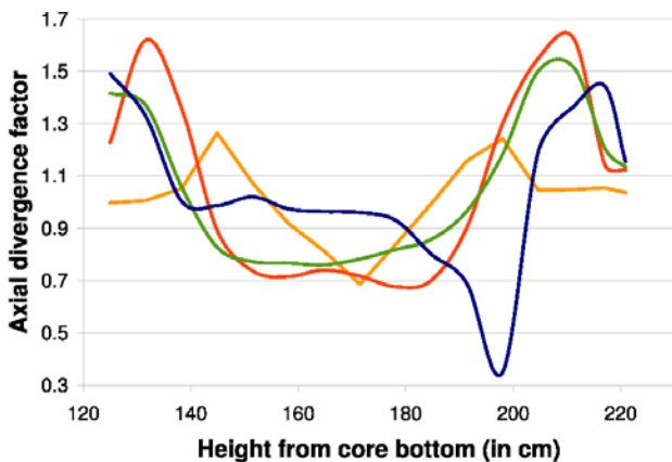
Figure 10: Variation of the axial power profile for a high-power channel - first part
