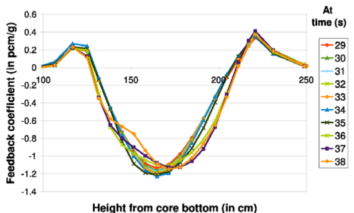
Figure 13: Coolant feedback reactivity coefficient as a function of time (high-power channel)
