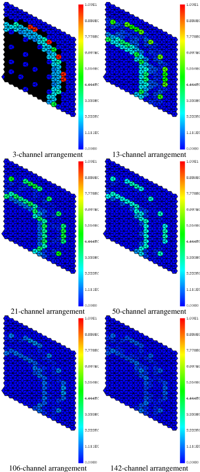
Figure 7: Absolute deviations of the averaged fuel-melt fraction with respect to the reference calculation
