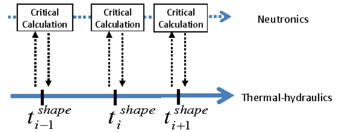
Figure 4: Strategy for obtaining the nominal state of a reactor
