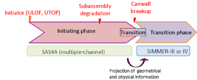
Figure 1: Standard computational route for severe accident
