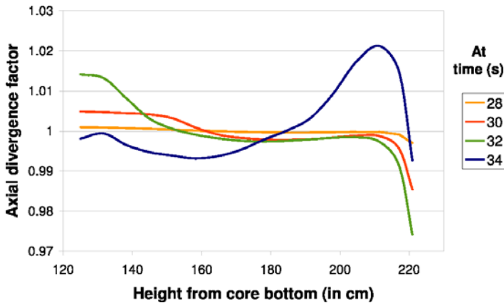
Figure 10: Variation of the axial power profile for a high-power channel - first part
