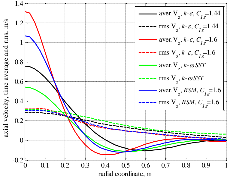
Figure 4. Radial distribution of the average and rms jet center line axial velocities at 110 seconds. Results for z=5.1m (see Figure 3).
