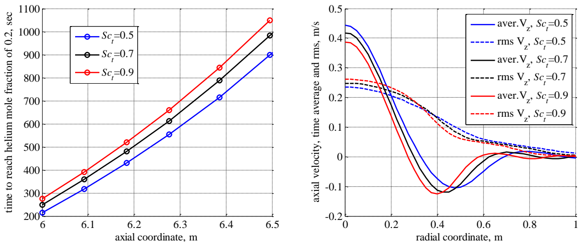
Figure 7. Sc_t impact for the modified k-\epsilon model. Left: time for helium concentration to drop to 0.2. Right: velocities at z=6.11m for 715 seconds into the transient.
