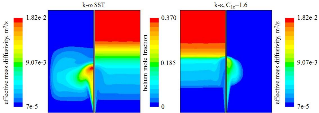
Figure 6. Effective mass diffusivity (outer contours) and helium mole fraction (inner contours) for 110 seconds. Results for k-\omega SST and k-\epsilon model with C_{1\epsilon}=1.6 .
