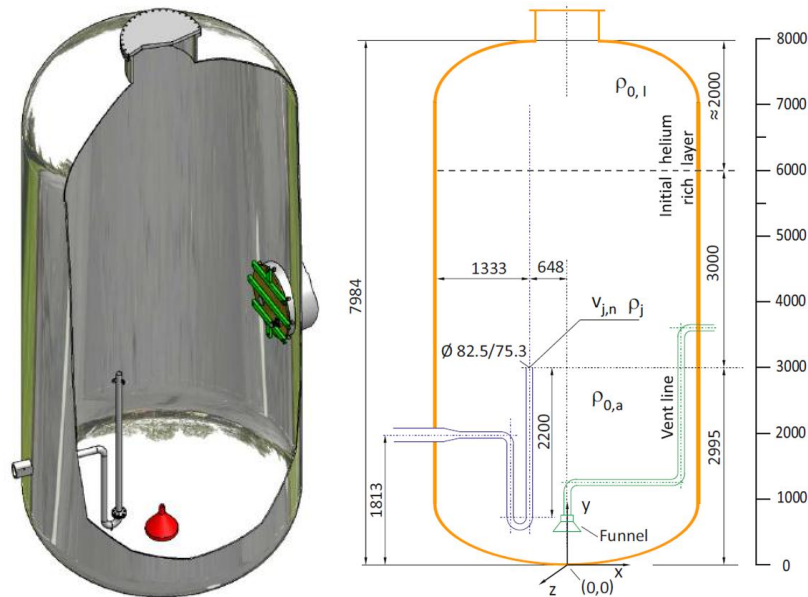
Figure 2. PANDA vessel IBE-3 set-up [1].
