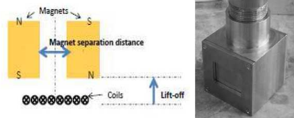
Fig. 2. Principle and photo of in sodium 8-phased array EMAT probe.
