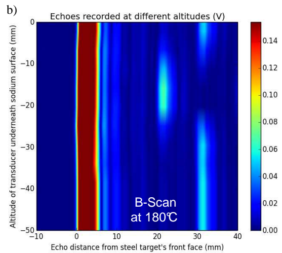
Fig 8. B-scan of the interior a 30mm thick stainless steel target comprising a 20x10mm notch on its backside – a) sketch of the experiment – b) B-scan
