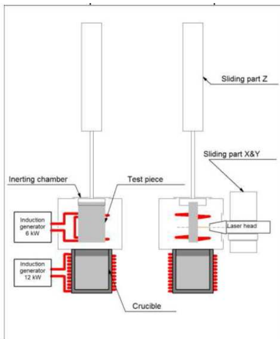
Fig. 30. BALHAZAR laser test facility.
