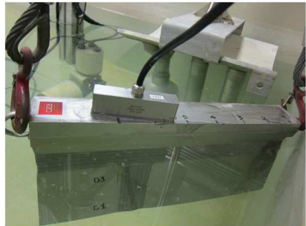
Fig. 19. Core supporting skirt mock 'up, during water tests.
