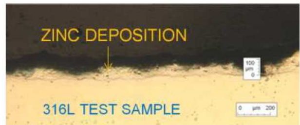
Fig. 31. Metallographic cross-section – zinc deposition on 316L steel.
