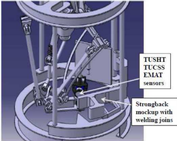
Fig. 12. Specific positioning device for US sensors, and strongback mockup for 2015 sodium close-range NDE tests.
