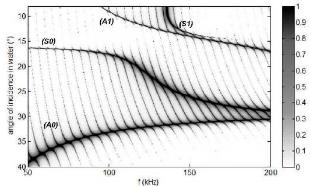
Fig. 13. Modulus of the transmission coefficients through a set of two plates, along frequency and incidence.
