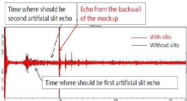
Fig. 21. NDE of core supporting skirt mockup (water test results at room temperature).
