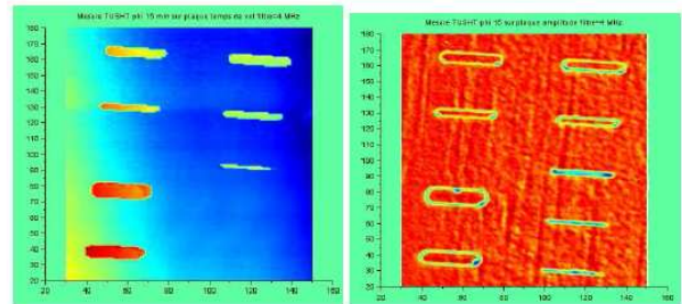
Fig. 26. Acoustic imaging of a plate with slits. Left: time of flight. Right: amplitude (under water test at room temperature).
