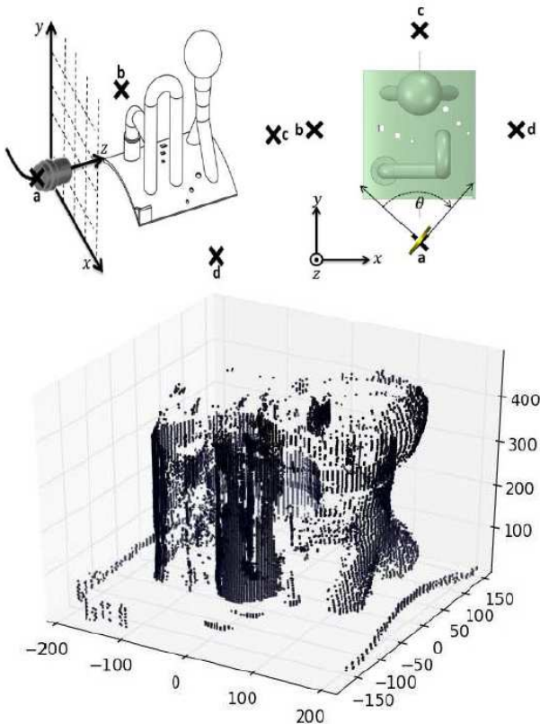
Fig. 27. XY raster and Z-theta approaches for CIVA code calculation of 3D mockup. Z-theta CIVA results.
