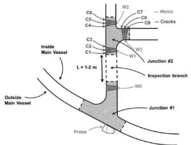
Fig. 16. Case study for guided wave inspection (top) and inspection configurations used (bottom).
