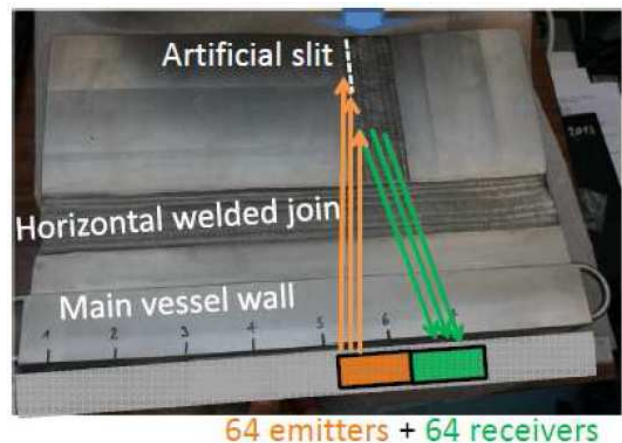
Fig. 20. Under water test configuration for vertical welded joint inspection with one 128 element sensor (plane wave case).
