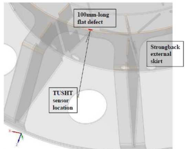
Fig. 10. CIVA code simulation of strongback inspection: example of NDE conditions.
