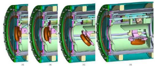
Fig. 34 Kinematic of the bell shutter: [A] Shutter closed, tight thanks to pressurized membrane [B] Depressurization of membrane and opening of the shutter [C] Removal of the shutter [D] Shutter completely removed.
