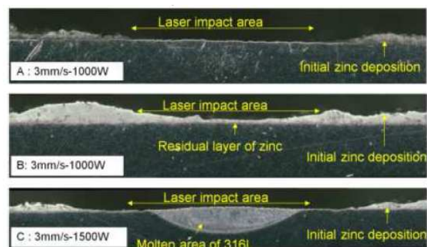
Fig. 32. Metallographic cross-sections - zinc evaporation.
