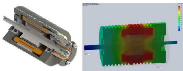
Fig. 35. Prototypic brushless motor working at 200°C.
