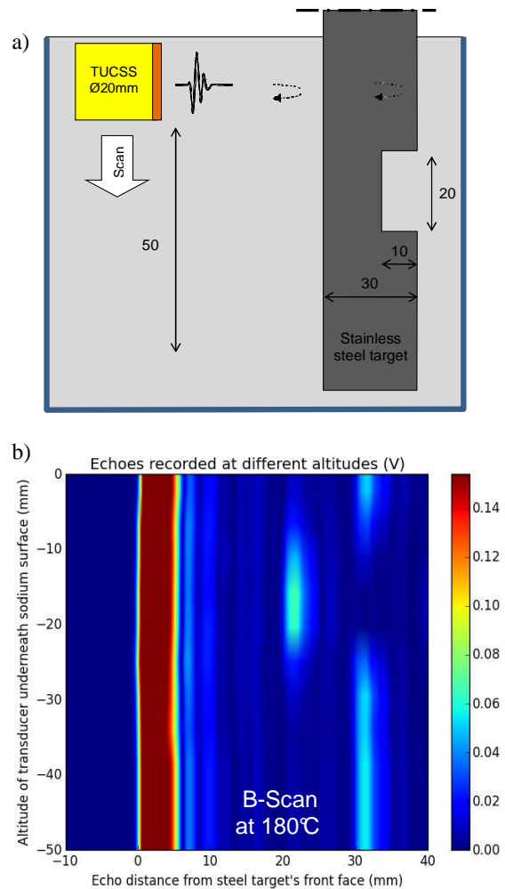
Fig 8. B-scan of the interior a 30mm thick stainless steel target comprising a 20x10mm notch on its backside – a) sketch of the experiment – b) B-scan
