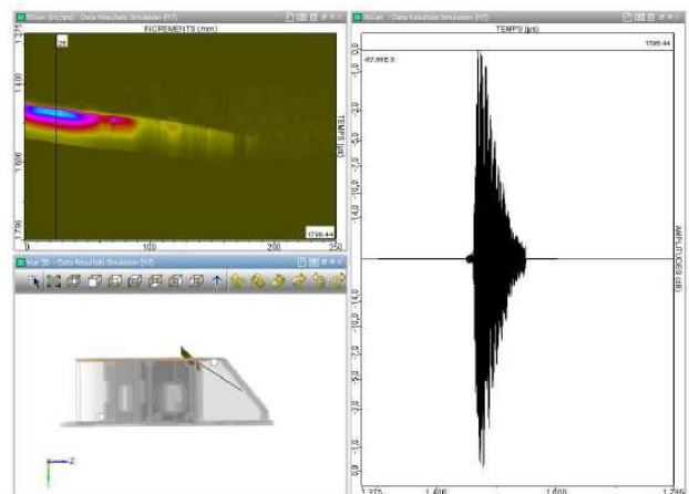
Fig. 11. CIVA code simulation of strongback inspection: example of NDE results.
