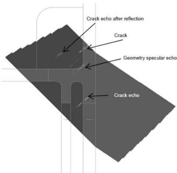
Fig. 18. NDE simulation of T45 inspection of strongback supporting skirt with two cracks, from behind the main vessel.
