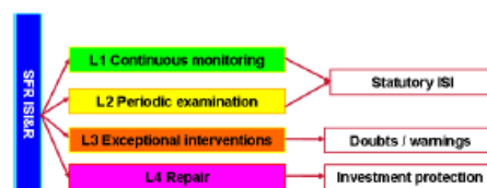
Fig. 1. French ISI&R organization for SFRs.
