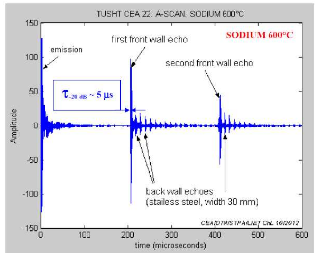
Fig. 6. TUSHT acoustic signal during sodium test at 600°C.
