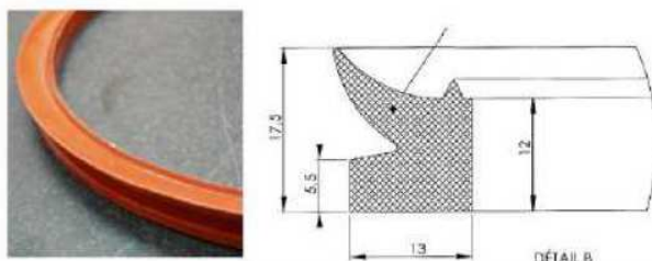
Fig. 33. Profile of silicone sealing joint.
