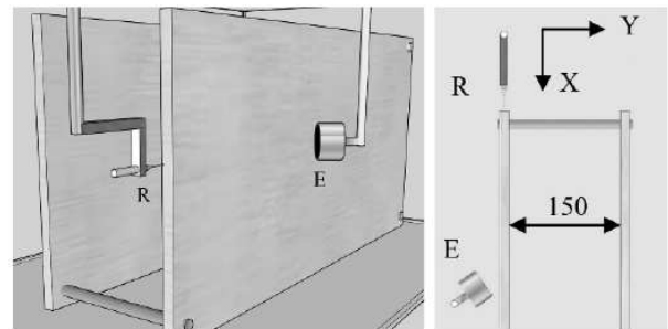
Fig. 14. Experimental setup (left: 3D, right: 2D top view).
