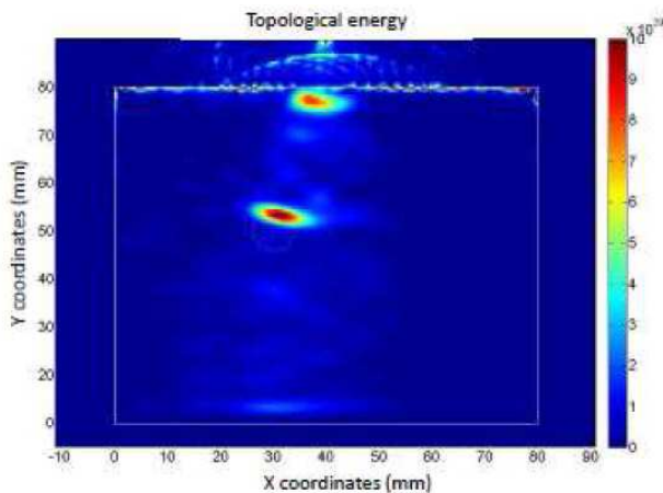
Fig. 24. Calculated topological energy for the case of a stainless steel block with an air cavity (adjoint field method).
