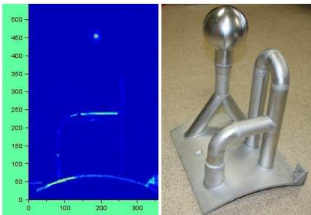
Fig. 28. In water 3D mockup ultrasonic imaging with sensor displacement in a vertical plan (echoes amplitude).
