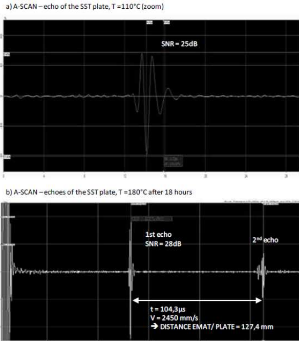
Fig. 3. A-SCAN of the EMAT echoes (in sodium at 110°C and 180°C).
