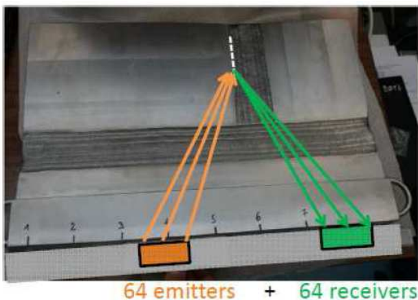
Fig. 22. Under water test configuration for vertical welded joint inspection with two 64 element sensors (focused wave case).
