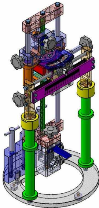
Fig 9. CAD representation of TUCSS testing device (DEFO)
