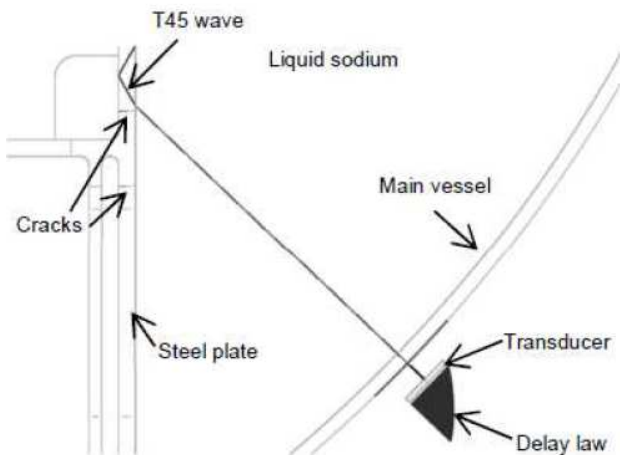
Fig. 17. Configuration of T45 inspection of strongback supporting skirt with two cracks, from behind the main vessel.
