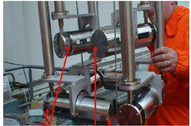
TUSHT TARGET Fig. 5. TUSHT and target setting for sodium test.
