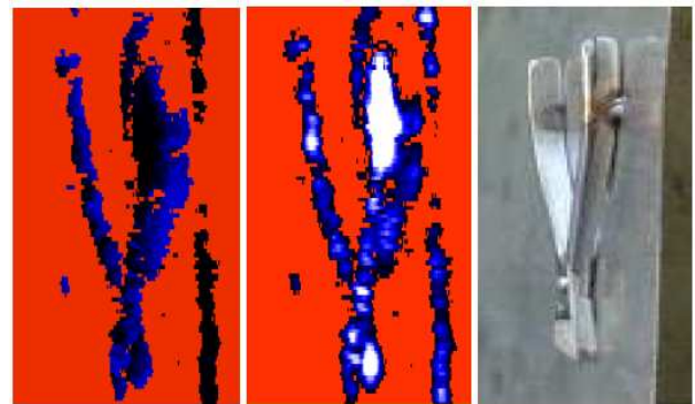
Fig. 29. In sodium acoustic imaging at 200°C: first plier raw reconstruction. Left: time of flight. Right: amplitude.
