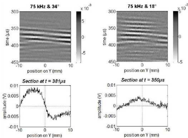
Fig. 15. Pressure amplitudes measured along the edge of the second plate. Left: antisymmetric mode. Right: symmetric mode.
