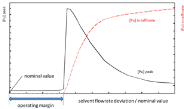
Figure 2. Plutonium peak concentration and plutonium leak in the raffinate in case of extraction solvent flowrate decrease
