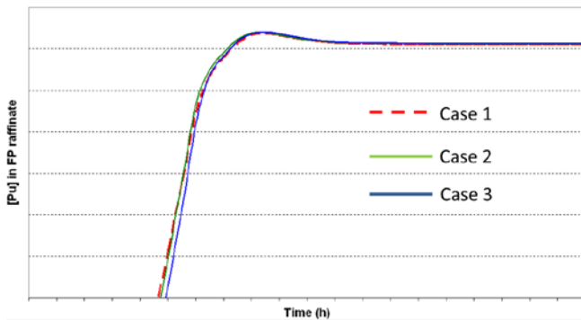
Figure 6- Dynamic simulation of "equivalent" malfunction
