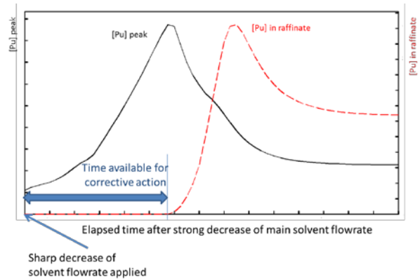
Figure 3- Plutonium leakage and build up in case of sharp decrease of extraction solvent flow rate
