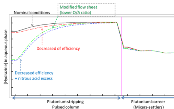
Figure 9- Hydrazine profiles simulation in plutonium stripping column
