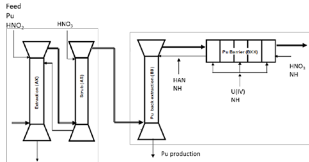
Figure 7- 2 nd plutonium purification flow sheet
