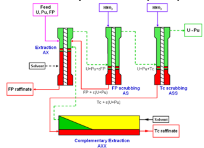
Figure 1. Extraction zone of the first purification cycle flow sheet
