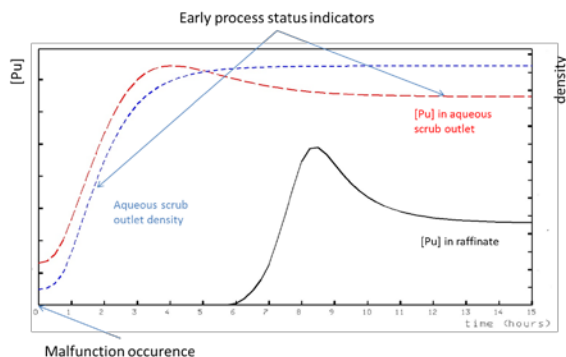
Figure 4- Process status indicators evolution in case of sharp decrease of extraction solvent flow rate
