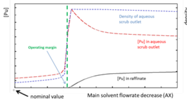
Figure 2. Identification of process status indicators
