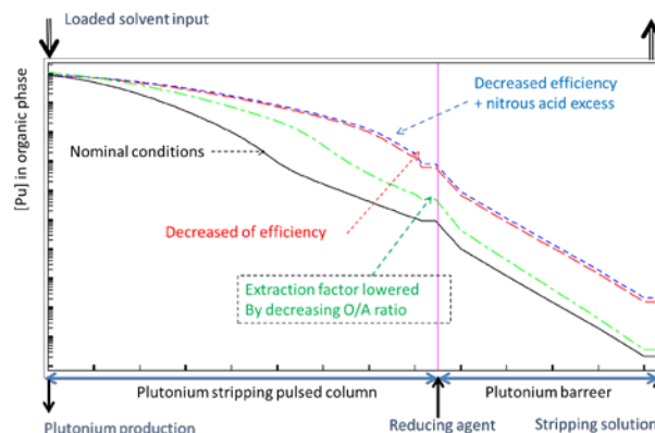
Figure 8- Organic [Pu] profile simulation in plutonium stripping column
