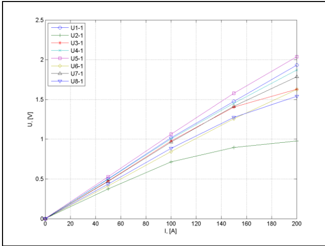
Fig. 21. 1 st coils signal : U = U(I) .
