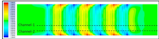
Fig. 7. Magnetic field ( B_x ) distribution: Q=45 l/s, I=200 A.
