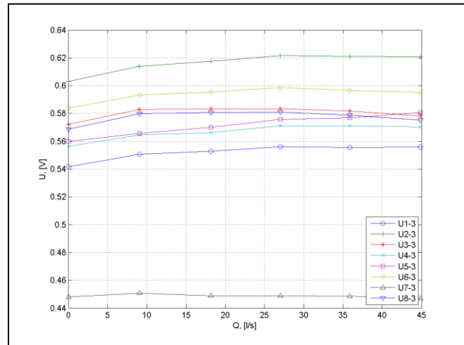
Fig. 26. 3 rd coils signal, I = 200A : U = U(Q) .
