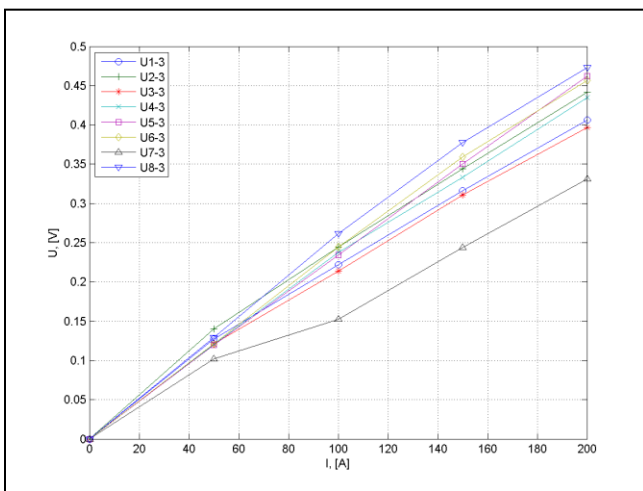
Fig. 23. 3 rd coils signal: U = U(I) .
