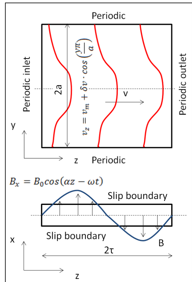
Fig. 2. Model of an infinite ALIP.
