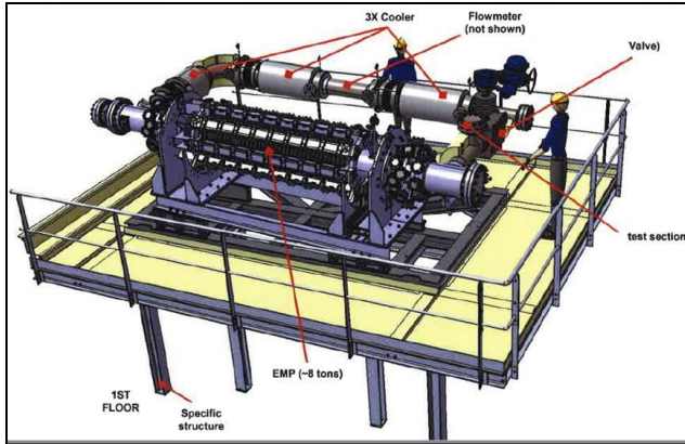
Fig. 1. A drawing of the PEMDYN facility.
