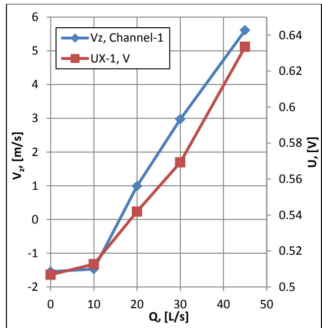
Fig. 12. Velocity of in the center of channel-1 and calculated voltage corresponding to magnetic field maximum.
