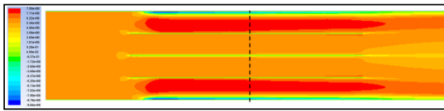
Fig. 9. Velocity z component distribution: Q=45 l/s, I=200 A
