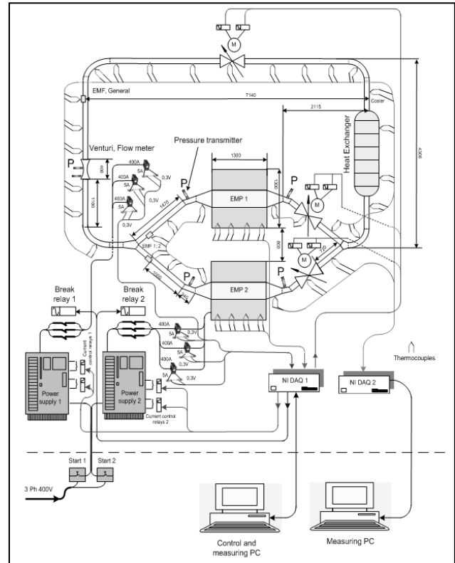
Fig. 14. The principal scheme of the measuring and control system of TESLA-EMP facility
