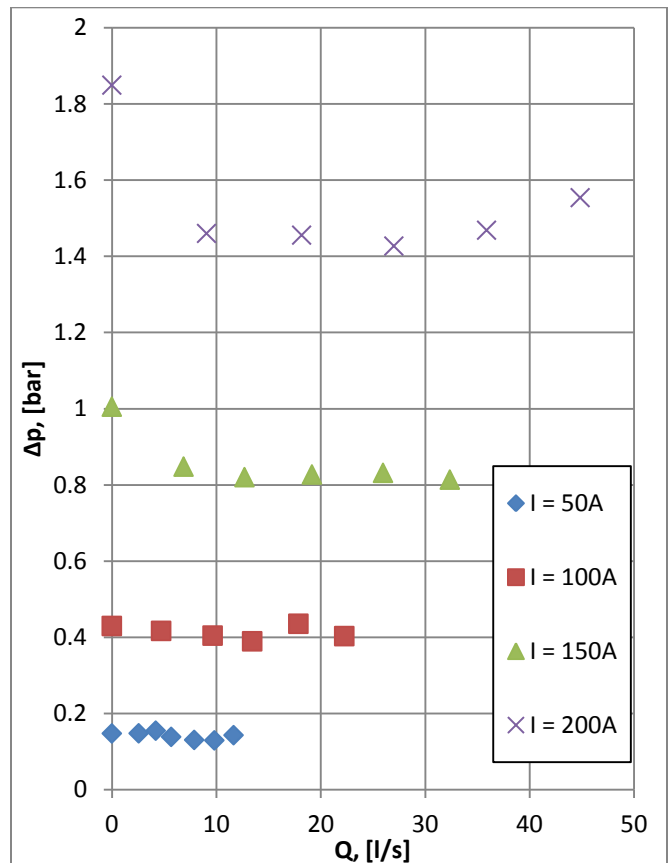
Fig. 17. Pressure – flowrate characteristics of EMIP with different line current.
