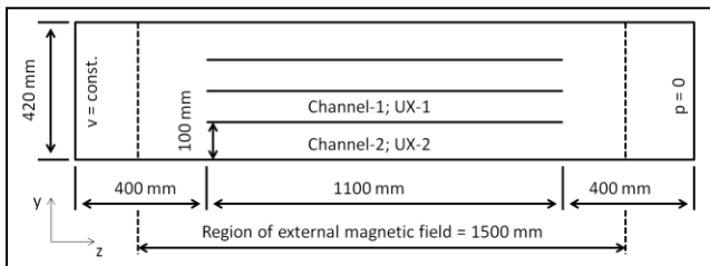
Fig. 5. Geometry of the EMIP model of TESLA-EMP.
