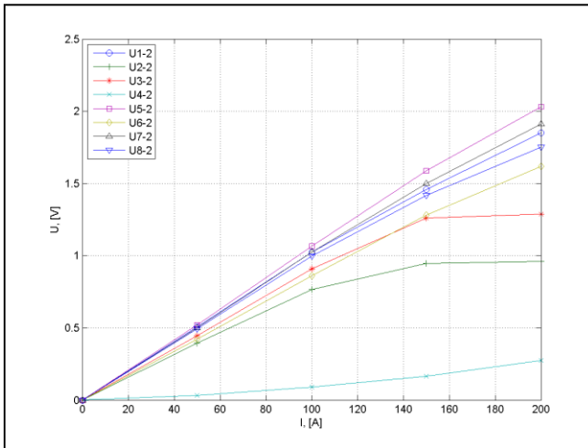
Fig. 22. 2 nd coils signal: U = U(I) .
