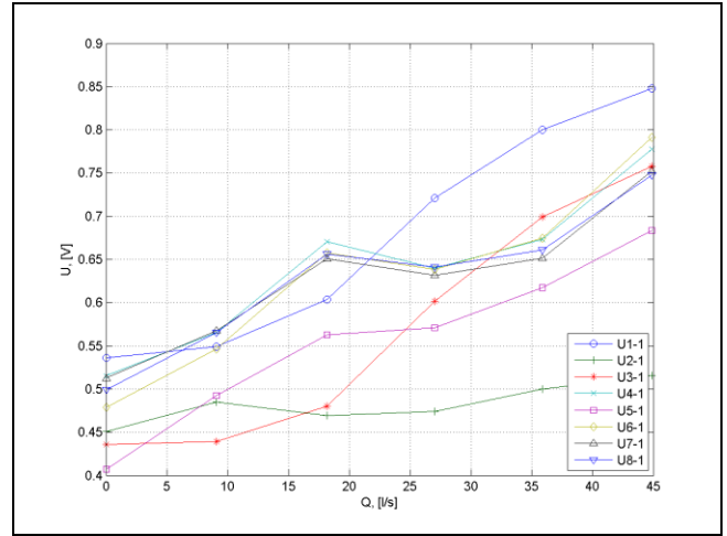
Fig. 24. 1 st coils signal, I = 200A : U = U(Q) .
