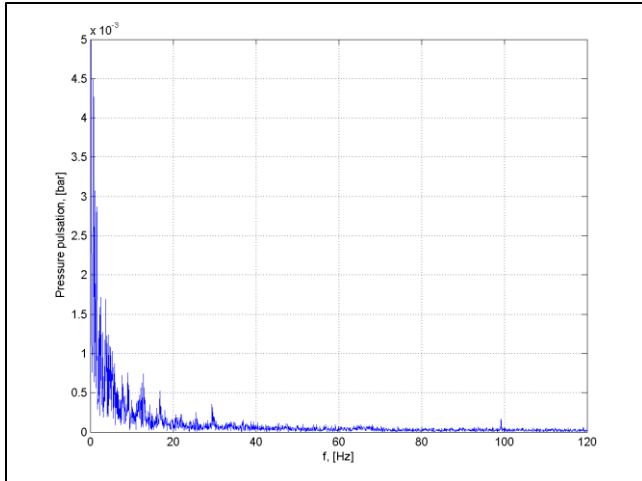
Fig. 18. \Delta p pulsation spectrum: I = 200A , Q = 0 L/s.
