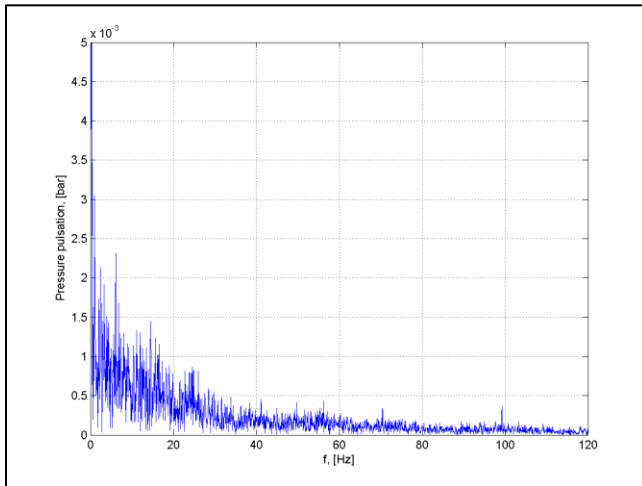
Fig.19. \Delta p pulsation spectrum: I = 200A , Q = 27 L/s.
