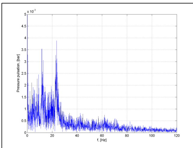
Fig. 20. \Delta p pulsation spectrum: I = 200A , Q = 45 L/s.
