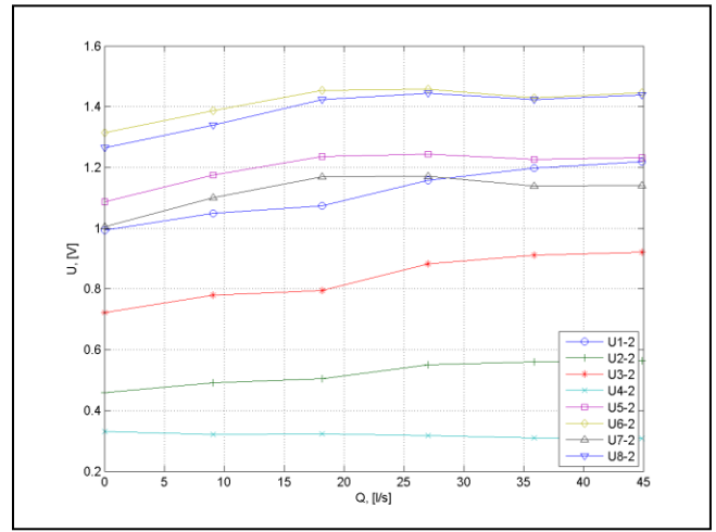
Fig. 25. 2 nd coils signal, I = 200A : U = U(Q) .
