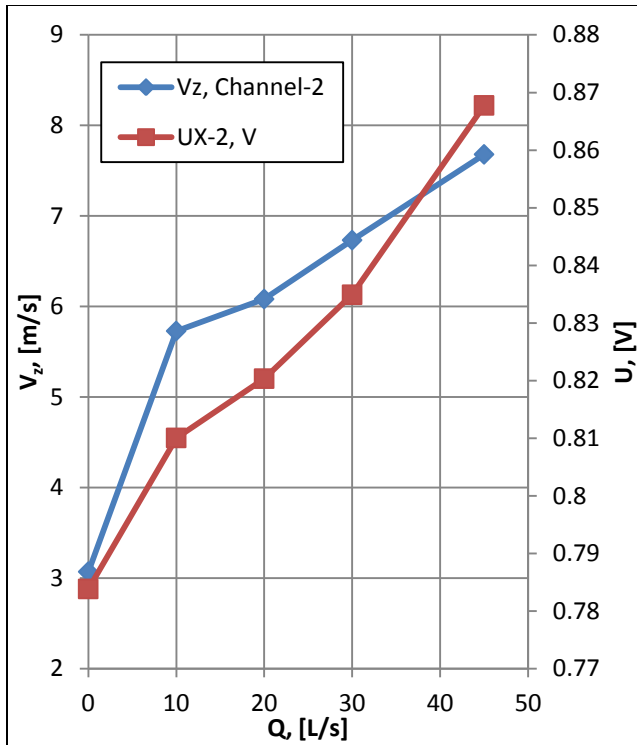
Fig. 13. Velocity of in the center of channel-2 and calculated voltage corresponding to magnetic field maximum.
