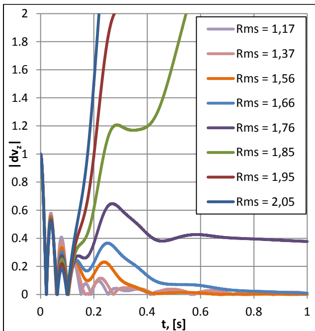
Fig. 3. Temporal development of v_z perturbation with Rm \approx 6.44 , N \approx 10 and different Rm_s .
