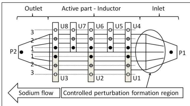
Fig. 16: Principal scheme of channel. Placement of magnetic field sensors (U1 – U8) and pressure measurements (P1 and P2).
