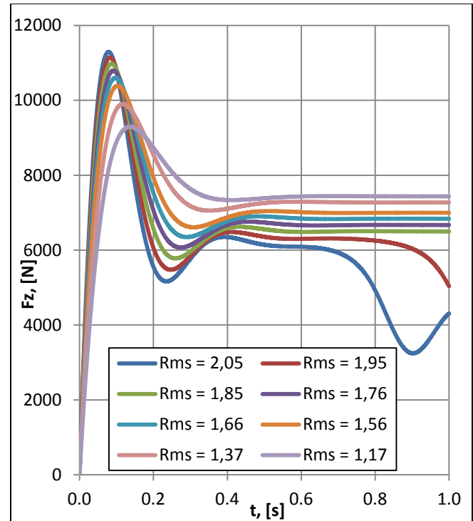
Fig. 4. Transient development of integral axial force F_z with different Rm_s .
