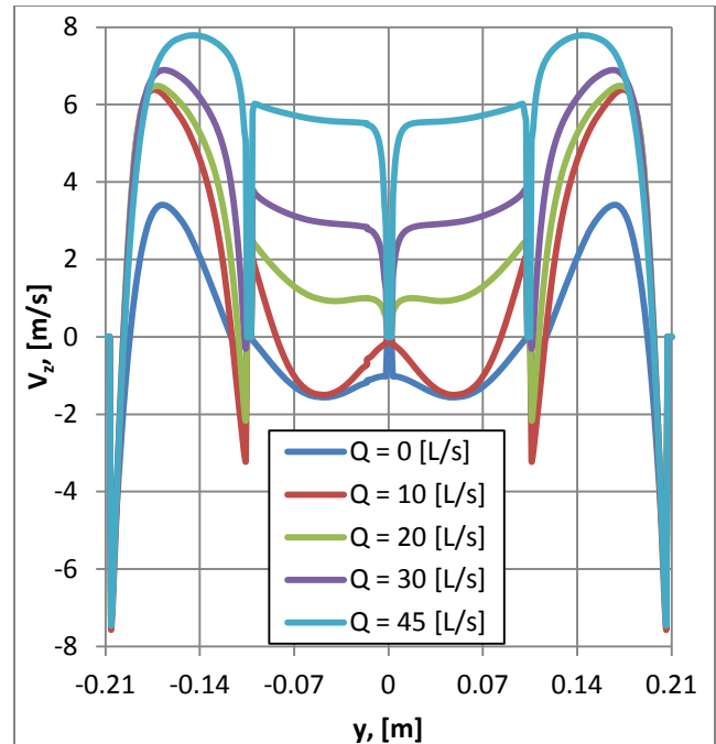
Fig. 11. Velocity z component distribution over y axis in the middle of the EMIP as a function of flowrate.
