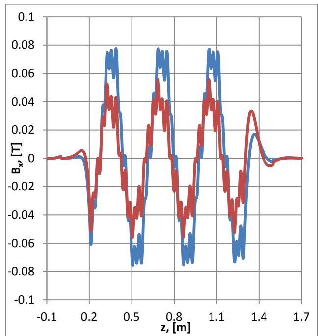
Fig. 8. Magnetic field distribution in the middle of the channel. Red: channel-1, blue: channel-2.
