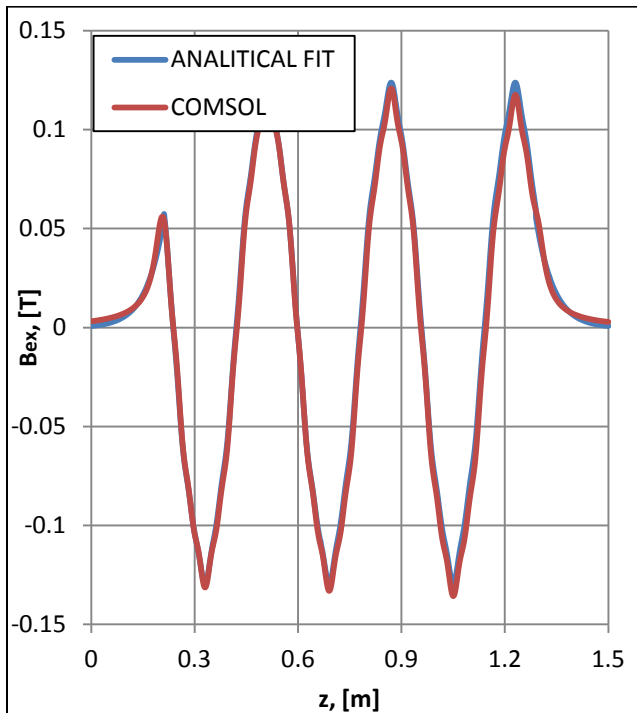
Fig. 6. COMSOL and analytical fit of the external magnetic field B_e x component in the middle of the channel.
