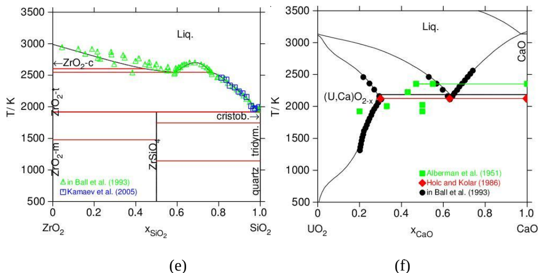
Figure 4: Calculated phase diagrams using the TAF-ID: (a) \text{UO}_2\text{-ZrO}_2 section assessed by A. Quaini (b) \text{U-O-Zr} at 2273 K section assessed by A. Quaini (c) \text{C-B-Fe} liquidus projection from M. Kurata (d) \text{U-B-C} at 1500 K assessed by N. Dupin (e) \text{ZrO}_2\text{-SiO}_2 assessed by N. Dupin (f) \text{UO}_2\text{-CaO} assessed by N. Dupin. A comparison with experimental data is reported when data are available.
