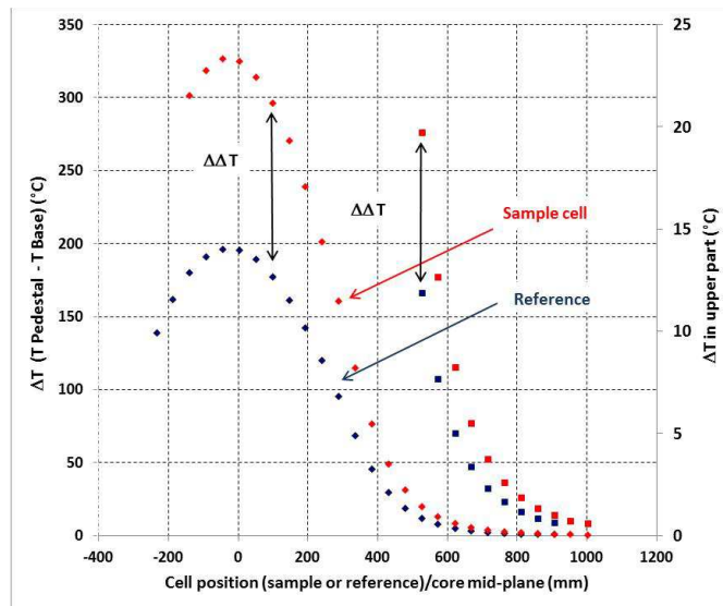
Fig. 4. \Delta T sample and \Delta T reference temperature differences in the 64South-East location at 64.35MWth recorded along the total displacement system stroke. The fissile height is located between -320 and +320mm vs the core mid-plane. Curves on the right should be read on the right scale which is a zoom for low values.
