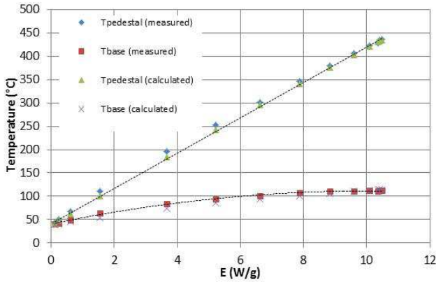
Fig. 8. Evolution of experimental and calculated temperatures of pedestal and base thermocouples of the sample cell with heating rate up to 10.5\text{W.g}^{-1} .
