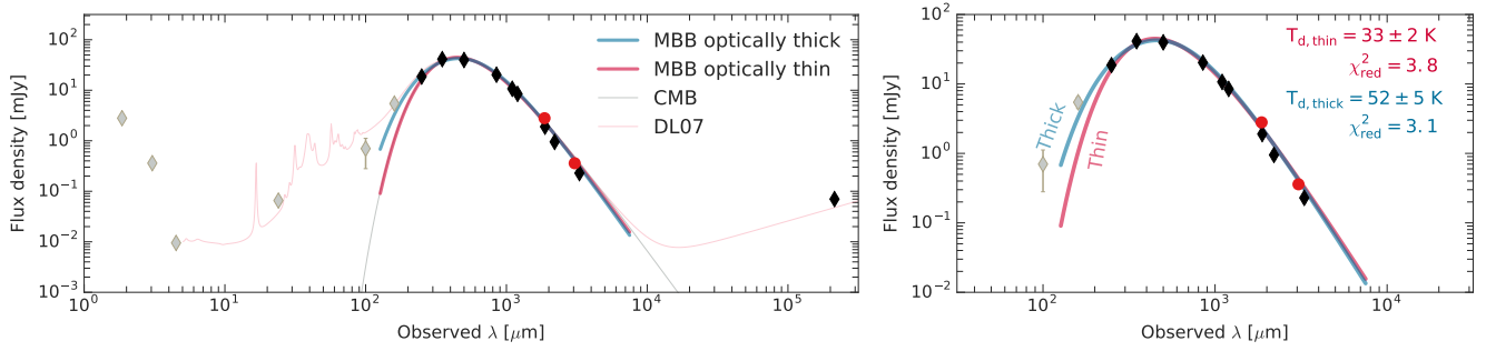
Fig. 2. Mid-IR to millimeter SED of GN20 in observed wavelength. Left: complement our new continuum measurements at 1.86 and 3.05 mm (red points) with existing photometry observations at observed and \lambda > 160 \mu\text{m} and \lambda \leq 160 \mu\text{m} (black and grey points, respectively), where the latter is omitted from the MBB modeling. Blue and red lines show the best-fit single-temperature MBB prescription assuming an optically thick ( \lambda_0 = 170 \pm 23 \mu\text{m} ) and thin dust emission, respectively. We also present the best-fit MBB model when accounting for the effect of the CMB (grey curve). The solid pink line shows the best-fit using the DL07 dust models, containing a diffuse ISM component and dust in PDR regions. The best-fit MBB parameters are listed in Table 1. Right: zoom-in of the rest-frame FIR part of the SED of GN20 when including the optically thick and thin MBB prescriptions. We note that the optically thick MBB model is a better match to the photometry observations at \lambda \leq 160 \mu\text{m} .
