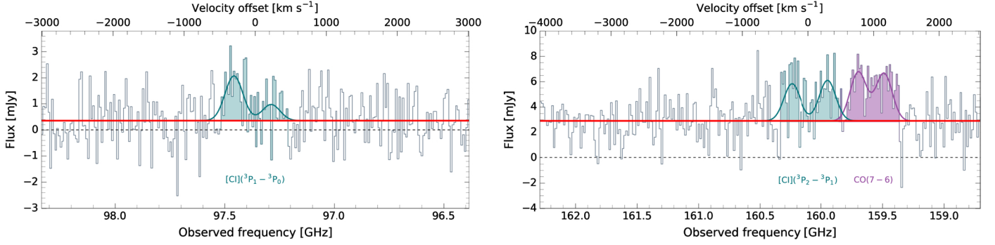
Fig. 1. Extracted spectra of the [C\text{ I}](^3P_1-^3P_0) line ( left ) and the [C\text{ I}](^3P_2-^3P_1) and \text{CO}(7-6) lines ( right ). Both spectra are binned in steps of 26\text{ km s}^{-1} . The colored areas indicate that the velocity ranges corresponding to detected line emission as labeled, which were used to obtain the velocity-integrated fluxes. Blue and purple solid lines show the best-fit double Gaussians, whereas the red line in each panel shows the continuum level. The velocity offset in both panels is relative to the expected frequency of the [C\text{ I}] lines at z = 4.0553 .
