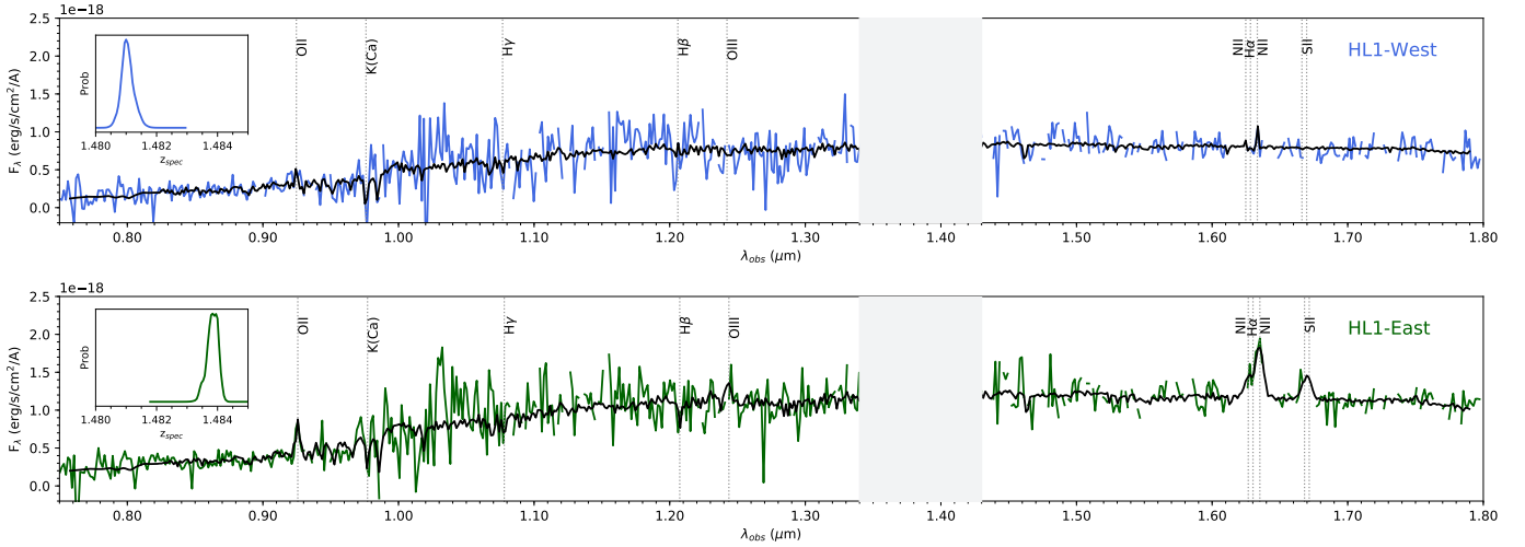
Fig. 6. Upper panel: VLT/X-shooter 1D spectra of HL1-West. Lower panel: VLT/X-shooter 1D spectra of HL1-East. The inset panels show the probability distribution function for the redshift. The black lines are the best spectral fits obtained with SLINEFIT.
