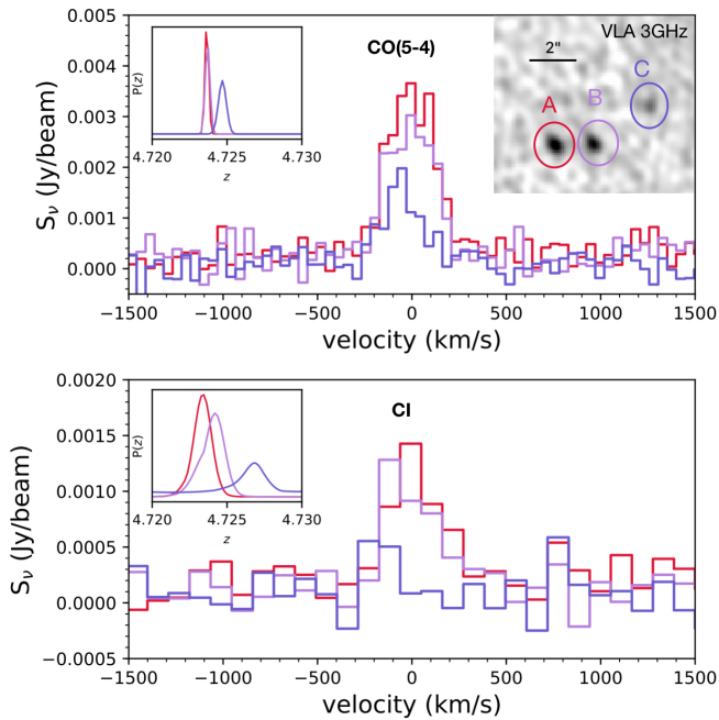
Fig. 3. Top panel: NOEMA observations of CO(5–4) lines of blob A (red), B (purple), and C (blue). Inset panel: VLA 3 GHz image of RV4. Bottom panel: [CI](1–0) lines of blob A (red), B (purple), and C (blue). The inset panels show the redshift probability distribution functions obtained with SLINEFIT.
