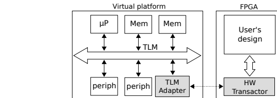
Fig. 1: Typical system built on a hybrid prototyping framework
