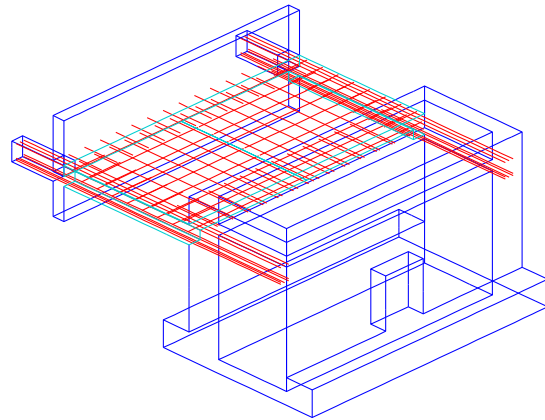
Figure 3: Finite element mesh: Reinforcement
