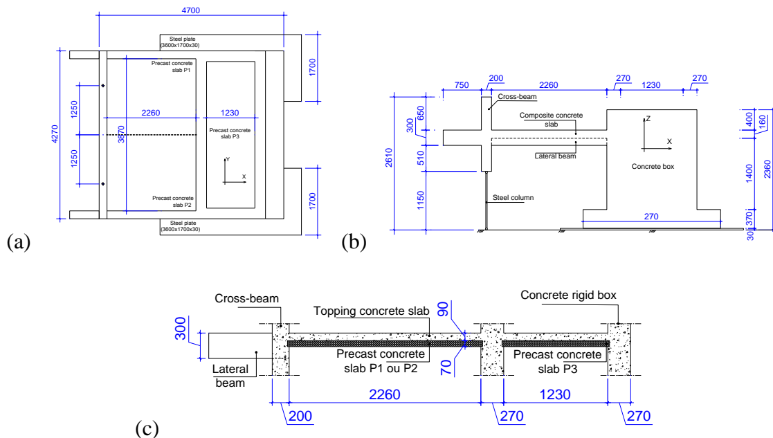
Figure 1: Dimensions of the model (unit: mm): (a) top; (b) elevation; (c) longitudinal section
