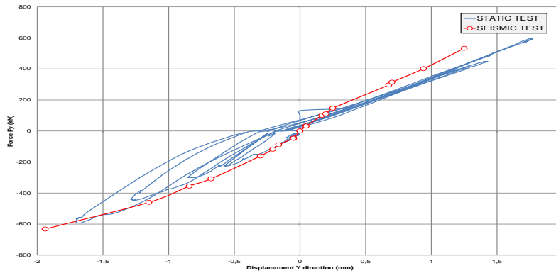
Figure 10: Force-Displacement curve – Comparison between Model-1 and Model-2
