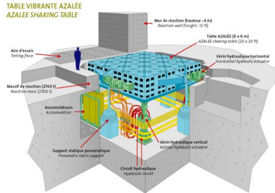
Figure 5: Seismic test set-up (Model-2)
