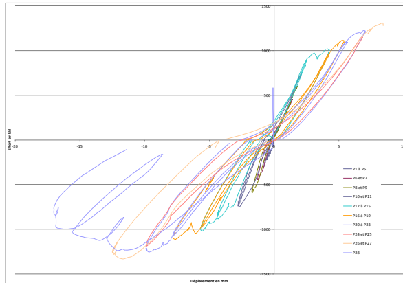
Figure 7: Force-displacement curves - Model-1
