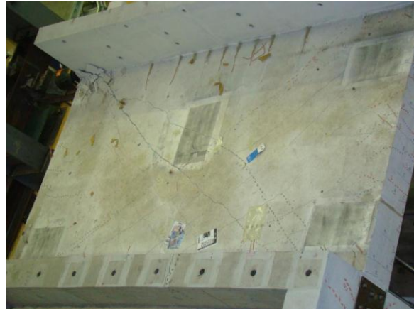
Figure 8: Ultimate state of the floor - Model-1 (after unloading; cracks partially closed)
