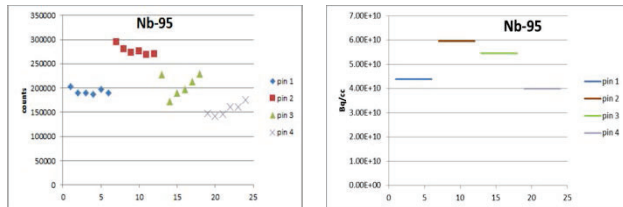
Fig. 2. Measured and calculated distributions ^{95}\text{Nb} per disk
