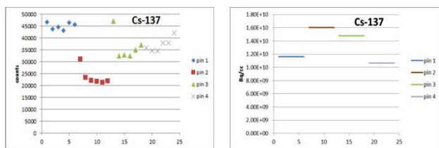
Fig. 3. Measured and calculated distributions ^{137}\text{Cs} per disk
