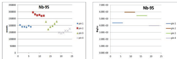
Fig. 2. Measured and calculated distributions ^{95}\text{Nb} per disk
