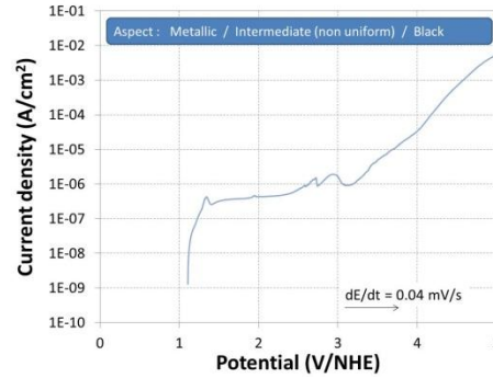
Fig. 3. Linear voltammetry of zirconium in nitric acid 6 mol/l at 30 °C ( dE/dt = 0.04 \text{ mV/NHE} )
