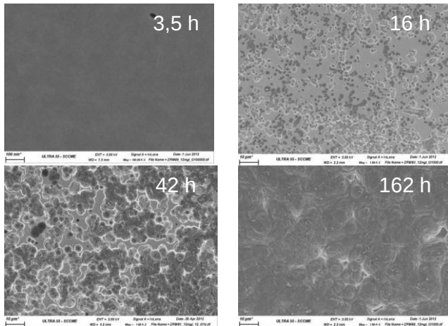
Fig. 15. SEM observations of zirconium corroded in \text{HNO}_3 6 mol/L, F 5,4 mg/L, 30 °C, 500 rpm, open circuit potential (initial oxide thickness: 11-12 nm)
