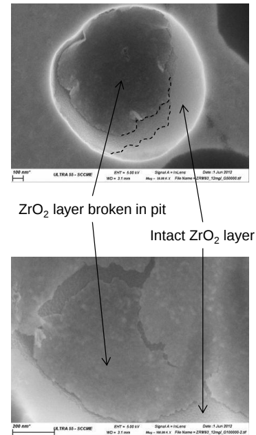
Fig. 16. SEM observations of zirconium corroded 16h in \text{HNO}_3 6 mol/L, F 5,4 mg/L, 30 °C, 500 rpm, open circuit potential (initial oxide thickness: 11-12 nm)
