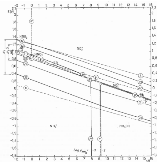
Fig. 1. Potential-pH diagram 16 of the nitrogen-water system at 25 °C
