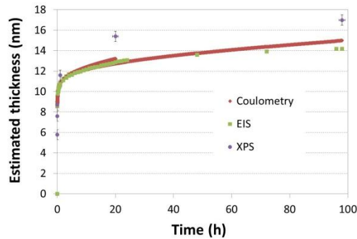
Fig. 9. Evolution of zirconium oxide thickness estimated by coulometry, EIS and XPS as a function of time (zirconium polarized at 1.4 V/NHE in \text{HNO}_3 6 mol/l at 30 °C).
