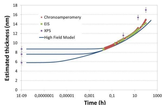
Fig. 12. Fitting of the High Field Model on experimental results (CA of zirconium at 1.4 V/NHE, respectively in \text{HNO}_3 6 mol/l at 30 °C)
