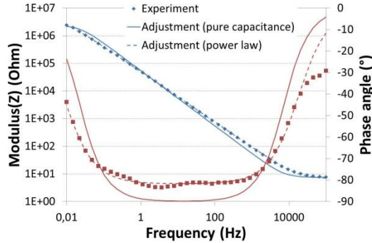
Fig. 8. Example of EIS spectrum
