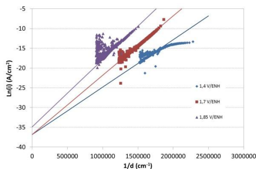
Fig. 11. Fitting of the “High Field Model” on experimental results (CA of zirconium at 1.4, 1.7 and 1.85 V/NHE, respectively in \text{HNO}_3 6 mol/l at 30 °C)
