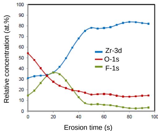
Fig. 18. XPS profile of zirconium corroded 140 h in \text{HNO}_3 6 mol/L, F 7.2 mg/L, 30 °C, 500 rpm, open circuit potential (initial \text{ZrO}_2 layer thickness 11-12 nm)
