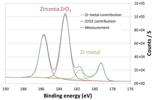
Fig. 7. Example of XPS Zr-3d spectrum
