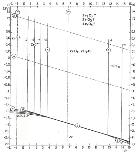
Fig. 2. Potential-pH diagram 16 of the zirconium-water system at 25 °C
