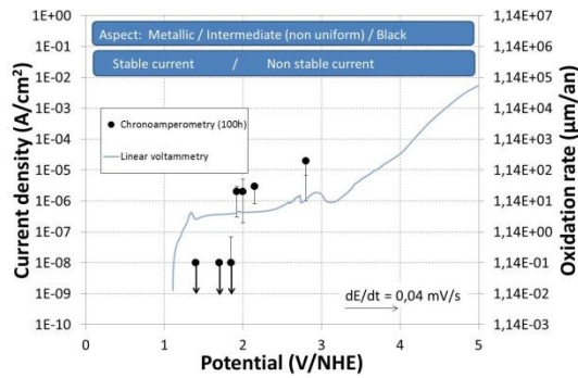
Fig. 6. Synthesis of the results (LV, CA) concerning the oxidation kinetics of zirconium in nitric acid 6 mol/l at 30 °C
