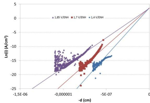
Fig. 10. Fitting of the “Point Defect Model” on experimental results (CA of zirconium at 1.4, 1.7 and 1.85 V/NHE, respectively in \text{HNO}_3 6 mol/l at 30 °C)
