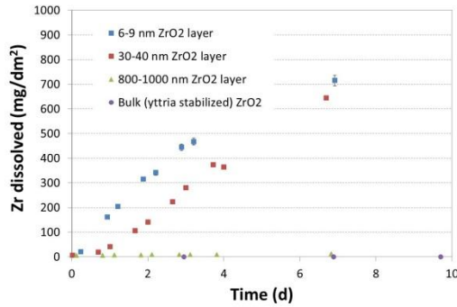
Fig. 17. Corrosion kinetics of zirconium in \text{HNO}_3 6 mol/L, F 5.4 mg/L, 30 °C, 500 rpm, open circuit potential (with different initial oxide thicknesses)
