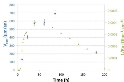
Fig. 14. Corrosion kinetics of zirconium in \text{HNO}_3 6 mol/L, F 5,4 mg/L, 30 °C, 500 rpm, open circuit potential (initial oxide thickness: 11-12 nm)
