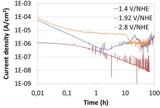
Fig. 5. Chronoamperometry at different potential of zirconium in nitric acid 6 mol/l at 30 °C (X axes expressed in logarithmic scale)
