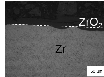
Fig. 4. Cross section of zirconium after the linear voltammetry in nitric acid 6 mol/l at 30 °C ( dE/dt = 0.04 \text{ mV/NHE} )
