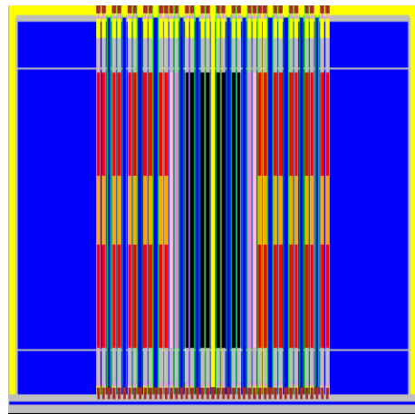
Fig. 4. EOLE UMZONE X-Z model for TRIPOLI-4®
