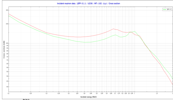
Fig. 18. 238 U capture cross section for JEFF-3.1.1 and 3.2
