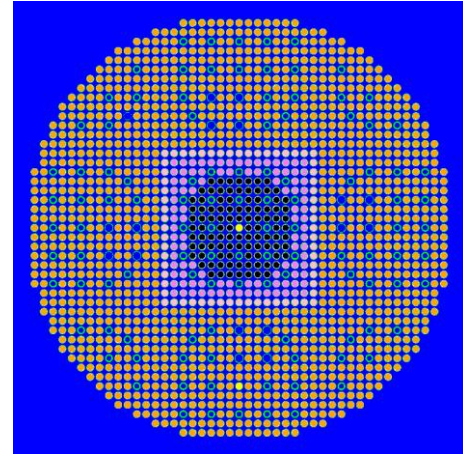
Fig. 3. EOLE UMZONE X-Y model for TRIPOLI-4®
