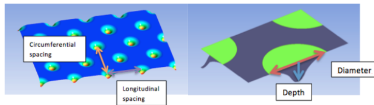
Figure 2: Parameters of the dimple texturing pattern
