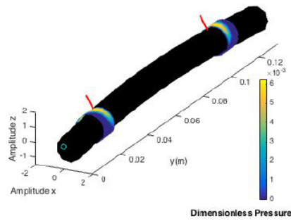
Figure 1: Hydrodynamic pressure projected on the rotating flexible shaft (in black) with rotating unbalance (in red).
