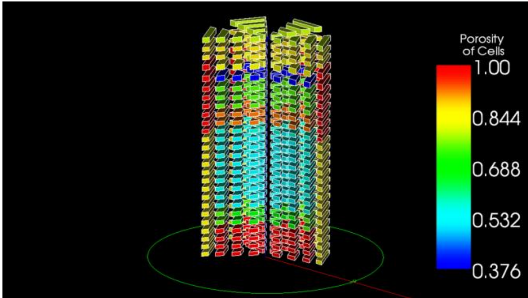
Figure 4. ROSA modelling visualization
