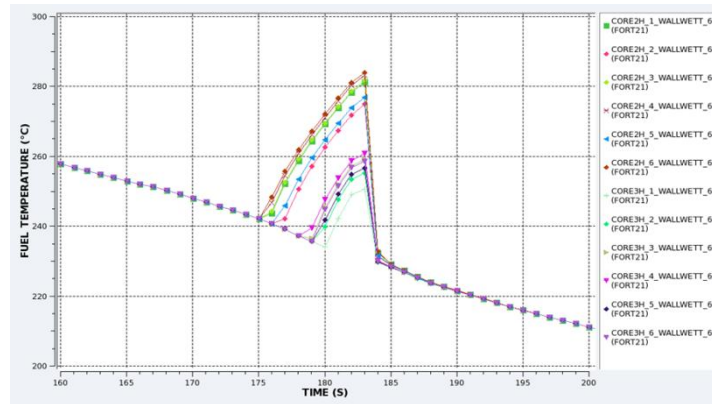
Figure 18. Fuel temperature vs time. Curves correspond to the hotter fuel rods values at 5 m from the bottom of the PV
