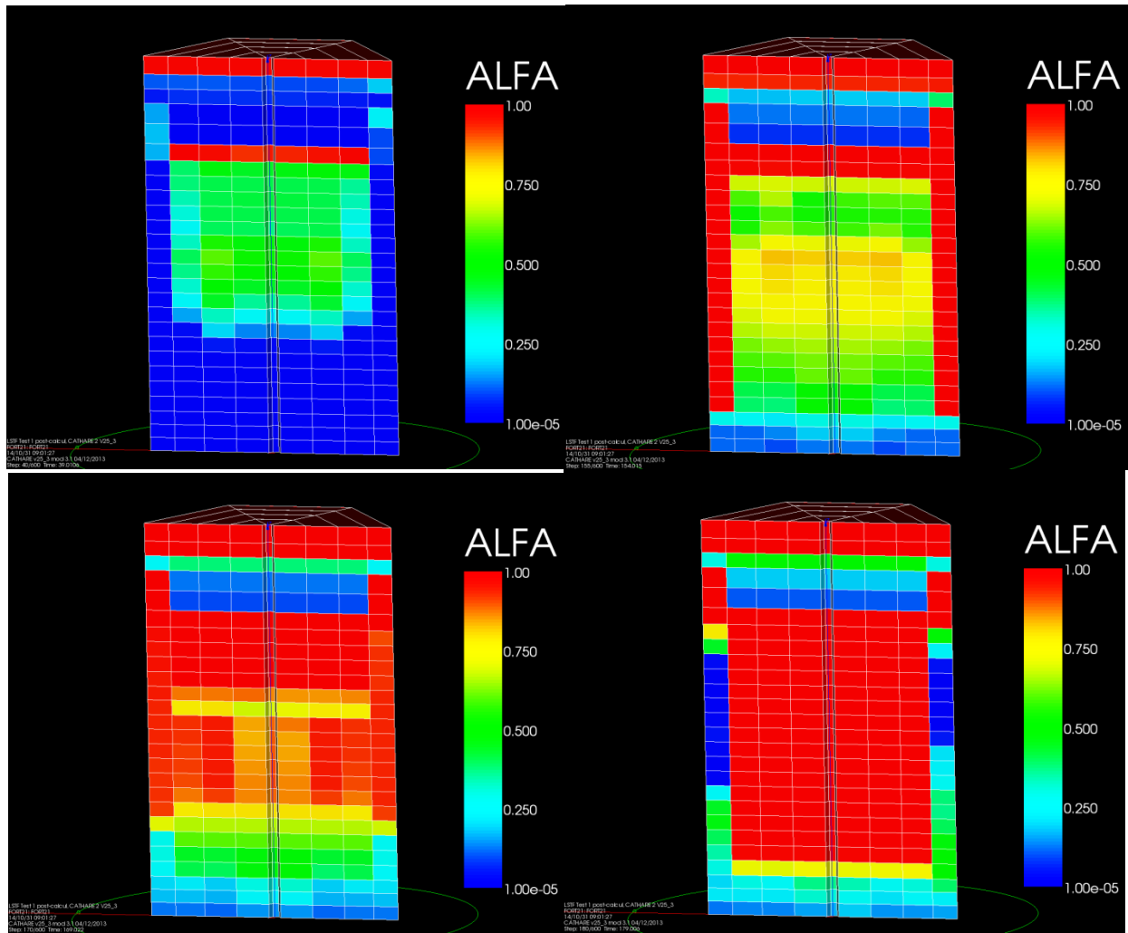
Figure 17. Void fraction vs time (39 s - 154 s - 169 s – 179 s)
