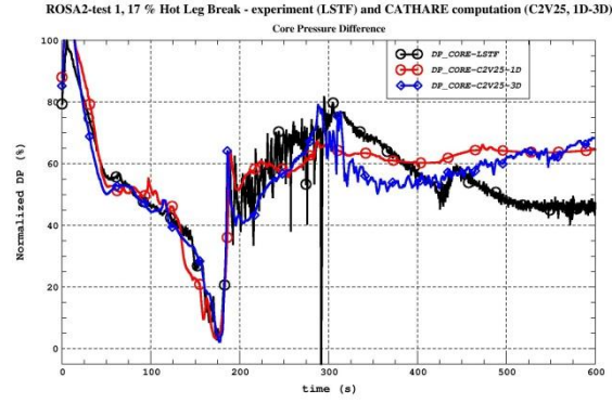
Figure 8. Core pressure difference
