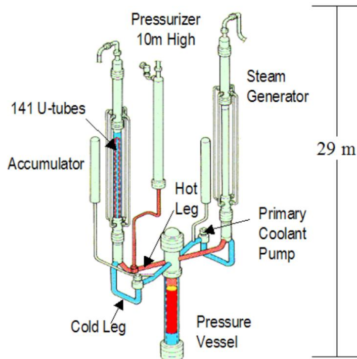
Figure 1. ROSA tests facility [1]
