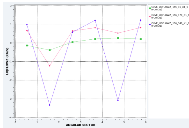
Figure 14. Liquid flowrate at 154 s vs angular sectors. Curves correspond to different crown (internal-green, medium-red and external-blue)
