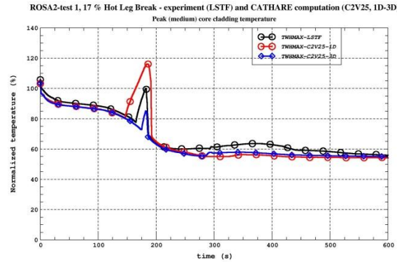
Figure 10. Temperature in the core rod
