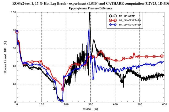
Figure 7. Upper plenum pressure difference
