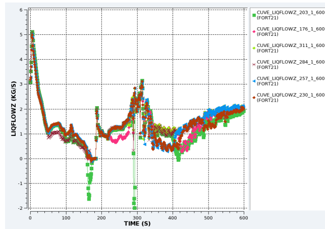
Figure 12. Liquid flowrate vs time. Curves correspond to the different sectors (1 to 6) in the second crown (the middle one) at about 5 m from the bottom of the PV
