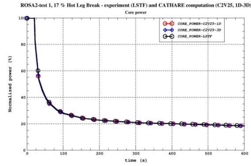
Figure 5. Core power
