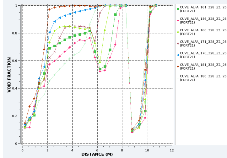
Figure 16. Void fraction vs PV elevation. Curves corresponds to different times (from 156 s to 186 s) measured in the external crown and sector 1. These values are taken in the end box level.
