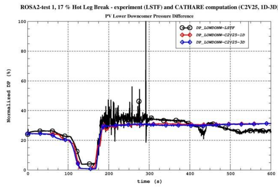
Figure 9. Lower downcomer pressure difference
