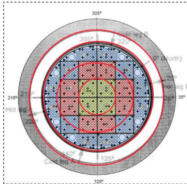
Figure 3. Radial core modelling
