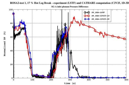
Figure 11. Pressure difference in the SG-A
