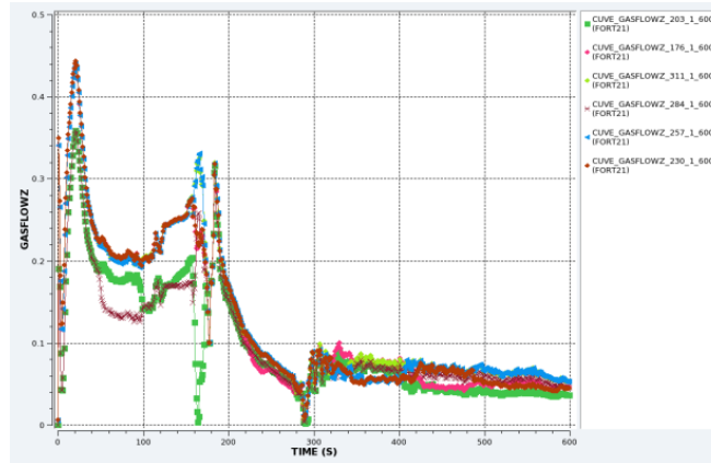
Figure 13. Gas flowrate vs time. Curves correspond to the different sectors (1 to 6) in the second crown (the middle one) at about 5 m from the bottom of the PV
