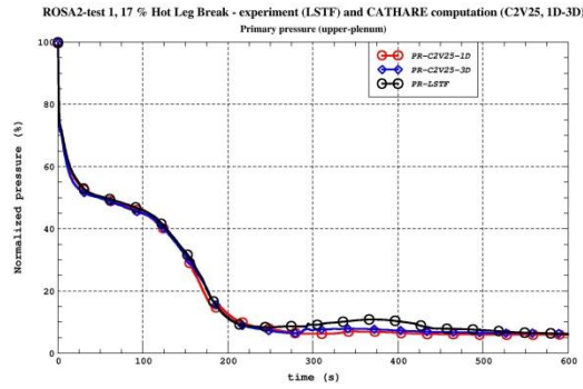
Figure 6. Pressure trend
