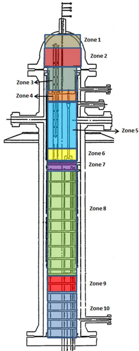
Figure 2. Axial modelling
