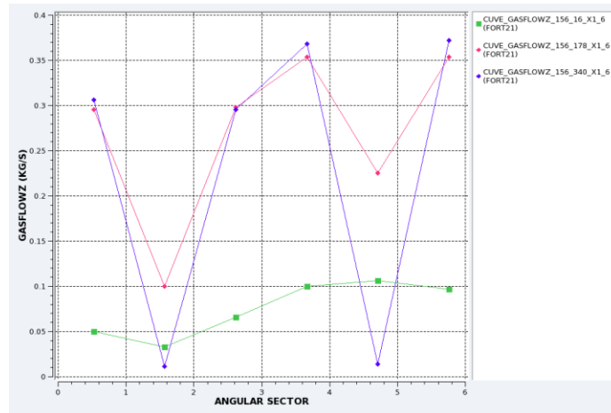
Figure 15. Gas flowrate at 154 s vs angular sectors. Curves correspond to different crown (internal-green, medium-red and external-blue)
