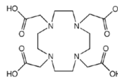
Figure 1: Developed formula of the DOTA ligand
