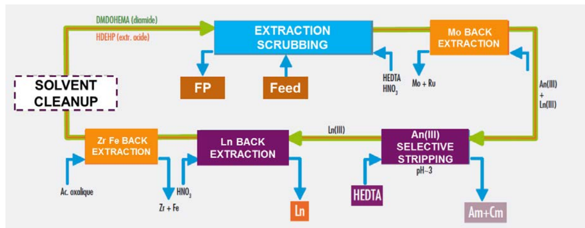
Fig.3: the DIAMEX/SANEX process flowsheet [6].
