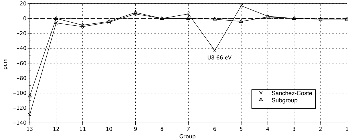
Figure 7. U235 absorption for a \text{UO}_2\text{Gd}_2\text{O}_3 assembly.
