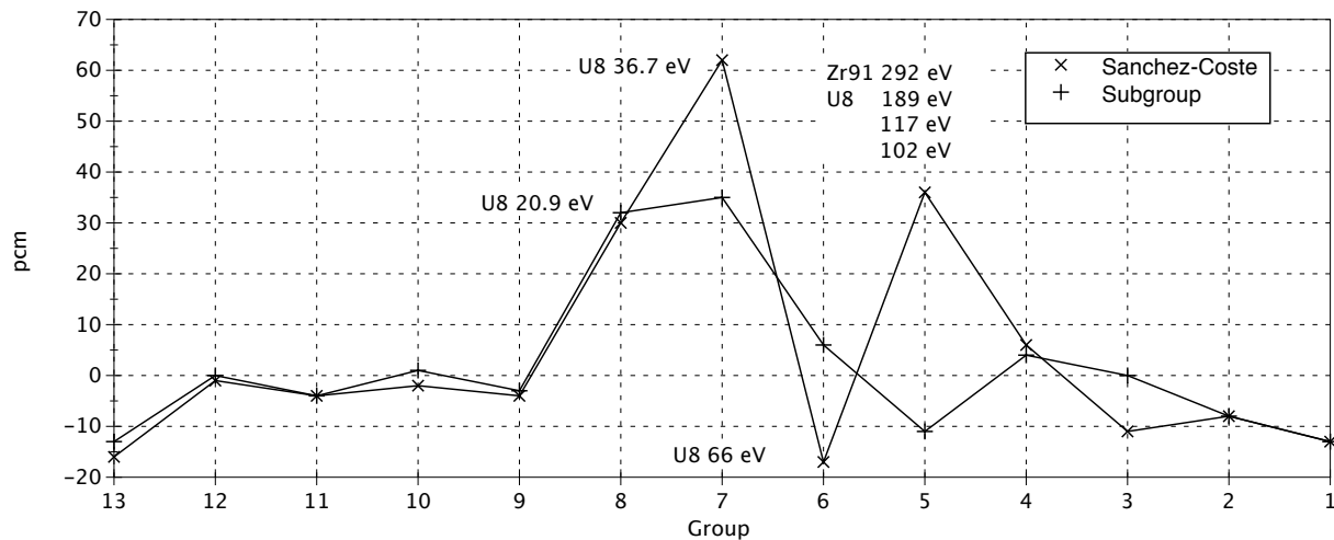
Figure 8. U238 absorption for a \text{UO}_2\text{Gd}_2\text{O}_3 assembly.
