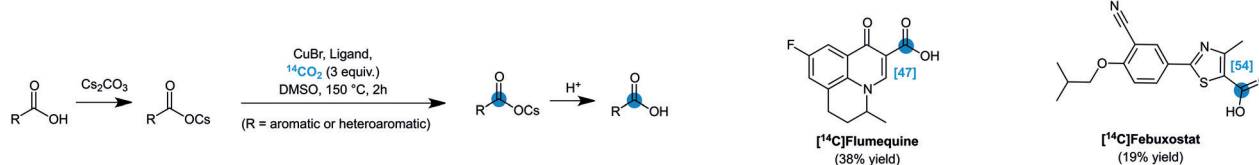
Figure 1. CIE reactions developed by the groups of Gauthier, Baran, and Cantat and Audisio, with examples of prepared 14 C-labelled compounds. The percentage of carbon-14 isotope incorporation is given in blue in square brackets, and the yields of the isolated labelled acids are given in black in parentheses.
