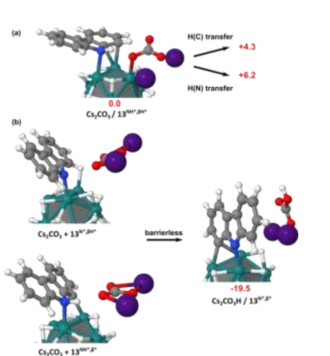
Figure 11: Ability of \text{Cs}_2\text{CO}_3 to coordinate to the catalyst surface and to adapt the role of a proton acceptor in the N-H and C-H activation step.
