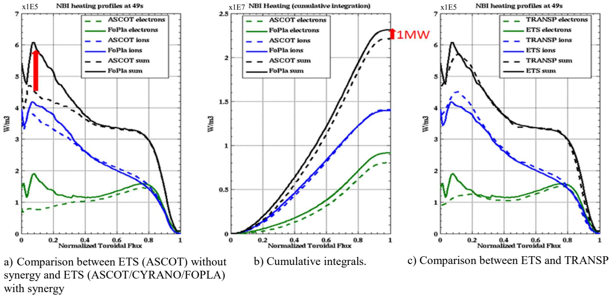
FIGURE 3: JET pulse 92436 at t=49s with ETS (ASCOT/CYRANO/FOPLA) and TRANSP (NUBEAM/TORIC/FPP)
