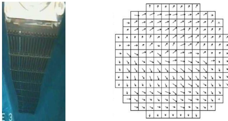
Figure 1. Picture of a deformed fuel assembly and horizontal displacements at mid core height.
