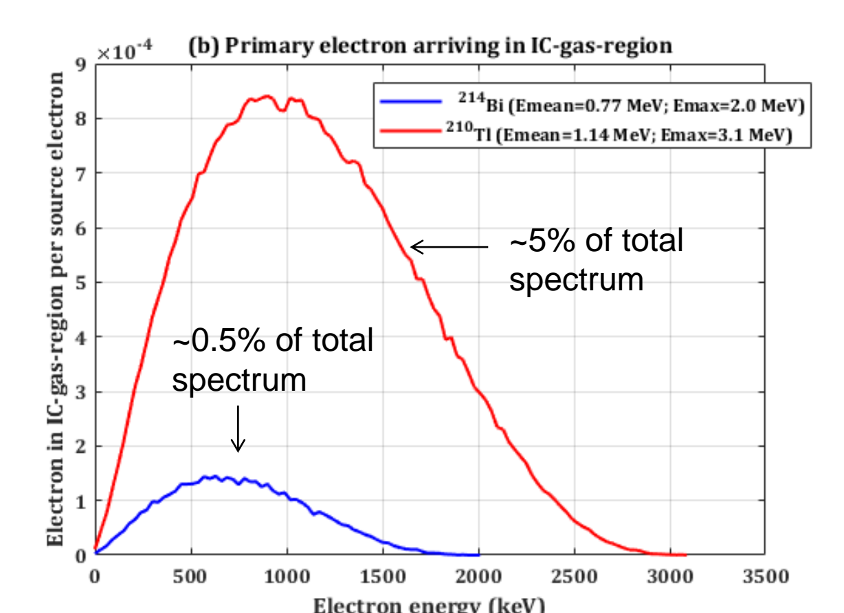
Fig. 8: (a) Primary electron released in the source from the total \beta spectrum of ^{214}\text{Bi} and ^{210}\text{Tl} (b) Primary electron released in the source and arriving in IC gas region
