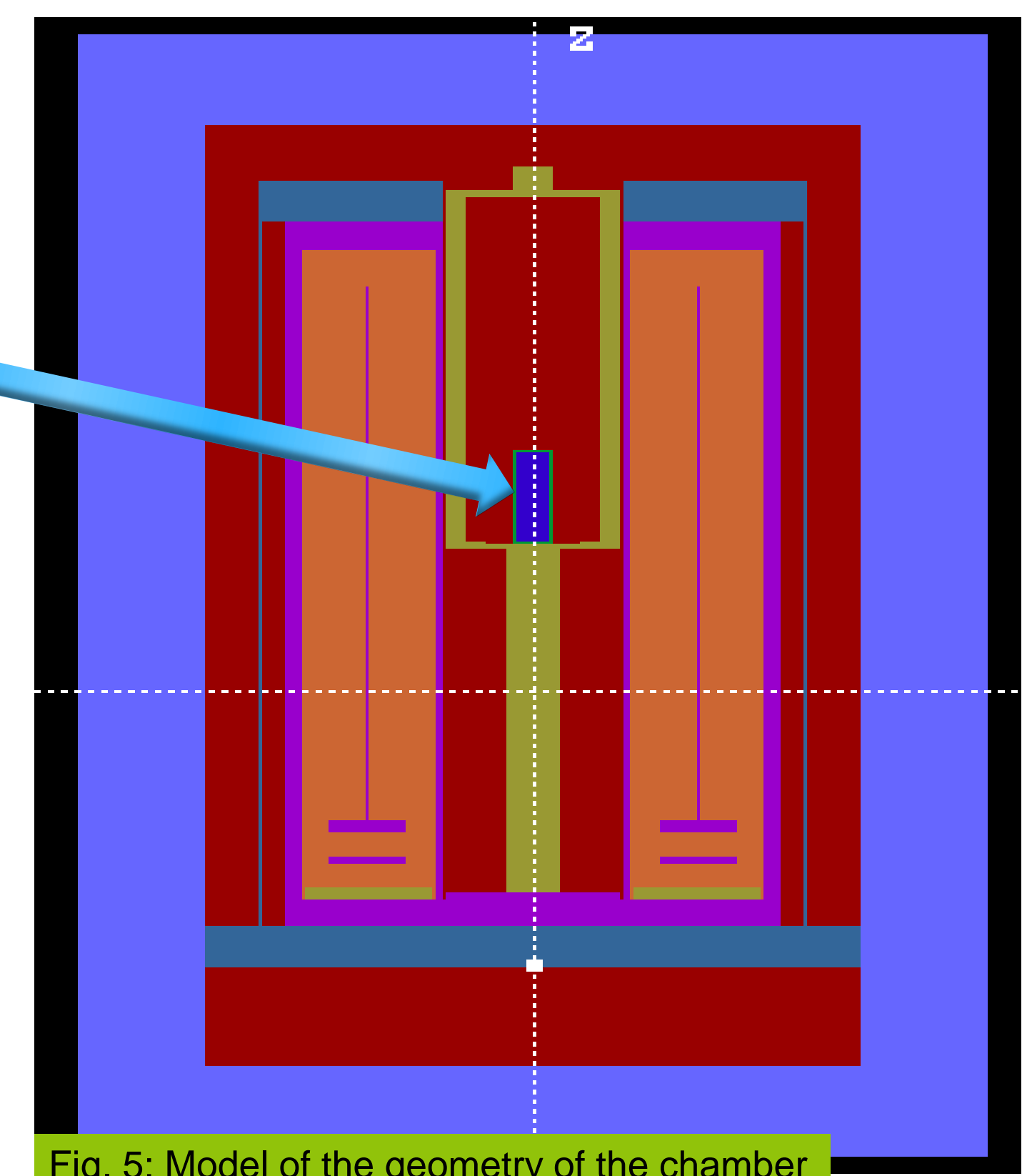
Fig. 5: Model of the geometry of the chamber
