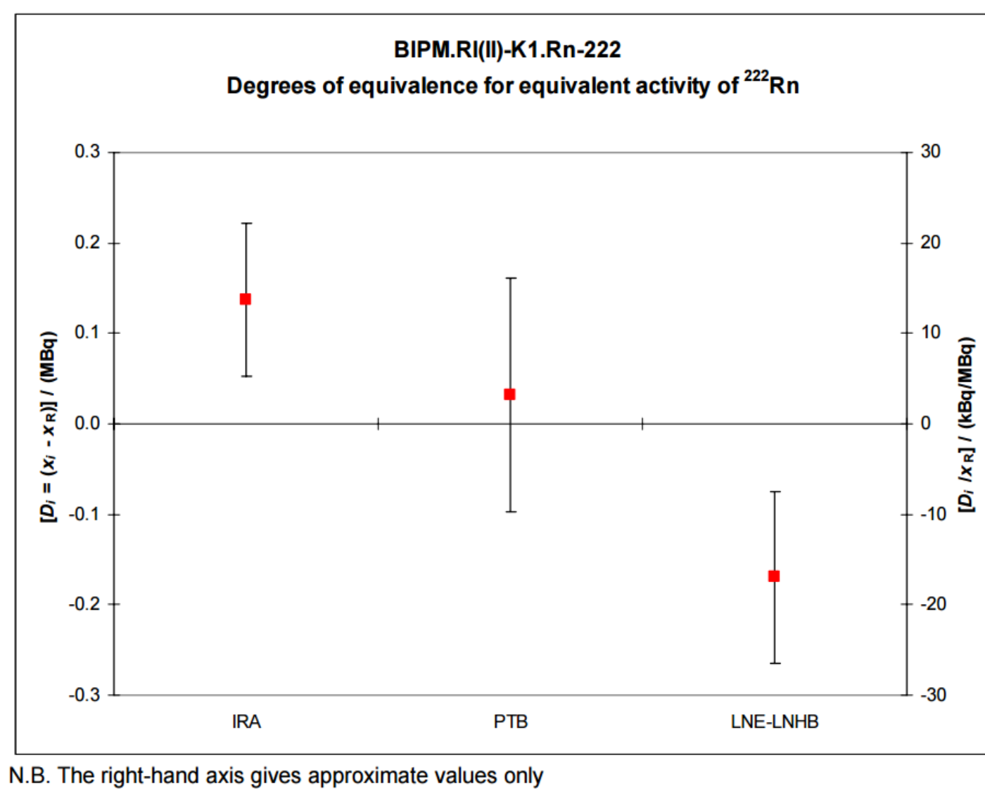
Fig. 1: Degrees of equivalence with the KCRV for ^{222}\text{Rn}
