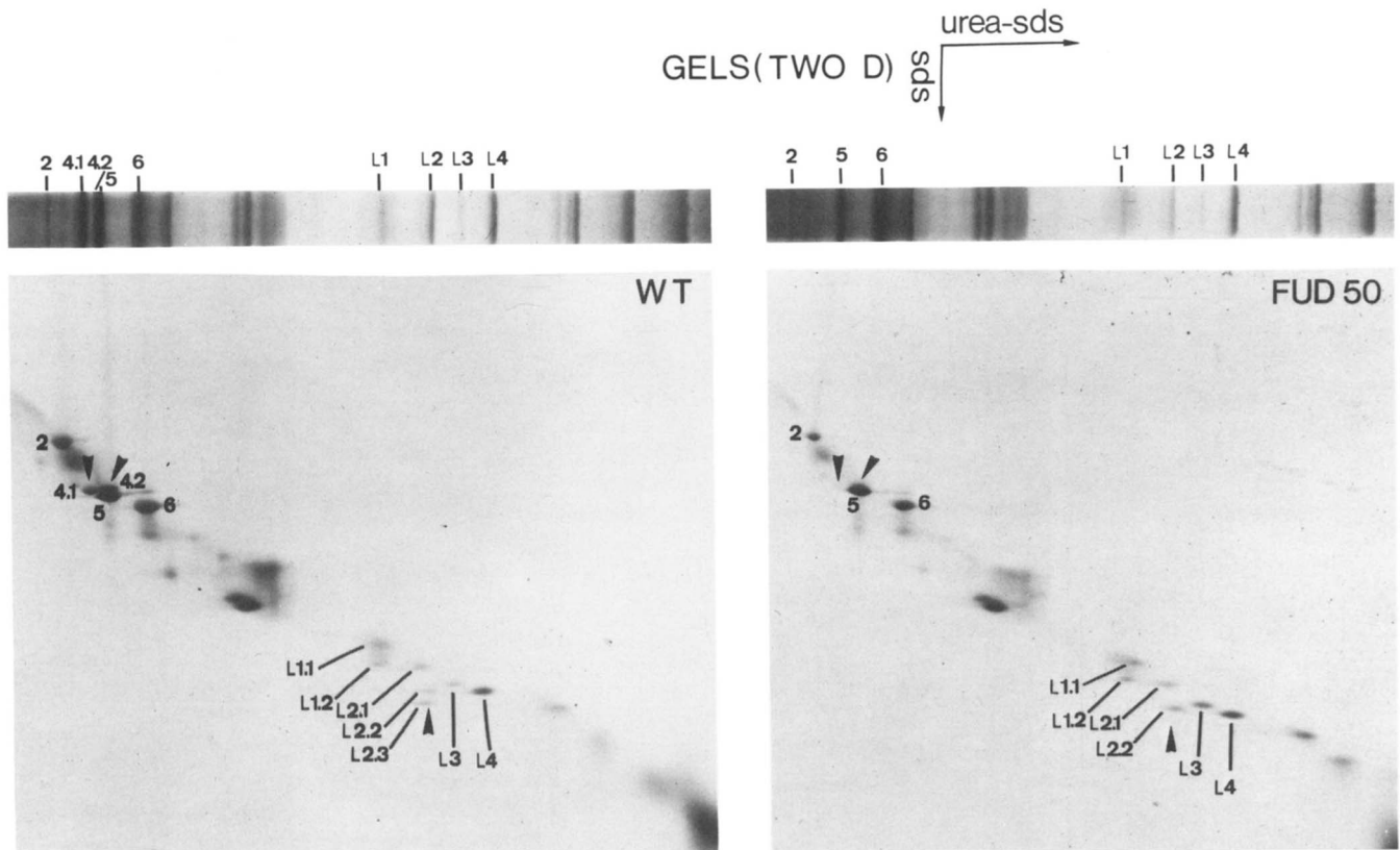
FIG. 5. Same as Fig. 4 using two-dimensional SDS-gel electrophoresis. First dimension, 12–18% acrylamide gel with 8 M urea. Second dimension, 7.5–15% acrylamide gel. Note the absence (arrows) of bands 4.1 and 4.2 ( \alpha and \beta ) and L2.3 ( \epsilon ) in the FUD50 thylakoids. In contrast, CF 0 subunits IV (L2.1) and I (L3) are clearly visible.
