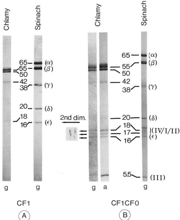
FIG. 1. Subunit composition of CF 1 (A) and CF 1 ·CF 0 (B) preparations from spinach and C. reinhardtii analyzed on 12–18% acrylamide gels containing 8 M urea. Subunits in the complexes from spinach are identified by their name and apparent M_r . Subunits in the complexes from C. reinhardtii are indicated by their apparent M_r only. A 20-kDa subunit is observed in CF 1 ·CF 0 from [ ^{14} C]acetate stationary labeled cells of C. reinhardtii after autoradiography (a) but not by Coomassie Blue staining (g). The inset corresponds to the 18–16-kDa region after two-dimensional gel electrophoresis (first dimension, 12–18% acrylamide with 8 M urea; second dimension, 7.5–15% acrylamide) of CF 0 ·CF 1 preparations.
