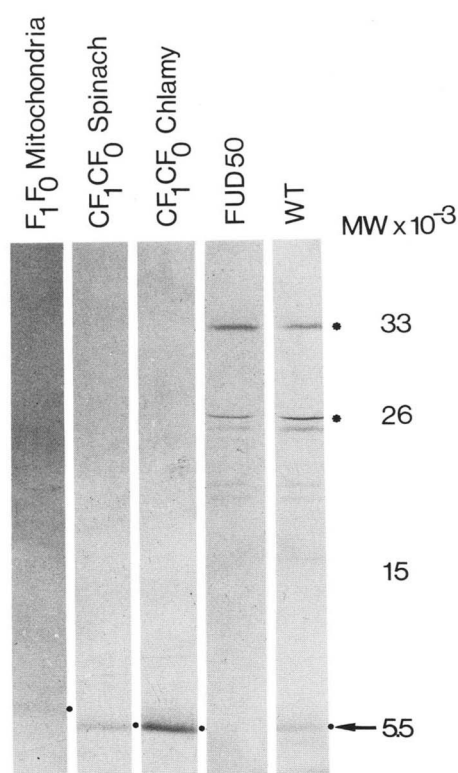
FIG. 6. Autoradiogram of a urea-SDS gel loaded with [ ^{14}\text{C} ] DCCD-labeled ATP synthases from various sources and thylakoid membranes from WT and FUD50 strains. Note the presence of a 5.5-kDa labeled band in purified complexes and in WT thylakoid membranes, but its absence in FUD50 thylakoid membranes. Asterisk (*) points to several labeled membrane polypeptides of unknown function present in the WT and FUD50 strains.
