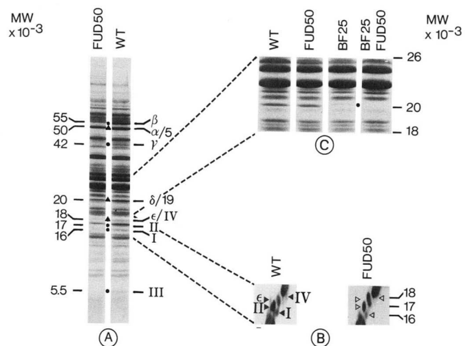
FIG. 2. A, polypeptide patterns of thylakoid membranes from the WT and FUD50 mutant lacking the chloroplast ATP synthase. Same gel system as described in the legend to Fig. 1. Identification of each ATP synthase subunit, lacking in the FUD50 mutant, and the corresponding apparent M_r are given on the left and right, respectively. 5–19 correspond to PSII polypeptides numbered following the nomenclature of Chua and Bennoun (14). B, two-dimensional gel electrophoresis after silver staining of the 18–16-kDa region of the FUD50 and WT thylakoids. First dimension, 12–18% acrylamide with 8 M urea; second dimension, 7.5–15% acrylamide gel; note the absence (white arrows) of two bands in the 18-kDa region in the FUD50 thylakoids. Also indicated are the losses of the 17- and 16-kDa polypeptides. C, enlargement of the 18–26-kDa region of a similar gel loaded with SDS-solubilized thylakoid membranes from the WT, the FUD50 mutant lacking the ATP synthase, the BF25 mutant specifically lacking in the OEE 2 subunit of PSII, and the double mutant BF25/FUD50. Note the presence of a minor 20-kDa band remaining in BF25 which is lacking in the double mutant.
