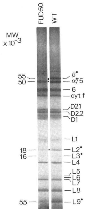
FIG. 4. Autoradiogram of chloroplast translates in thylakoid membranes from the WT and F mutant. Cells were pulse-labeled for 45 min with [ 14 C]acetate in the presence of cycloheximide. Molecular weights are indicated in positions corresponding to ATP synthase subunits of chloroplast origin (*). Polypeptides are named after Delepelaire (13). L2, L3, and L9 correspond respectively, to subunits IV, I, and III.
