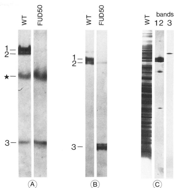
FIG. 7. Nondenaturing electrophoresis (6% acrylamide gels) of proteins extracted by a chloroform shock from WT and FUD50 thylakoid membranes. A, silver staining; B, immunoblots with antibodies against the \beta subunit of \text{CF}_1 . Three bands, 1–3, are recovered from WT, whereas only the region of band 3 remains visible in the case of FUD50. Asterisk (*) indicates a band occasionally observed after silver staining in these experiments. C, urea/SDS electrophoresis of bands 1–3 (silver staining). Bands 1 and 2 contain \text{CF}_1 subunits, but band 3 contains a single 70-kDa polypeptide.
