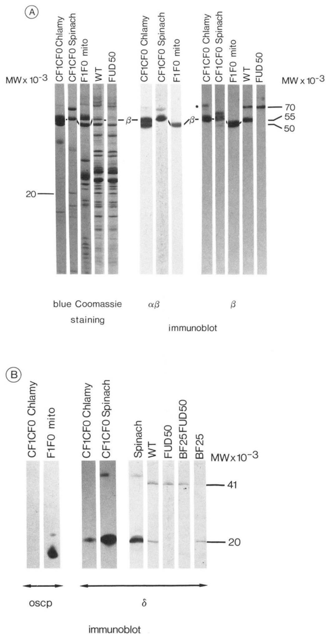
FIG. 3. A , ATP synthases from various sources and thylakoid membranes from WT and FUD50 after urea/SDS electrophoresis and Coomassie Blue staining or subjected to immunoblotting and probed with antibodies directed against \alpha/\beta or \beta subunits. Antibody recognition patterns of the 55-kDa bands in the different samples (-----) indicate that they correspond to the \beta subunit in chloroplasts from spinach and C. reinhardtii but to the \alpha subunit in beef heart mitochondria. Indicated by an asterisk (*) is the 70-kDa polypeptide from C. reinhardtii which is present in CF 0 ·CF 1 preparations and in the WT and FUD50 thylakoids. B , ATP synthases from various sources and thylakoid membranes from spinach, WT, FUD50, BF25, and BF25/FUD50 after urea/SDS electrophoresis, subjected to immunoblotting, and probed with antibodies directed against the OSCP or \delta subunits. A cross-reaction between 20-kDa polypeptides in spinach and C. reinhardtii is observed in purified complexes in WT and BF25 thylakoid membranes, but is absent in the FUD50 and BF25/FUD50 thylakoid membranes which lack the ATP synthase. Also visible is a cross-reaction with a 41-kDa polypeptide of unknown origin, the presence of which is not related to the presence of the ATP synthase in C. reinhardtii .
