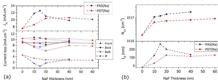
Figure 6. a) Top: evolution of the J_{SC} of the best solar cells as function of the NaF thickness used in the PAS (blue) and PDT (red) processes. Bottom: evolution for the same solar cells of the current loss in the front electrode (reflection + absorption in ZnO:Al/ZnO/CdS), the back electrode (absorption in MoS 2 /Mo), in the bulk of the absorber due to insufficient collection length and at the CZTS/CdS interface due to recombination. b) Top: Evolution of the apparent carrier density measured by C–V as function of the NaF thickness used in the PAS (blue) and PDT (red) processes. Bottom: Evaluation of the carrier diffusion length in the CZTS as function of the NaF thickness used in the PAS (blue) and PDT (red) processes.
