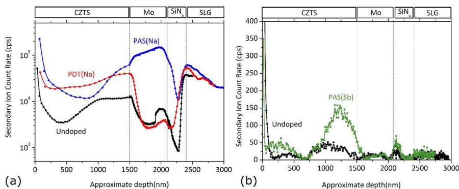
Figure 2. a) Na ToF-SIMS profiles in CZTS/Mo/SiN x /SLG structures and (b) Sb ToF-SIMS profiles in CZTS/Mo/SiN x /SLG structures. The position of the different layers (CZTS, Mo, SiN x , SLG) is estimated from the Cu, Zn, Sn, S, Mo, Si N, and O profiles not shown.
