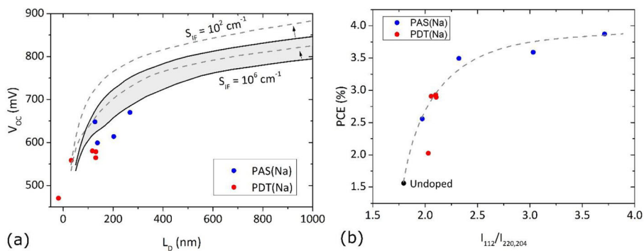
Figure 7. a) V_{OC} of the CZTS-based solar cells for both PAS(Na) and PDT(Na) processes as function of L_D estimated from EQE simulations. The solid lines represents device simulation (extracted from ref. [32] for a 1.45 eV bandgap and assuming \mu = 100 \text{ cm}^2 \text{ V}^{-1} \text{ s}^{-1} ) with different CZTS/CdS ( S_{IF} ) and Mo/CZTS ( S_B ) interface recombination velocities: for the top curve, S_{IF} = 10^2 \text{ cm}^{-1} and S_B = 10^2 \text{ cm}^{-1} and for the bottom curve, S_{IF} = 10^6 \text{ cm}^{-1} and S_B = 10^7 \text{ cm}^{-1} . Recombination at the Mo/CZTS interface has a minor impact since the carrier collection length is smaller than the absorber thickness. Dashed lines represents same simulations assuming \mu = 40 \text{ cm}^2 \text{ V}^{-1} \text{ s}^{-1} . b) PCE of the CZTS-based solar cells for both PAS(Na) and PDT(Na) processes as function of the preferential orientation of the absorber. The dashed line is a guide for the eyes.
