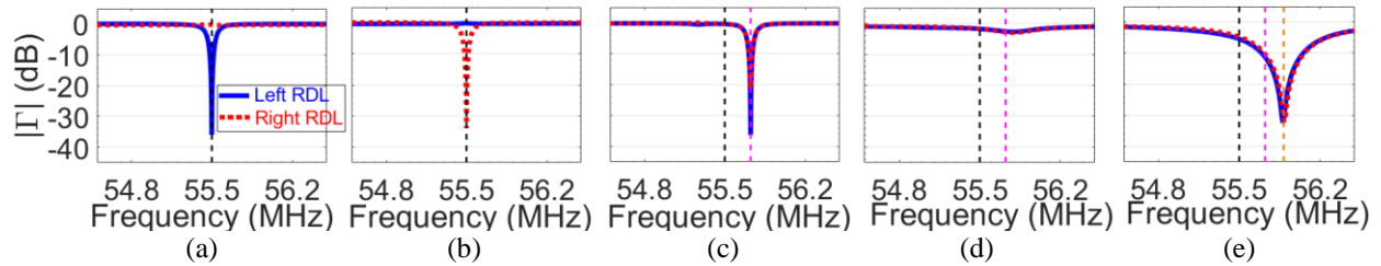
FIGURE 3. Example for the manual tuning of a full-launcher (see text). The black, magenta and orange vertical line correspond respectively to F_0 , F_0+\Delta F_0 and F_0+\Delta F_1 . Here F_0=55.5\text{MHz} . The data is obtained from numerical modeling involving S-matrices computed on HFSS and RF network computations performed on SIDON [21].
