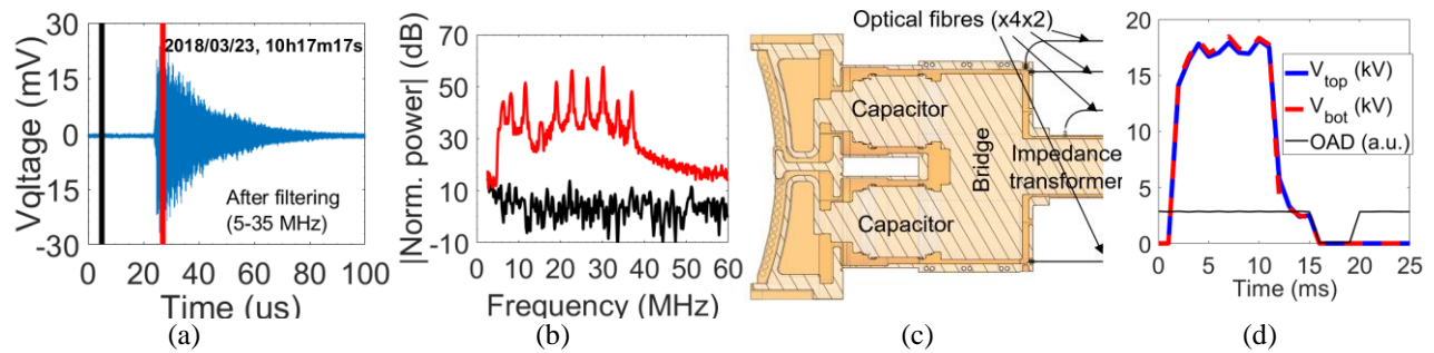
FIGURE 8. (a) Typical arc signature as measured by the SHAD system. (b) Short-term Fourier transforms at the 2 \mu s black and red time-intervals of (a). (c) Poloidal cross-section through a poloidal pair of straps illustrating the location of the optical fibres that are used for arc detection. (d) Validation of the Optical Arc Detection (OAD).
