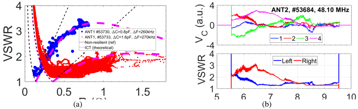
FIGURE 7. (a) The successful employment of the manual tuning strategy in experiments on plasma. (b) Operation of the real-time controlled impedance-matching. Top: time-traces for V_C (the vector of signals that are proportional to the capacitors velocities). A positive (resp. negative) value for V_C leads to a capacitance increase (resp. decrease). Bot: time-traces of the VSWR.
