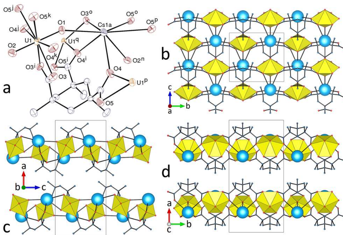
Figure 6. (a) View of complex 6. Displacement ellipsoids are drawn at the 40% probability level and hydrogen atoms are omitted. Symmetry codes: i = x, 1/2 - y, z ; j = 1/2 - x, y + 1/2, z - 1/2 ; k = 1/2 - x, -y, z - 1/2 ; l = x, y, z - 1 ; m = x, 1/2 - y, z - 1 ; n = x, y, z + 1 ; o = 1/2 - x, y + 1/2, z + 1/2 ; p = 1/2 - x, -y, z + 1/2 ; q = 1/2 - x, 1 - y, z + 1/2 . (b) View of the dimeric assembly with uranium coordination polyhedra yellow and caesium cations shown as blue spheres. (c) and (d) Two views of the packing with layers edge-on. Only one position of the disordered caesium atom is shown in all views.
