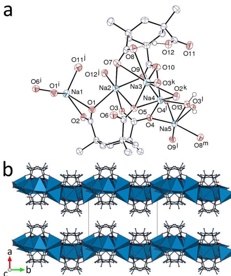
Figure 1. (a) View of complex 1 . Displacement ellipsoids are drawn at the 50% probability level. Carbon-bound hydrogen atoms are omitted and the hydrogen bond is shown as a dashed line. Symmetry codes: i = -x, 2 - y, 1 - z ; j = x, 3/2 - y, z + 1/2 ; k = x, 3/2 - y, z - 1/2 ; l = -x, 1 - y, 1 - z ; m = -x, y - 1/2, 1/2 - z . (b) Packing with layers viewed edge-on, showing sodium coordination polyhedra.
