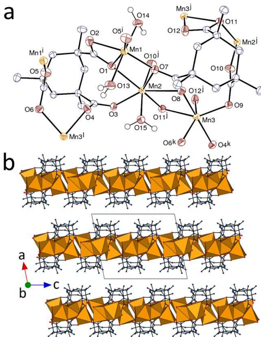
Figure 3. (a) View of complex 3 . Displacement ellipsoids are drawn at the 50% probability level. Carbon-bound hydrogen atoms are omitted. Symmetry codes: i = 1 - x, -y, -z ; j = 1 - x, 1 - y, -z ; k = 1 - x, y + 1/2, 1/2 - z ; l = 1 - x, y - 1/2, 1/2 - z . (b) Packing with layers viewed edge-on, showing manganese coordination polyhedra.
