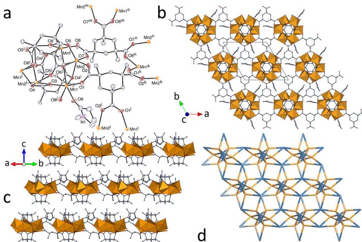
Figure 5. (a) View of complex 5. Displacement ellipsoids are drawn at the 30% probability level and hydrogen atoms are omitted. Symmetry codes: i = y - x + 1, 1 - x, z ; j = 1 - y, x - y, z ; k = 1 - y, x - y + 1, z ; l = y - x, 1 - x, z ; m = 2 - y, x - y + 1, z ; n = y - x + 1, 2 - x, z ; o = x + 1, y + 1, z . (b) View of the dimeric assembly showing manganese coordination polyhedra. (c) Packing with layers viewed edge-on. (d) Nodal representation of the network (orange, manganese; blue, tricarboxylate ligand). Orientation slightly rotated with respect to that in (b).
