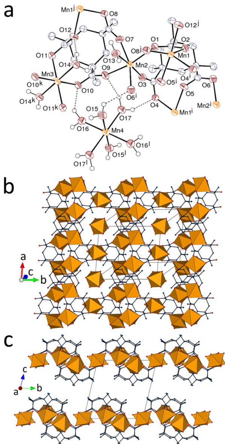
Figure 4. (a) View of complex 4. Displacement ellipsoids are drawn at the 30% probability level. Carbon-bound hydrogen atoms are omitted and hydrogen bonds are shown as dashed lines. Symmetry codes: i = -x, 1 - y, 2 - z ; j = 1 - x, 1 - y, 2 - z ; k = 1 - x, 2 - y, 2 - z ; l = -x, 2 - y, 2 - z . (b) View of the dimeric assembly showing manganese coordination polyhedra. (c) Packing with layers viewed edge-on.
