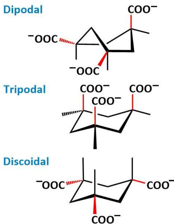
Scheme 1. The three conformations of \text{Kta}^{3-} found in its metal ion complexes.
