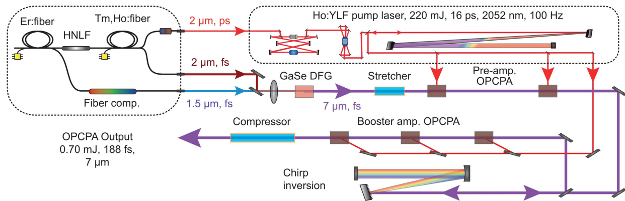
Fig. 3. Layout of the 7 \mu\text{m} OPCPA. The mid-IR seed is generated using the two broadband femtosecond outputs from a three-color fiber front-end via DFG. Afterward, the mid-IR pulses are stretched in a dielectric bulk and consecutively amplified in a pre-amplifier and a booster amplifier separated with a chirp inversion stage. Maximum efficiency of the OPCPA is achieved by tailoring the seed-to-pump pulse durations in the pre-amplifier and booster amplifier. The broadband high-energy mid-IR pulses are recompressed using a dielectric bulk rod of \text{BaF}_2 .
