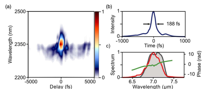
Fig. 4. Pulse characterization of the 7 \mu\text{m} compressed pulses. (a) Measured third-harmonic FROG, (b) the retrieved pulse envelope with 188 fs FWHM duration, and (c) measured (filled gray) and retrieved spectrum (red line) and phase (green line).
