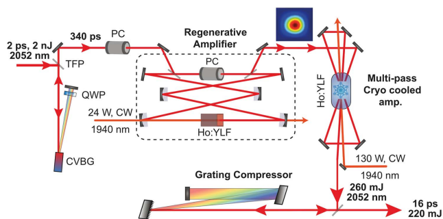
Fig. 1. Layout of the 2052 nm Ho:YLF solid-state laser system. The narrowband 2052 nm pulses from the three-color fiber front-end are stretched in a CVBG, and the repetition rate is reduced in a PC before amplification in a water-cooled regenerative amplifier and cryogenic cooled booster amplifier consecutively. Finally, the stretched pulses are back compressed using a pair of dielectric-coated gratings.
