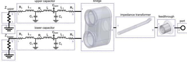
FIGURE 2: Half Antenna schematic.
