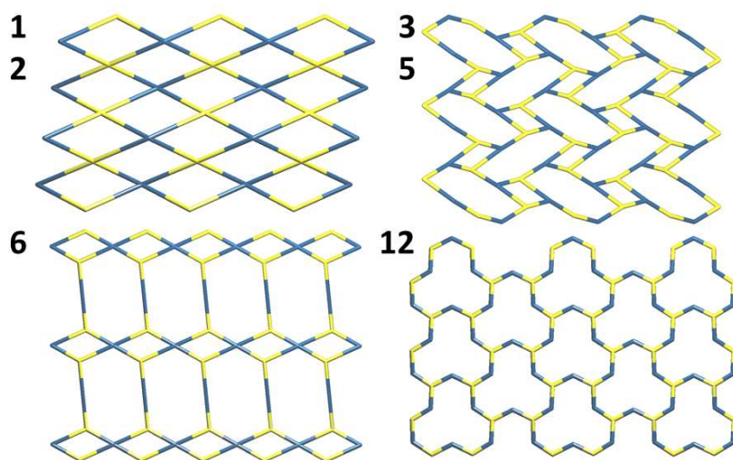
Figure 2. Nodal representation of the diperiodic networks in complexes 1 , 2 , 3 , 5 , 6 and 12 (uranium, yellow; dicarboxylate ligand, blue).
