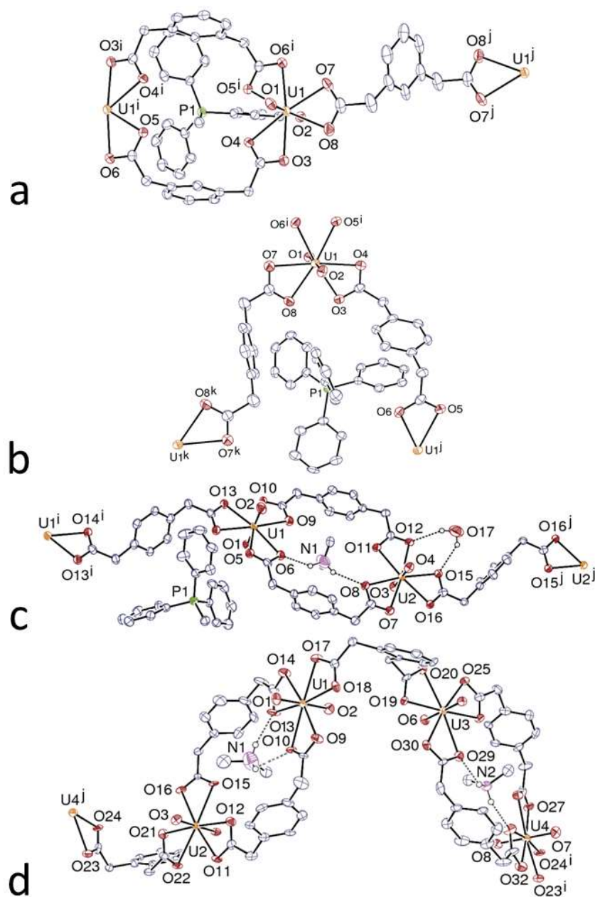
Figure 8. Views of compounds 13 (a), 14 (b), 15 (c), and 16 (d) with phosphonium cation in 16 and carbon-bound hydrogen atoms omitted. Hydrogen bonds are shown as dashed lines. Only one position of the disordered aromatic ring in 13 is shown. Symmetry codes: 13 i = 1 - x, 1 - y, 1 - z; j = -x, 2 - y, -z ; 14 i = x + 1, y, z; j = x - 1, y, z; k = 1 - x, 1 - y, 1 - z ; 15 i = -x, -y, 2 - z; j = 3 - x, 2 - y, 1 - z ; 16 i = x, y, z + 1; j = x, y, z - 1 .
