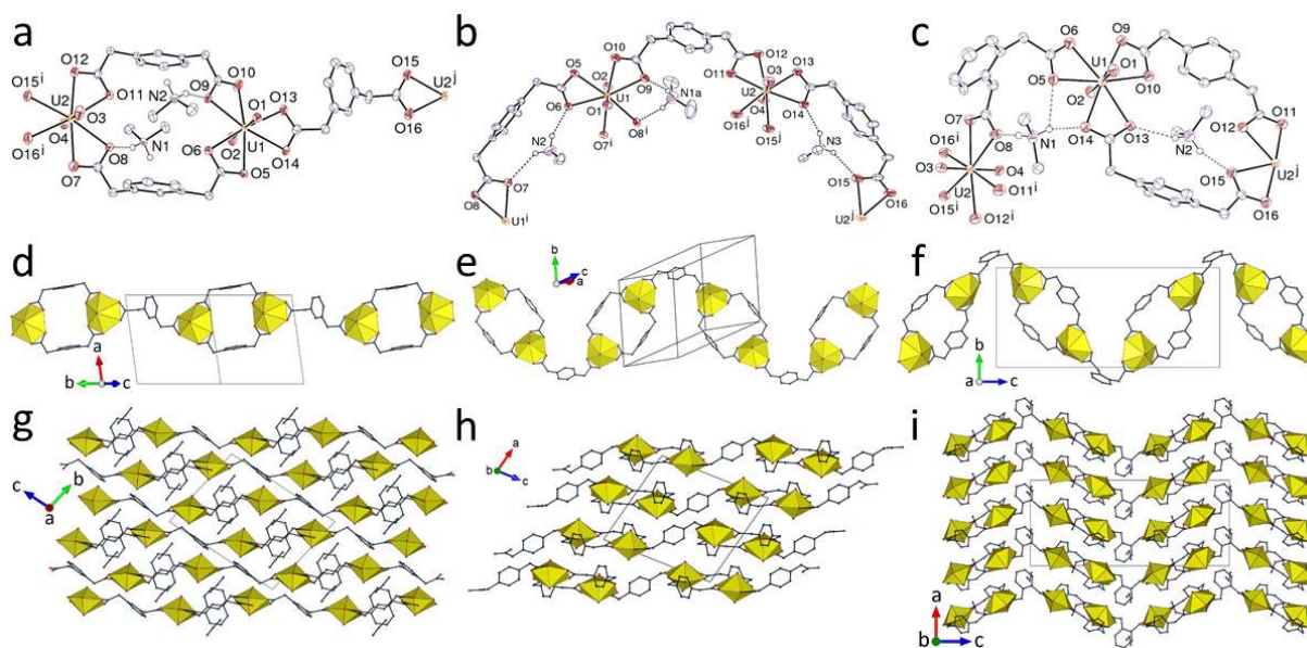
Figure 6. Views of compounds 9 (a), 10 (b), and 11 (c), with carbon-bound hydrogen atoms omitted and hydrogen bonds shown as dashed lines. Symmetry codes: 9 i = x, y + 1, z - 1 ; j = x, y - 1, z + 1 ; 10 i = 1 - x, -y, 2 - z ; j = -x, 1 - y, -z ; 11 i = 2 - x, -y, z - 1/2 ; j = 2 - x, -y, z + 1/2 . View of the 1D polymers in 9 (d), 10 (e), and 11 (f). Packing with the chains viewed side-on in 9 (g), 10 (h), and 11 (i).
