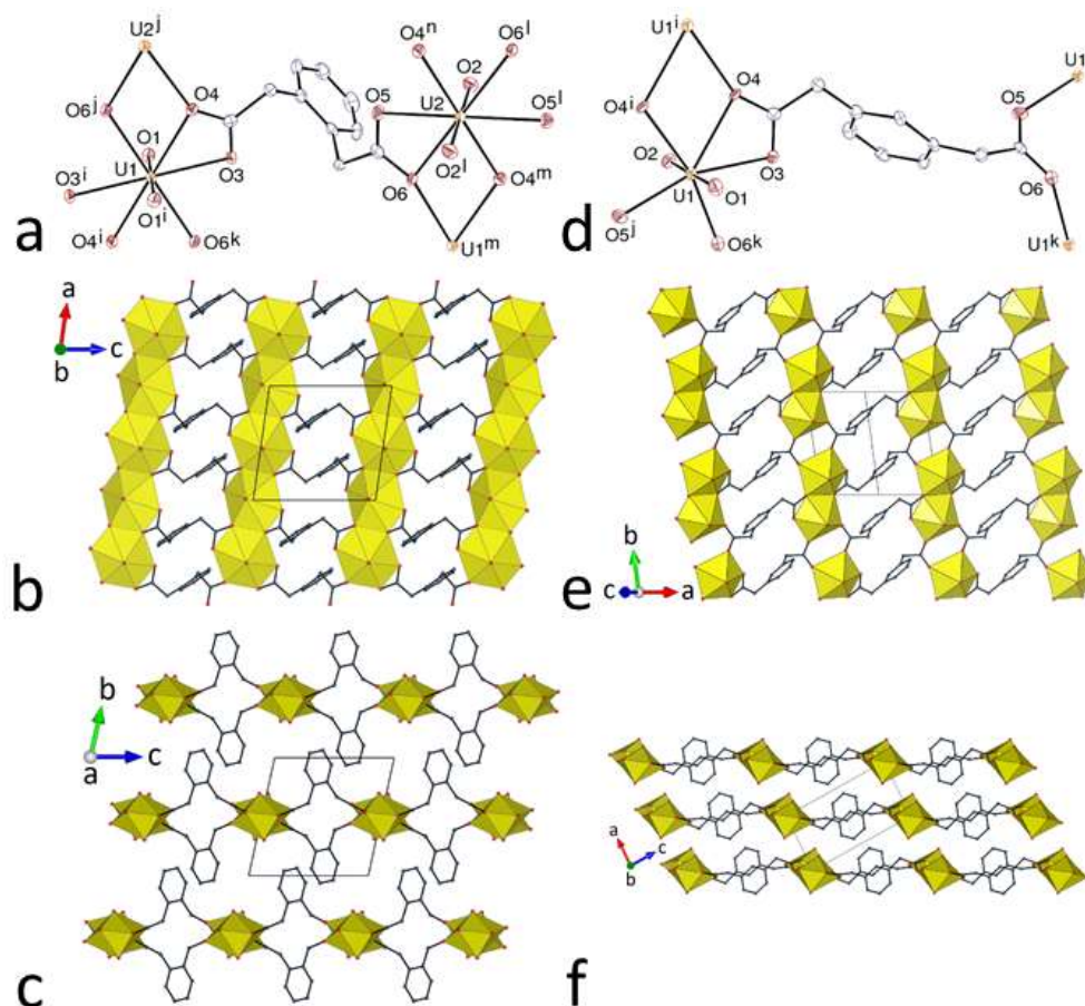
Figure 1. (a) View of compound 1 with solvent molecule and hydrogen atoms omitted. Symmetry codes: i = 1 - x, 1 - y, 2 - z ; j = x, y, z + 1 ; k = 1 - x, 1 - y, 1 - z ; l = 2 - x, 1 - y, -z ; m = x, y, z - 1 ; n = 2 - x, 1 - y, 1 - z . (b) View of the 2D network in 1 showing uranium coordination polyhedra. (c) Packing in 1 with layers viewed edge-on. (d) View of compound 2 with hydrogen atoms omitted. Symmetry codes: i = -x, -y, 2 - z ; j = x - 1, y, z + 1 ; k = 1 - x, 1 - y, 1 - z ; l = x + 1, y, z - 1 . (e) View of the 2D network in 2 . (f) Packing in 2 with layers viewed edge-on.
