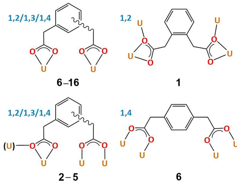
Scheme 1 Coordination modes of the three isomers of \text{pda}^{2-} in complexes 1–16 . The U in parenthesis corresponds to the additional bonding in complex 2 .
