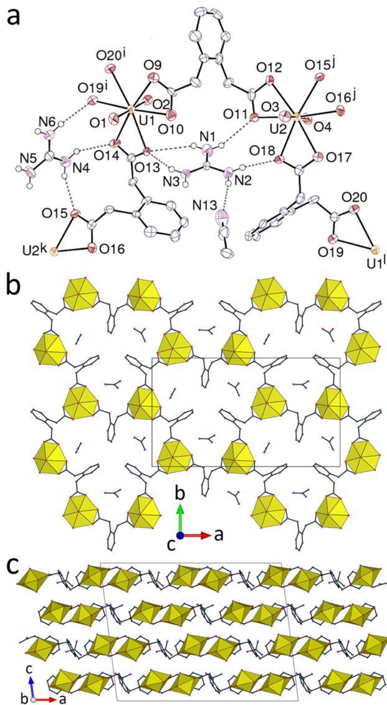
Figure 7. (a) View of one of the two independent units in compound 12 with carbon-bound hydrogen atoms omitted and hydrogen bonds shown as dashed lines. Symmetry codes: i = x - 1/2, y + 1/2, z ; j = x + 1/2, y + 1/2, z ; k = x - 1/2, y - 1/2, z ; l = x + 1/2, y - 1/2, z ; m = x, y + 1, z . (b) View of the 2D assembly. (c) Packing with layers viewed edge-on.
