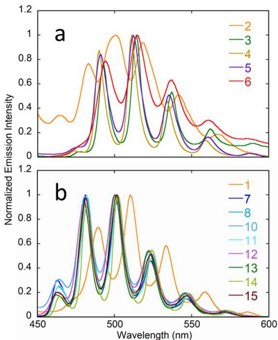
Figure 10. Normalized emission spectra for the complexes with O_5 (a) or O_6 (b) equatorial environments, recorded in the solid state at room temperature under excitation at a wavelength of 420 nm.
