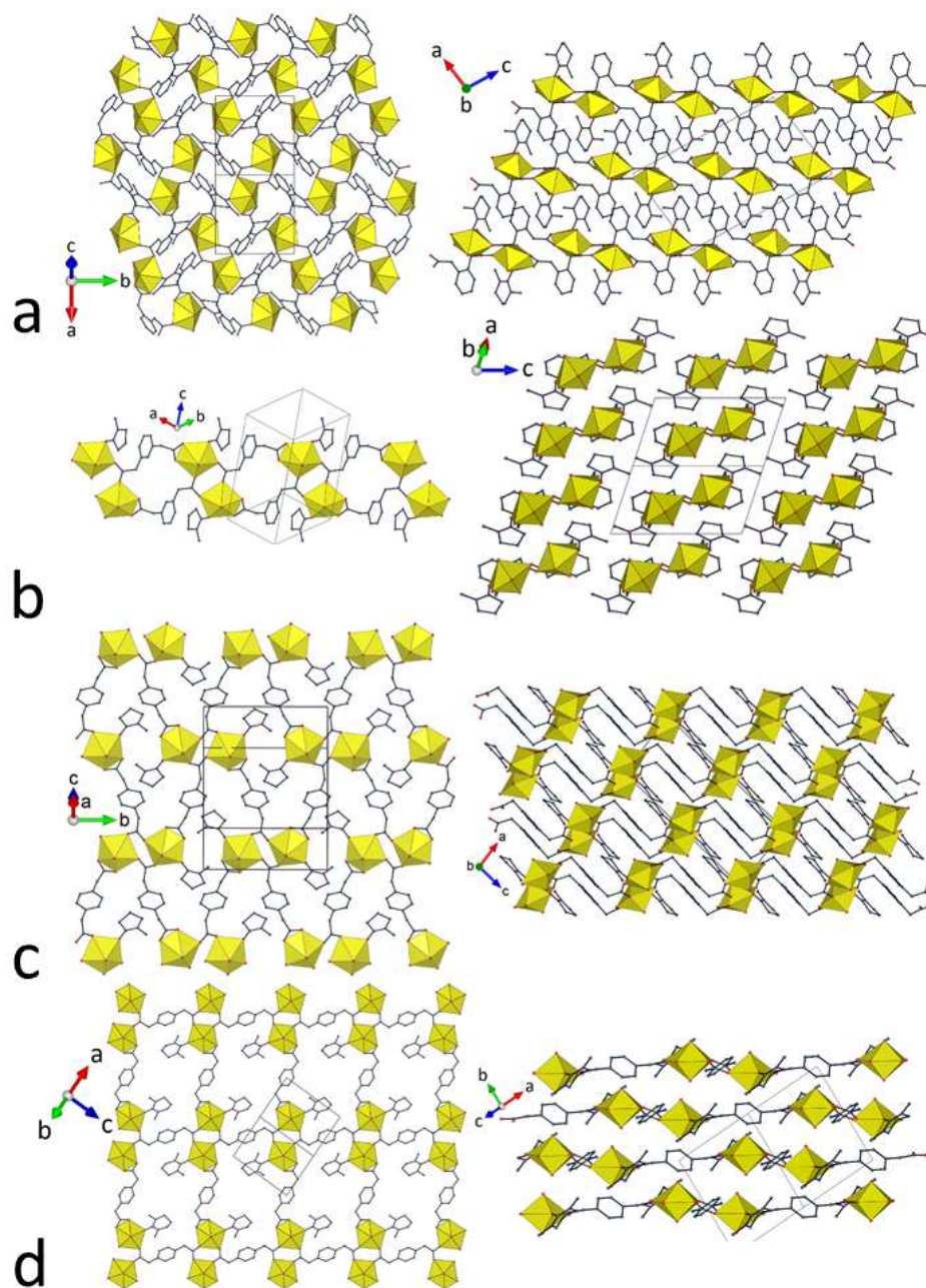
Figure 4. (a) View of the 2D assembly (left) and the packing with layers edge-on (right) in compound 3 . (b) View of the 1D polymer (left) and the packing with chains end-on (right) in compound 4 . (c) View of the 2D assembly (left) and the packing with layers edge-on (right) in compound 5 . (d) View of the 2D assembly (left) and the packing with layers edge-on (right) in compound 6 .
