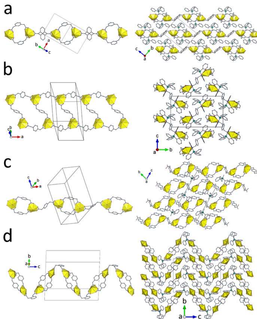
Figure 9. Views of the 1D polymer (left) and the packing (right) in compounds 13 (a), 14 (b), 15 (c), and 16 (d).
