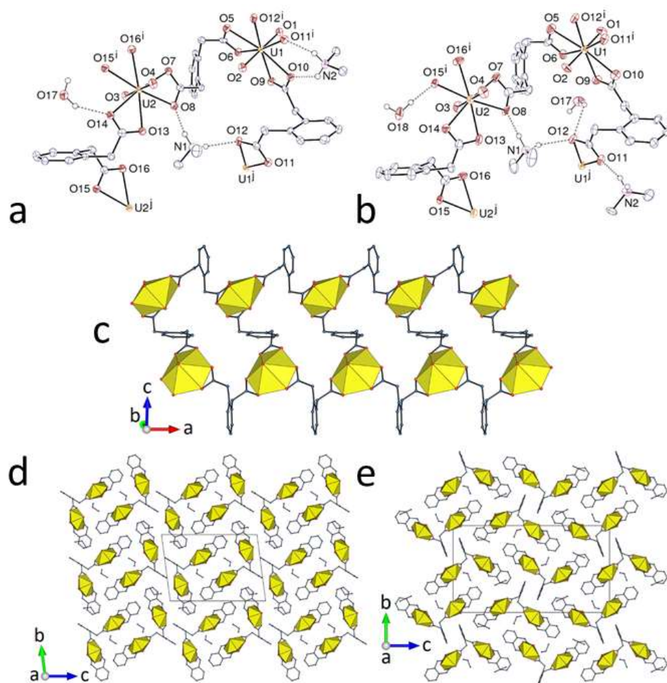
Figure 5. Views of compounds 7 (a) and 8 (b), with carbon-bound hydrogen atoms omitted and hydrogen bonds shown as dashed lines. Symmetry codes: i = x + 1, y, z ; j = x - 1, y, z for both. View of the 1D polymer in 8 (c). Packing in 7 (d) and 8 (e), with chains viewed end-on.
