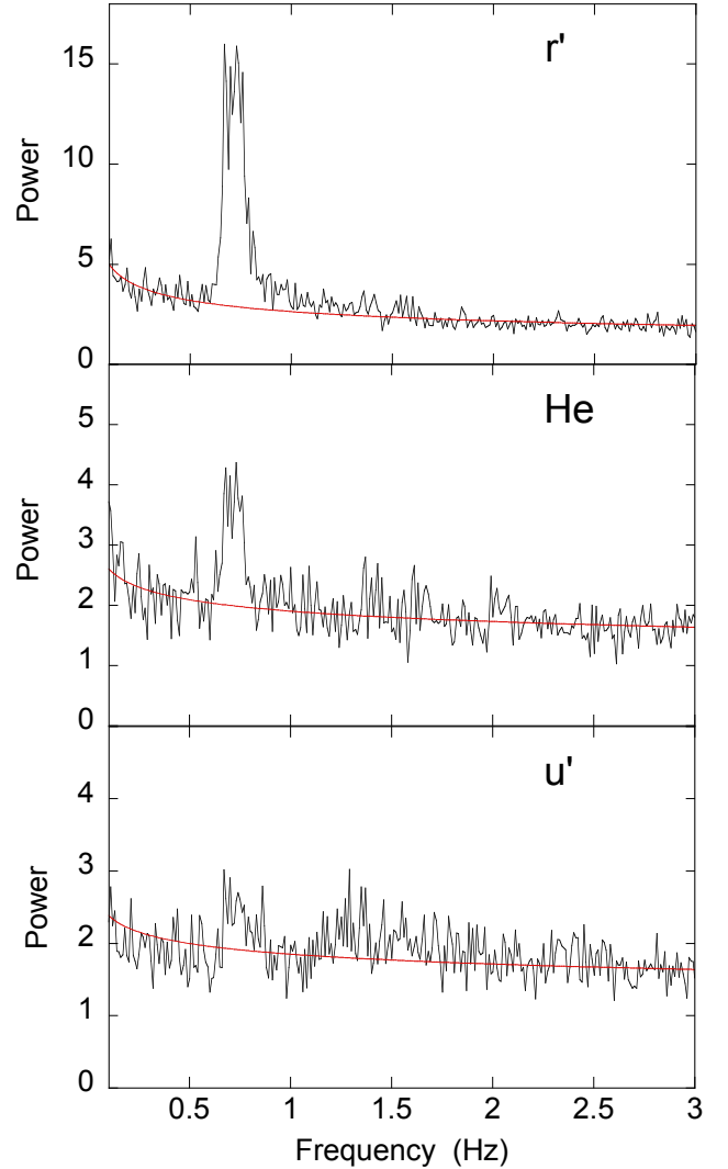
Fig. 3. Bright phase QPO frequency profiles. Mean power density spectra are shown in the range of 0.1–3 Hz for the bright phase interval 0.75–1.15, excluding B4, in the three wavelength bands ( top : r' , middle : He, bottom : u' ). The Y-scale is the power computed with Leahy normalisation. The red line shows the subtracted background fitted as a power-law outside the 0.5–1 Hz interval.
