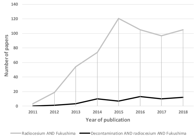
Figure 1. Evolution of the number of studies published on radiocesium and Fukushima (including or not including a reference to decontamination) in the literature between 2011 and 2018, according to the Scopus search engine.
