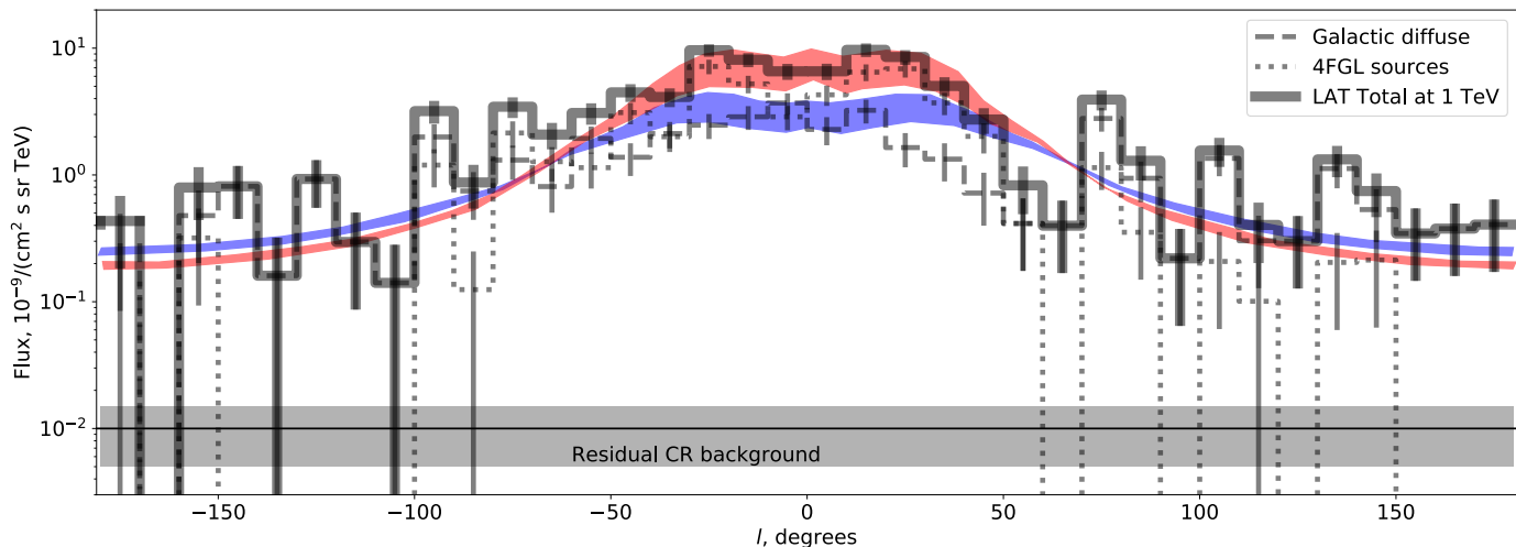
Fig. 2. Galactic longitude profile of the signal from Galactic latitude range |b| < 2^\circ . Dashed and dotted lines show the diffuse and resolved 4FGL source flux components. Solid line is the sum of the two components. Blue and red model curves are from Cataldo et al. (2019). Grey band shows the level of residual cosmic ray background.
