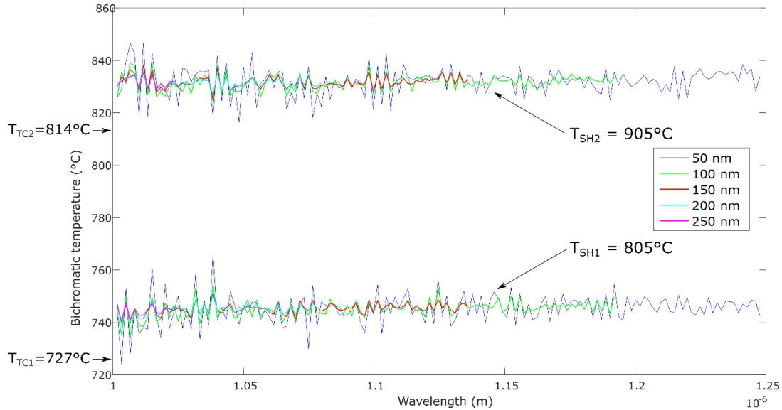
Figure 6: Scanned bichromatic temperature as function of the wavelength \lambda_1 , with calculation made for several gaps (from 50 to 250nm) and both \lambda_1 and \lambda_2 included in the wavelength range: 1-1.3 \mu\text{m} , for two sample heater temperatures ( T_{\text{SH}} ): 805°C and 905°C, with an emissivity ratio hypothesis \varepsilon_2/\varepsilon_1 = 1
