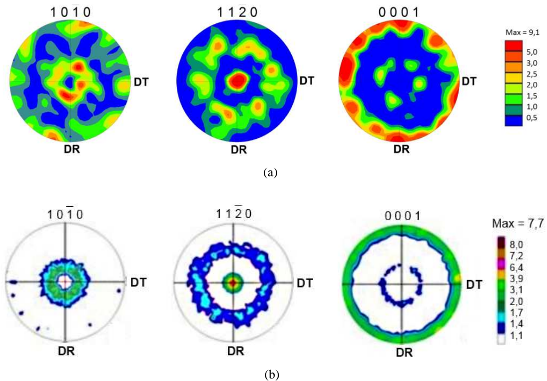
FIG. 4—Pole figures \{10.0\} , \{11.0\} and \{00.1\} recalculated for a model \alpha_{\text{Zr}}(\text{O}) sample containing 2 wt.% of oxygen in average: (a) surface analysis by EBSD, (b) volume analysis by neutron diffraction; DR: radial direction; DT: circumferential direction.
