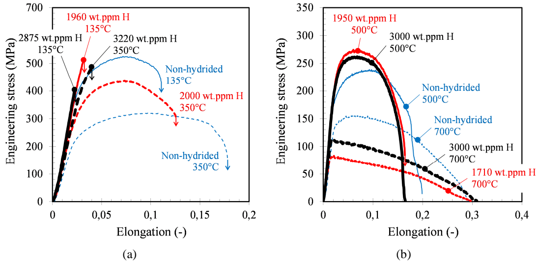
FIG. 15—Examples of engineering stress-strain (deduced from cross-head displacement) curves obtained (a) at 135 and 350°C and (b) at 500 and 700°C for model (prior-) \beta_{Zr} materials, non-hydrated or containing between 1710 and 3220 wt.ppm of hydrogen (and at least 0.2 wt.% of oxygen).
