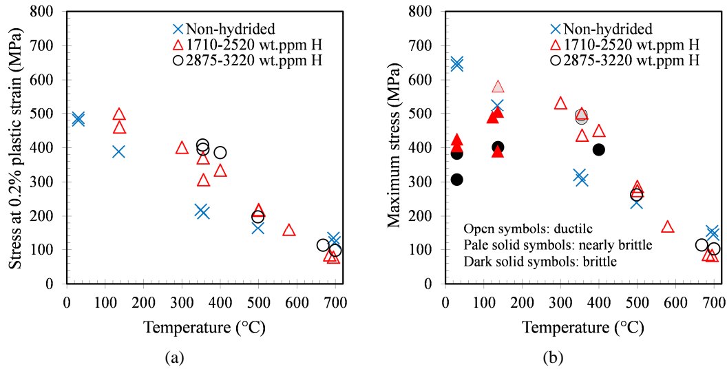
FIG. 17—Evolution as a function of temperature of (a) the yield stress at 0.2% plastic strain and (b) the ultimate (maximum) stress obtained for model (prior-) \beta_{Zr} materials, non-hydrided or containing between 1710 and 3220 wt.ppm of hydrogen (and at least 0.2 wt.% of oxygen).
