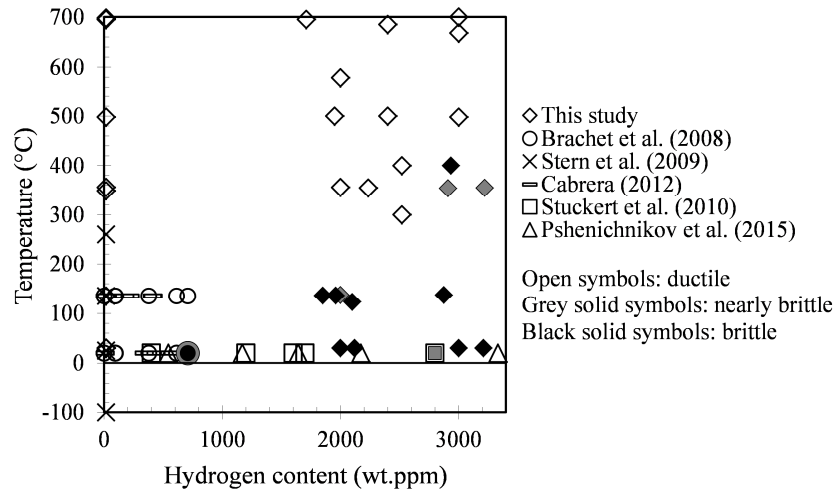
FIG. 18—Ductile or brittle fracture modes of the (prior-) \beta_{Zr} phase as a function of temperature and mean hydrogen content; data from this study and from Brachet et al. [3], Stern et al. [14], Cabrera [63], Stuckert et al. [62] and Pshenichnikov et al. [38] (features given in Table 3).
