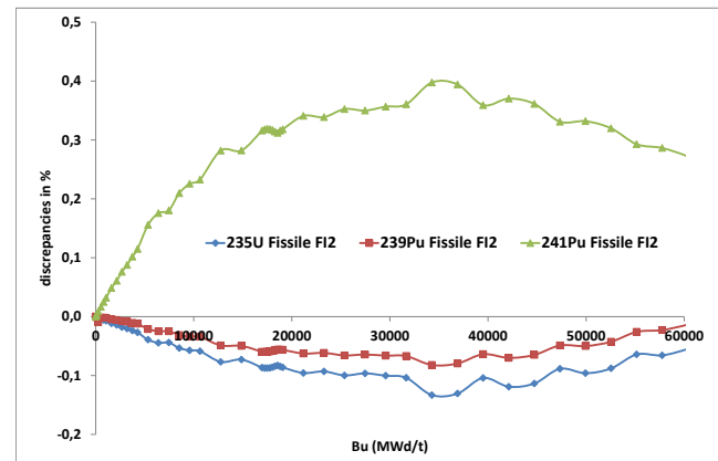
Fig. 13. Relative discrepancies on averaged concentrations in the FI2 assembly between APOLLO2 and CRONOS2 8 group
