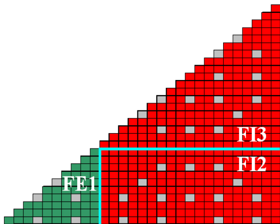
Fig. 4. Cluster of assemblies used to generate collapsed cross sections for CRONOS2
