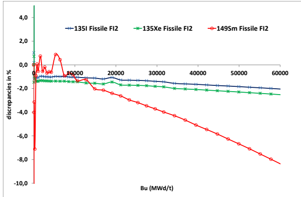
Fig. 15. Relative discrepancies on averaged concentrations for some fission products between APOLLO2 and CRONOS2 8 group [FI2 assembly]
