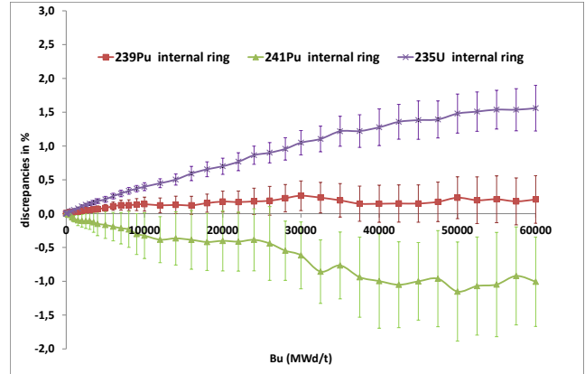
Fig. 9. Relative discrepancies on the concentrations between APOLLO2 and TRIPOLI-4® [cell named FISSILE 1 - internal ring]
