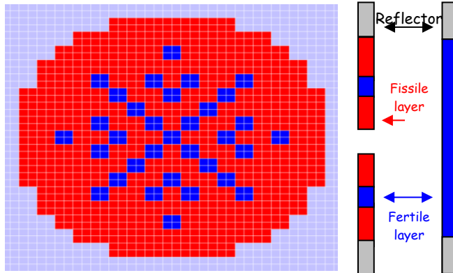
Fig. 2. Geometric description of the HCPWR 19x19 core
