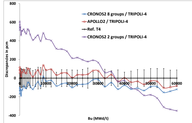
Fig. 7. Evolution of the discrepancies on K infinity and standards deviation
