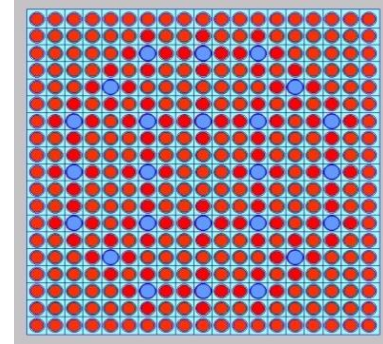
Fig. 1. Geometric description of the HCPWR 19x19 FA
