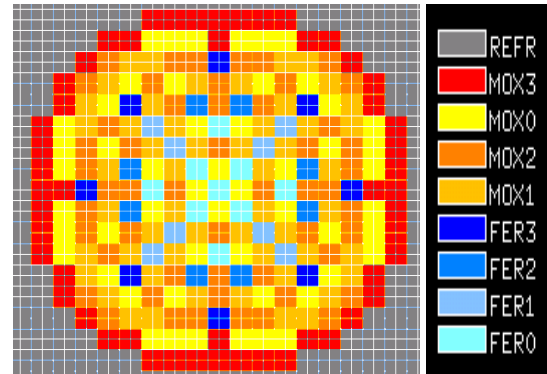
Fig. 3. Loading pattern of the HCPWR 19x19 core
