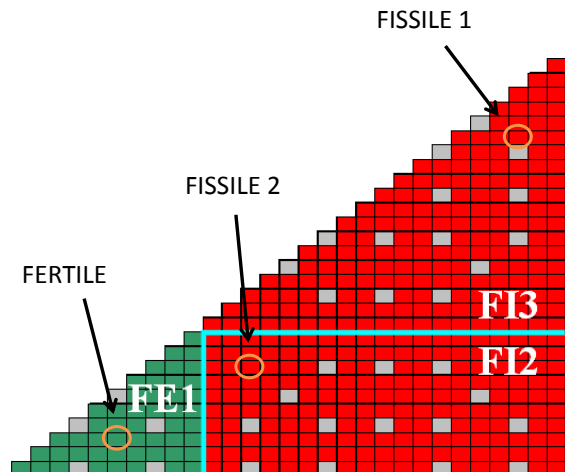
Fig. 8. Positions of the studied cells in the cluster of assembly
