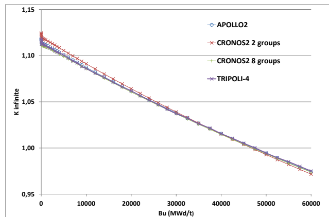
Fig. 6. Evolution of K infinity during depletion
