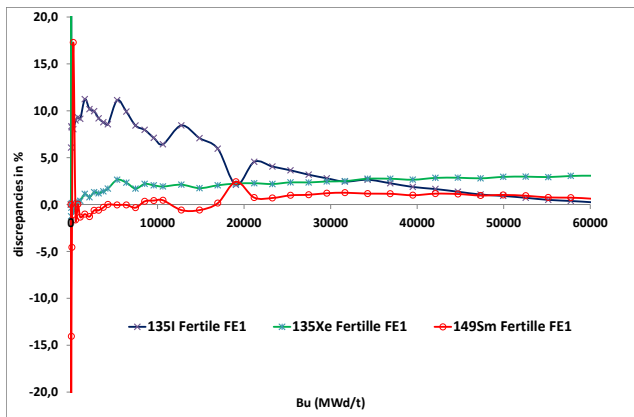
Fig. 16. Relative discrepancies on averaged concentrations for some fission products between APOLLO2 and CRONOS2 8 group [FE1 assembly]
