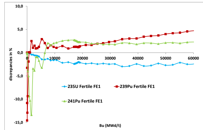
Fig. 14. Relative discrepancies on averaged concentrations in the FE1 assembly between APOLLO2 and CRONOS2 8 group
