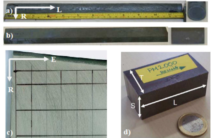
Figure 1: ODS materials available for investigations; a) hot extruded S1 rod, b) hipped S2 slab, c) hot rolled S3 plate, d) hot rolled S4 block
