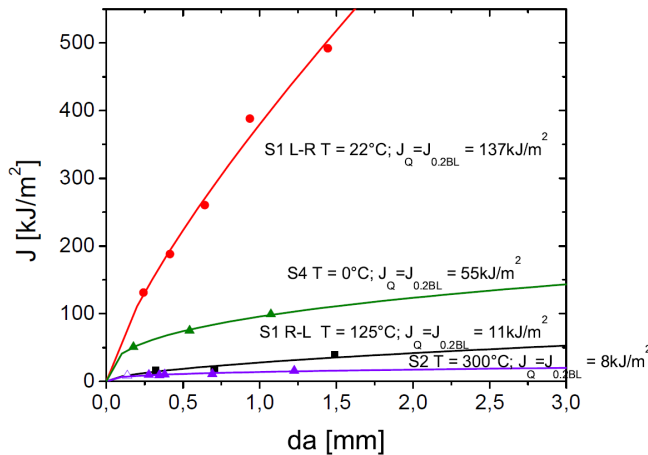
Figure 7: Fracture toughness J and J_Q = J_{0.2BL} data in the upper shelf regime of S1, S2, S4 ODS-materials
