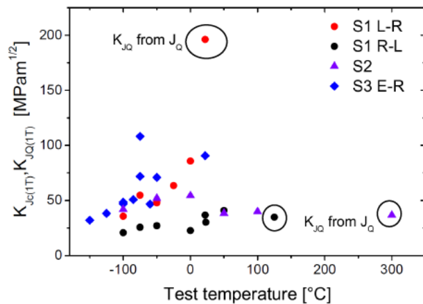
Figure 4: Fracture toughness K_{Jc(T)} , K_{JQ(T)} data in the transition region of S1, S2, S3 ODS-materials
