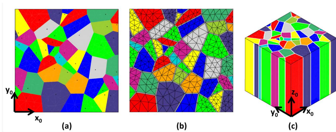
FIG. 4 - Example of creation of a numerical microstructure with 50 grains : a) Voronoï diagram of 0.5 \times 0.5 \mu\text{m}^2 square, b) mesh of the grains and the grain boundaries and c) final microstructure obtained by extrusion with Z_0 axis parallel to the diffusion direction.
