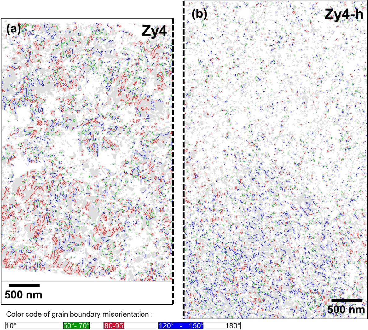
Fig. 17 - Colored maps of oxide grain boundaries on a) Zy4 and b) Zy4-h samples, function of the misorientation angle range. Only half maps of the scanned areas are shown, a) the left part of Zy4 sample and b) the right part of the Zy4-h sample.
