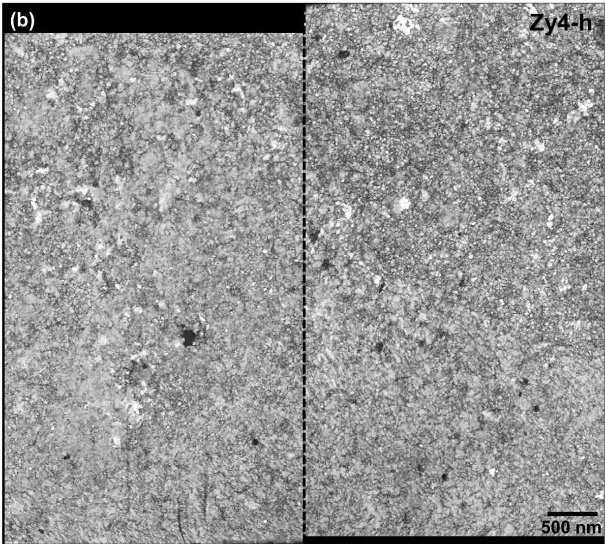
Fig. 5 - Correlation index maps of oxide planes grown on a) Zy4 and b) Zy4-h samples, 1 \mu\text{m} above the oxide/metal interface, which is delimited on TEM images (Fig 3) with a dashed rectangular.
