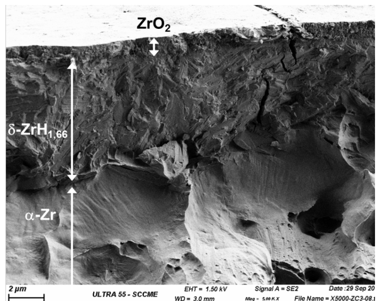
FIG. 1 – SEM fractography of the Zy4-h surface after cathodic charging and corrosion during 14 days in simulated PWR conditions.
