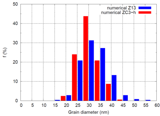
Fig. 8 - Grain size distributions for Zy4 and Zy4-h numerical microstructures.
