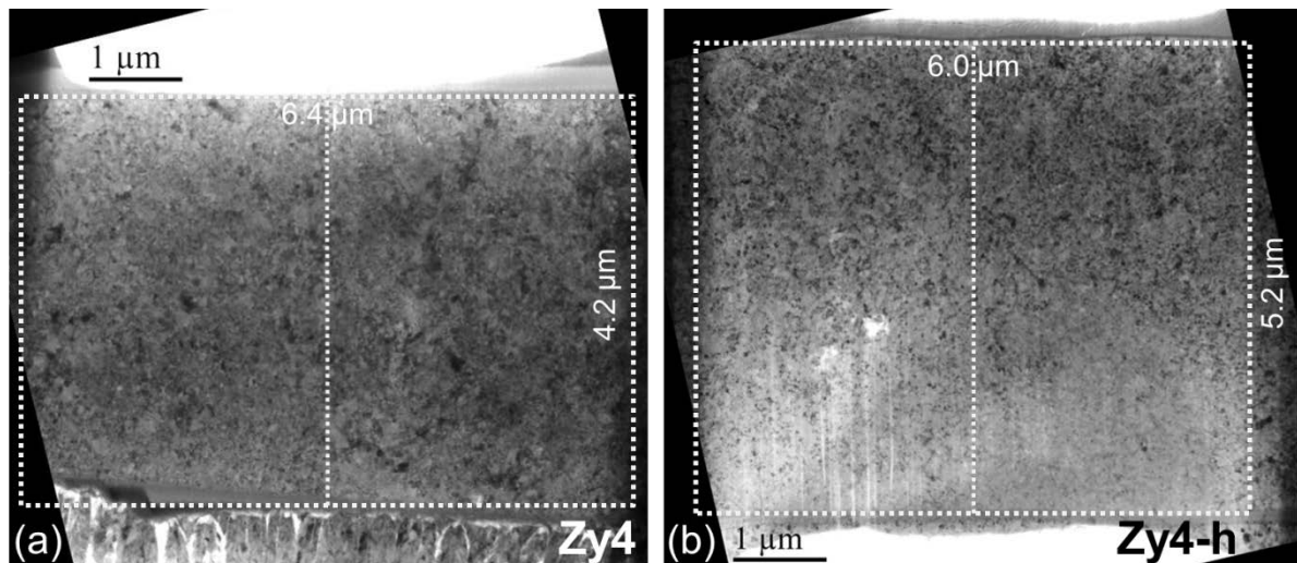
FIG. 3 - Bright-field TEM images of the FIB thin areas taken about 1 μm away from the oxide/metal interface, in the oxide layer formed on a) Zy4 and b) Zy4-h. The scanned regions with TEM are delineated with white dots.
