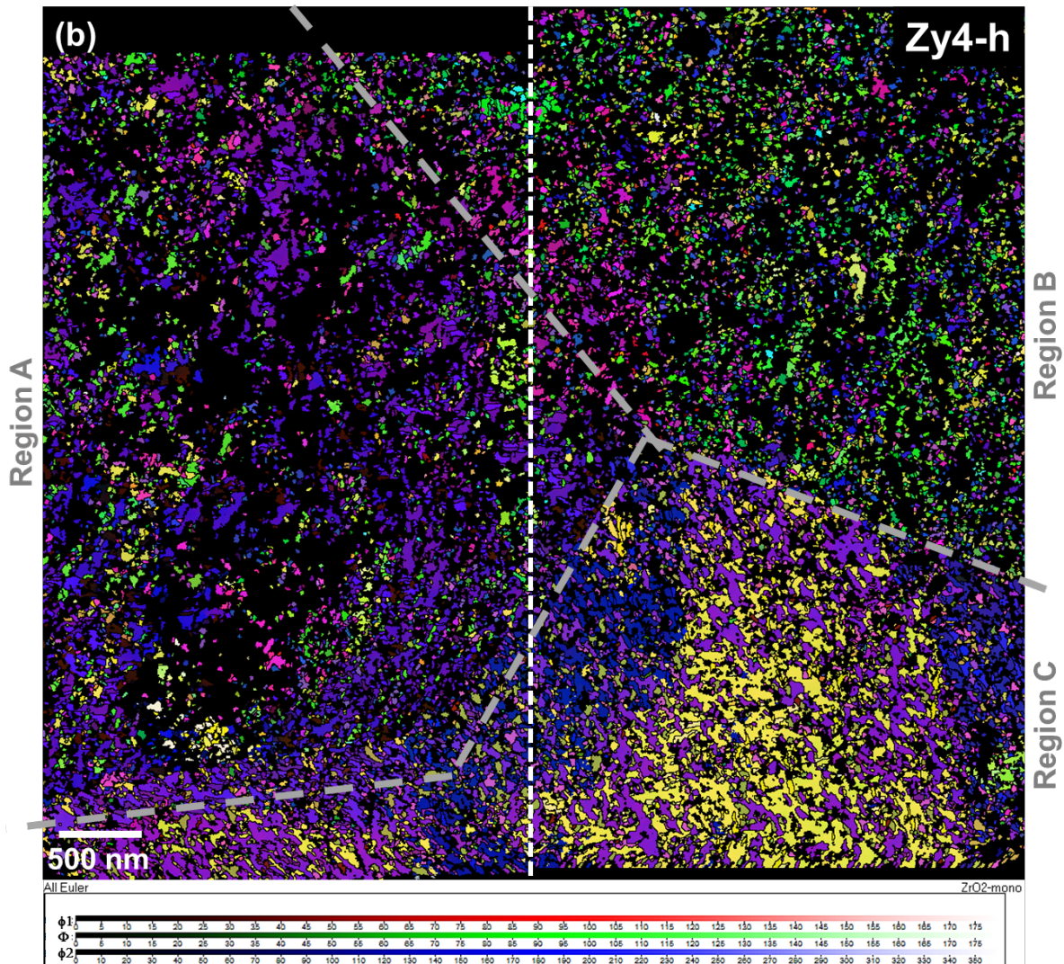
Fig. 12 - Orientation map of the transverse section plane of oxide grains grown on Zy4-h sample, 1 \mu\text{m} above the oxide/metal interface, which is delimited on Fig 3b) with a dashed rectangular. Monoclinic phase orientations are colored as a function of the corresponding Euler angles ( \phi_1 , \Phi , \phi_2 ).
