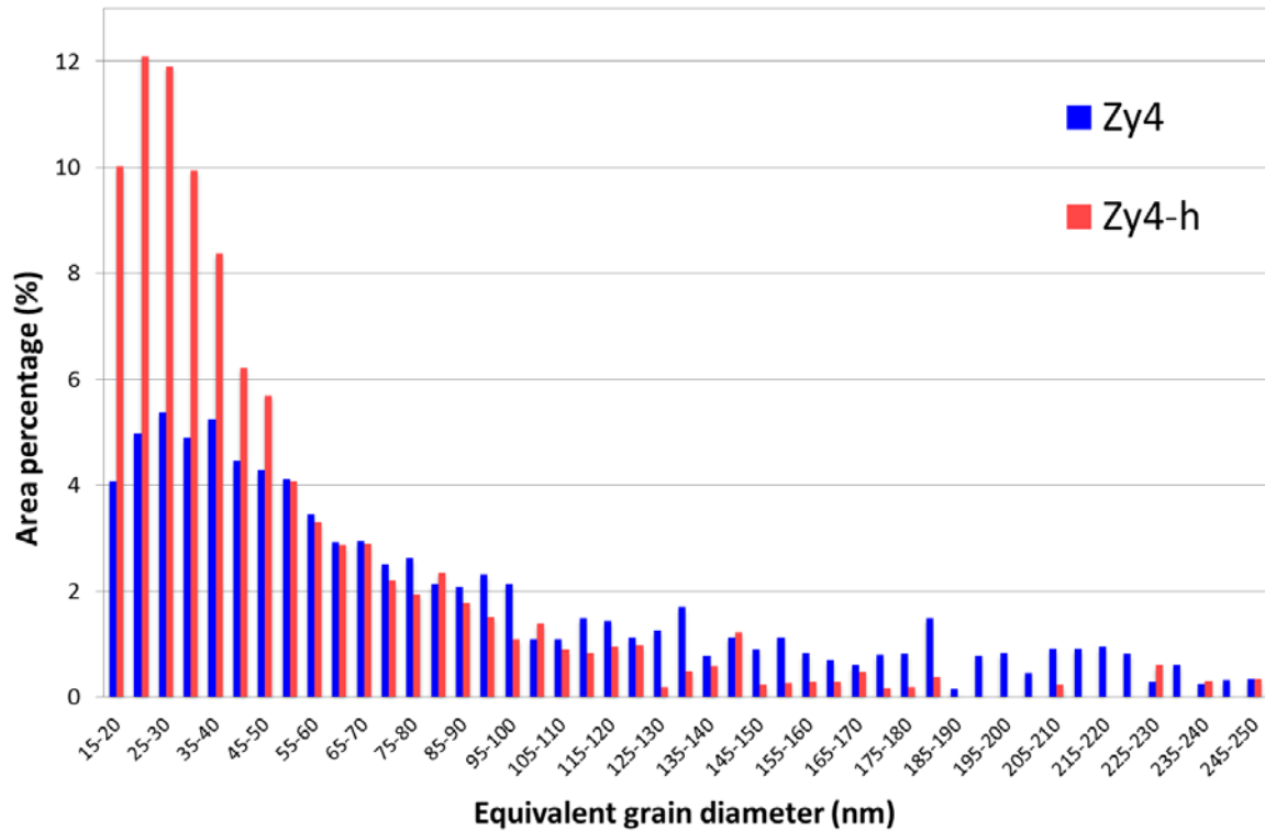
Fig. 6 – Grain size distribution of columnar grain width grown on Zy4 and Zy4-h, in area percentage.
