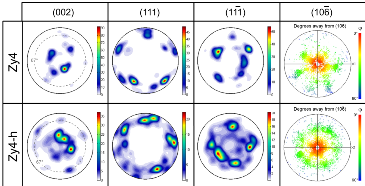
Fig. 13 – Pole Figures of the monoclinic oxide grains located 1 \mu\text{m} away the oxide/metal interface. The (111) , (11\bar{1}) and (002) poles are shown in color intensity levels. The (10\bar{6}) pole figure shows the pole position of all indexed points with the ACOM-TEM method, the color legend correspond to the angular deviation with (10\bar{6}) , referred Fig. 14,15 and 16.
