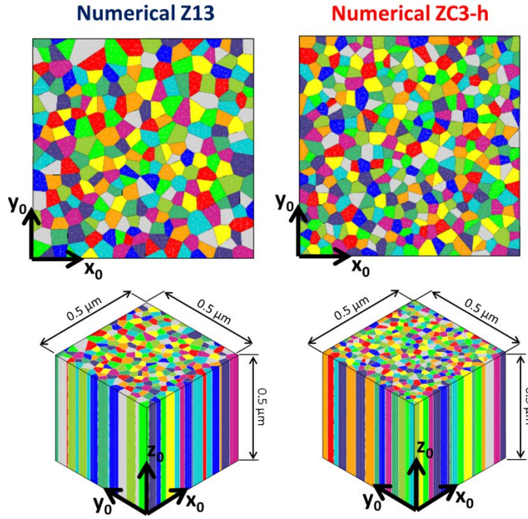
Fig. 7 - Numerical samples of Zy4 (250 grains) and Zy4-h (380 grains).
