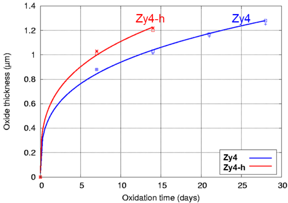
FIG. 2 - Corrosion kinetics curves of reference (Zy4) and pre-hydrated (Zy4-h) Zircaloy-4 samples corroded in static autoclave with light primary water at 360°C and 18.7 MPa. The water chemistry was composed of 1000 wt.ppm of boron and 2 wt.ppm of lithium.
