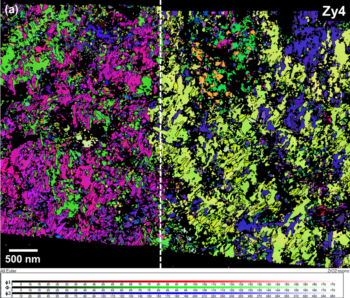
Fig. 11 - Orientation map of the transverse section plane of oxide grains grown on Zy4 sample, 1 \mu\text{m} above the oxide/metal interface, which is delimited on Fig 3a) with a dashed rectangular. Monoclinic phase orientations are colored as a function of the corresponding Euler angles ( \phi_1 , \Phi , \phi_2 ).
