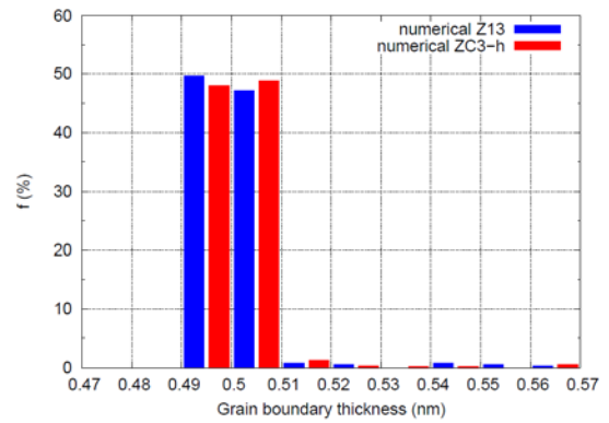
Fig. 9 - Grain boundary thickness distributions for Zy4 and Zy4-h numerical microstructures.
