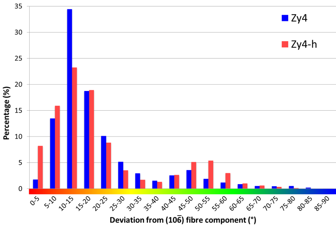
Fig. 15 - Intensity profile of (10\bar{6}) pole figure (Fig. 13) function of the polar angle for both Zy4 and Zy4-h samples.
