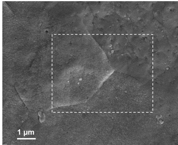
Fig. 18 – SEM Image of the Zy4-h sample surface before FIB milling. The dashed rectangular delineates the surface of the oxide layer thinned and scanned 0.3 μm deeper.
