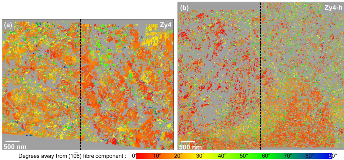
Fig. 14 - Orientation maps of the monoclinic ZrO_2 grains colored function of the angle deviation from (10\bar{6}) fibre component of oxide foils a) Zy4 and b) Zy4-h.
