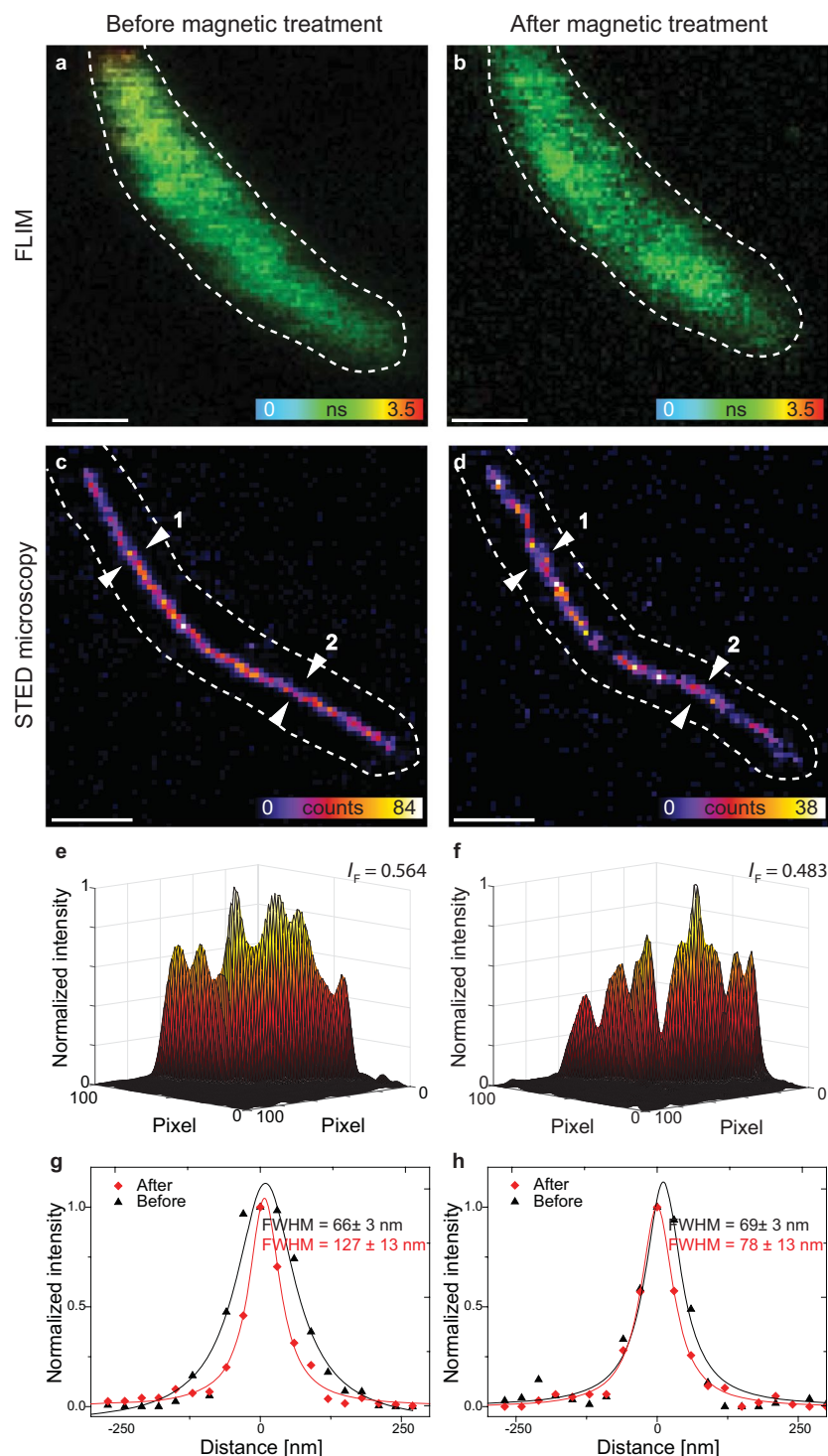
Figure 4. The in vivo FLIM-FRET and STED experiments on MSR-1 cells before and after application of a magnetic torque. FLIM images (a,b) and STED images (c,d) of MSR-1 cells with MamJ-phiYFP and TagRFP657-MamK before (a,c) and after (b,d) applying treatment (10 times rotation of two magnets up to 270°). (e,f) Corresponding 3D surface intensity plots of the STED images. We normalized the intensity and used a Gaussian filter. Normalized fluorescence intensities along the filament structures were calculated to I_F = 0.564 and I_F = 0.483 , respectively (SI). (g,h) Intensity line profiles. Lorentzian approximation provides a full-width at half maximum (FWHM) at position 1 before magnetic treatment of 66 \pm 3 nm and after magnetic treatment of 127 \pm 13 nm. At position 2, the apparent filament diameter is 69 \pm 3 nm before and 78 \pm 13 nm afterwards. Intensity line profiles represent normalized raw image data and fitting curves (fitted value \pm standard error). Scale bar: 1 \mu m.
